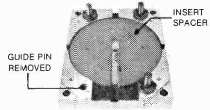
INSERT MOLD FRAME ASSEMBLY
