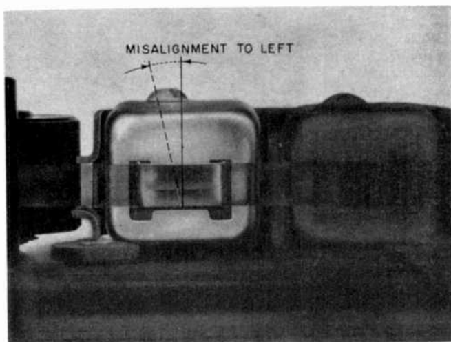
Figure 2: due to bumps or jars, head may become misaligned.
