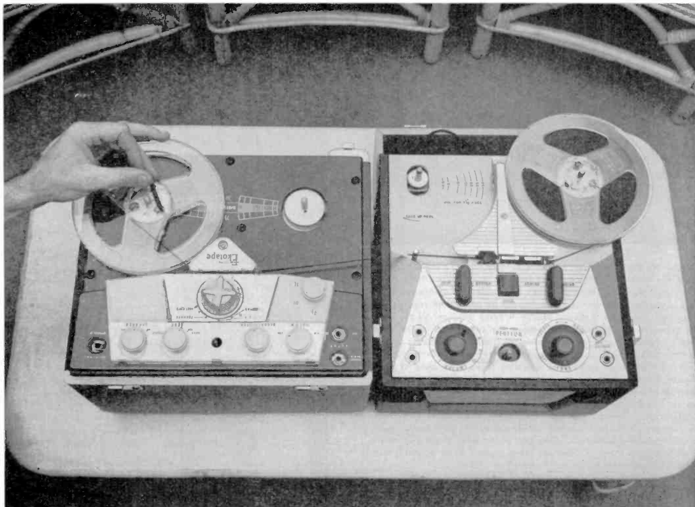
Above: picture shows how the reels are mounted on the recorders for binaural recording. The tape in this case travels from right to left and goes through the heads of both machines. Below: since the Ekotape is used to pull the tape through both machines, the pressure roller is removed from the Pentron by removing the screw that holds it in place. This allows the tape to pass freely over the Pentron capstan. Once the machines are aligned, reference marks should be placed on them so that they may be realigned easily.
