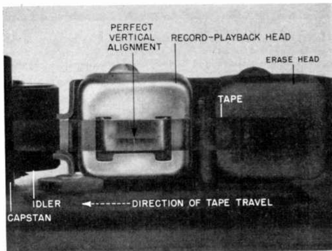
Figure 1: When your recorder left the factory its head was in perfect alignment and would playback or record with maximum fidelity.
