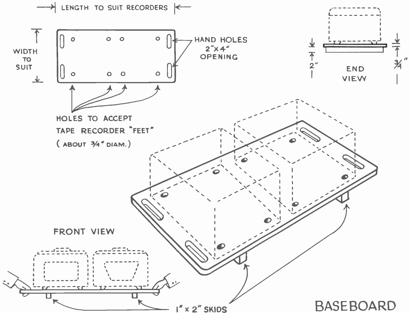
The sketch shows a type of baseboard that easily can be made from 3/4-inch plywood to insure exact placement of recorders relative to each other for recording and playback. It is absolutely essential that recorders always be placed in exactly the same relative positions.
