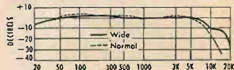
Response: wide and normal IF positions.
