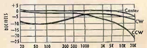
Tone control curves.
