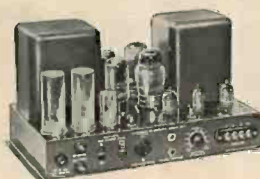
Straightforward layout of 260A.
