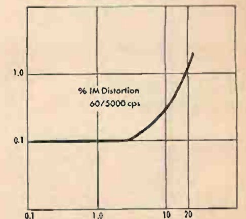
Intermodulation distortion.
