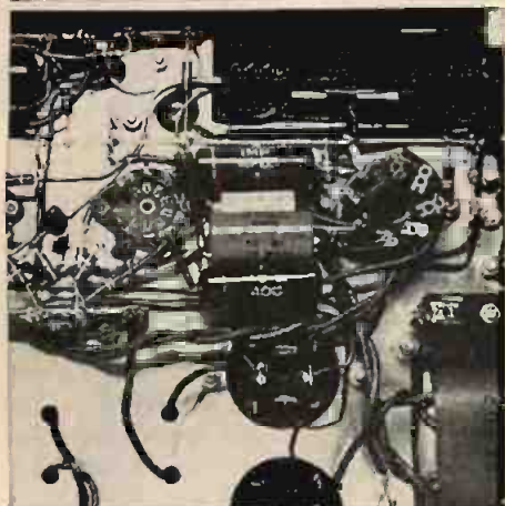
Drawing versus real life. To make the drawing clearer, parts are compressed. In actual practice, the 400-volt capacitor comes almost on top of socket marked J.
