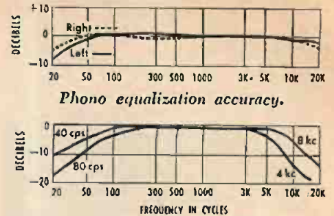
Rumble and scratch filter characteristics?
