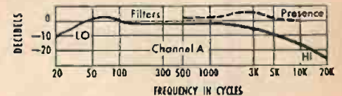
Effect of filter controls.
