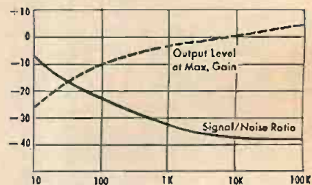
Output level and signal-to-noise ratio.
