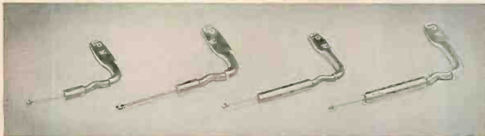
From left to right, a Clevite "Walco" W-75 with a short wire shank; the W-77 with a longer shank made of tubing; the W-103 for stereo, with shank-length midway between the other two; the W-107 stereo model, identical with the W-103 except that the twin tips are not diametrically opposite each other.
