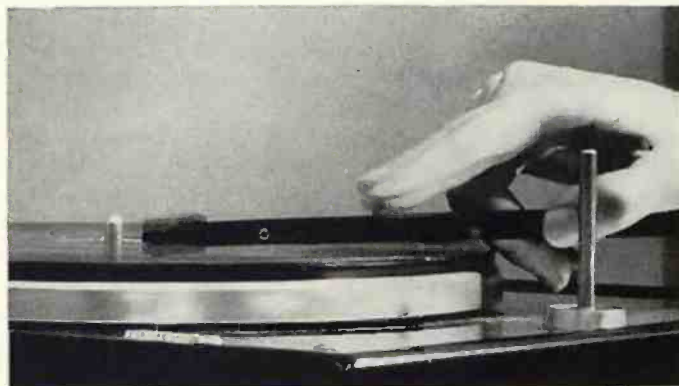
The Shure Studio Dynetic Cartridge is an integral part of the tone arm. Separate cartridges are available under the name "Professional Dynetic." The phantom view shows how the cartridge is elevated clear of the record. (Shure Bros., Inc., 222 Hartley Ave., Evanston, Ill.)
