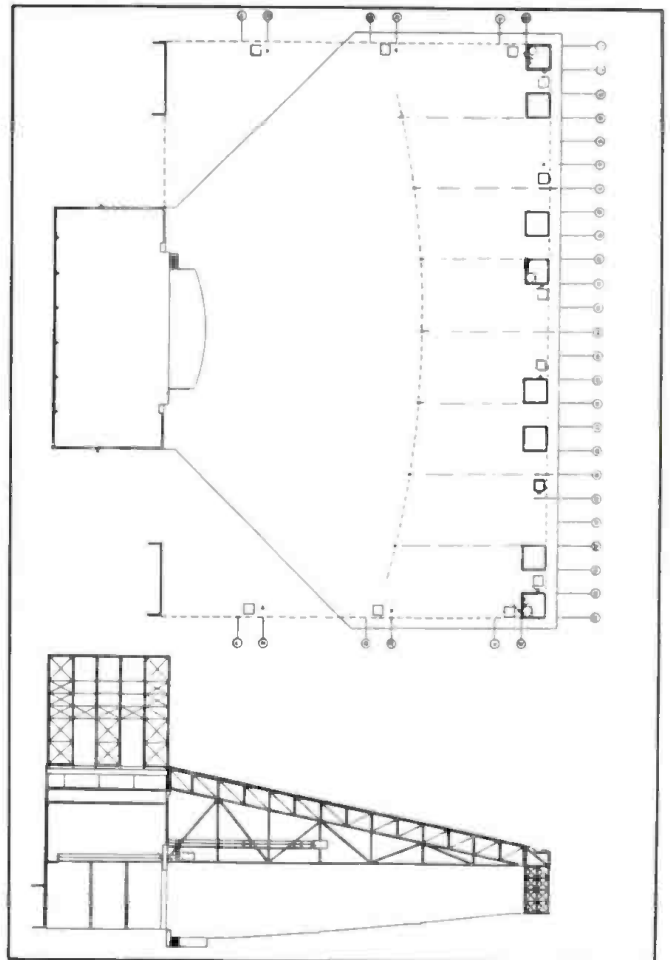
Figure 3. Plan and section of Riverbend.
