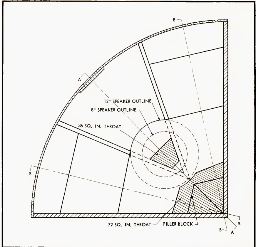
Fig. 4. Section through the phase-inversion chamber showing placement of the speaker unit, as well as throats of both front and back horns.
