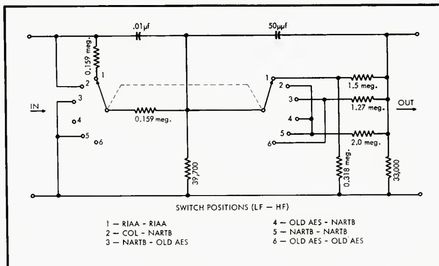
Fig. 6. Complete schematic of the recording characteristic simulator
