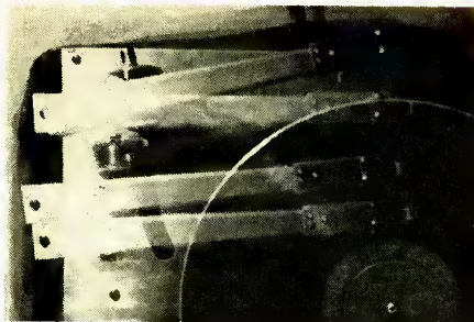
Fig. 3. Multiple exposure of device in operation showing pickup arm on the rest and in successive positions on the record. Note that the arm is tangent in all positions.
