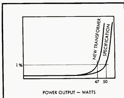
Fig. 5. Typical relationship between the published specification for distortion characteristic, and the measured figures, when the new output transformer has resulted in loss of efficiency, due to some cause that should be identified.
