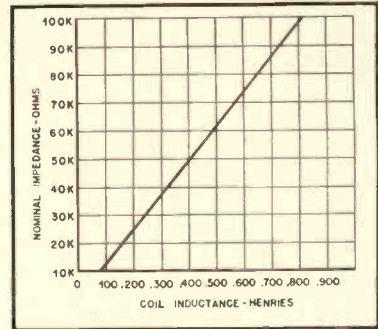
Fig. 4. Nominal impedance of a magnetic pickup as a function of coil inductance.
