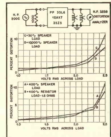
Fig. 7. Harmonic distortion vs. power output.
