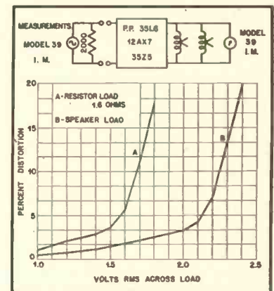
Fig. 6. Intermodulation distortion vs. power output.
