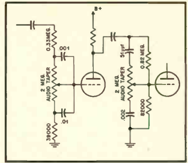
Fig. 6. Circuit values to approximate the curves of Fig. 5. As many of the values of the original \mathcal{R} circuit as possible have been retained.
