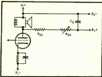
Fig. 4. D.c. bias on high-impedance speaker may be avoided by use of second B supply to buck out d.c. from main B supply.
