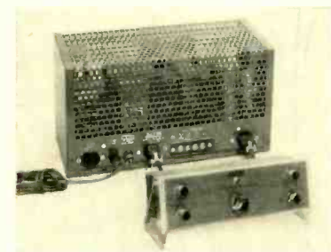
The amplifiers discussed by the author include, at left, the Altec Lansing A-333-A with the A-433-A preamplifier, and below from left to right, the Bell 2145A, the Brook 12A3, and the Leak "Point One."
