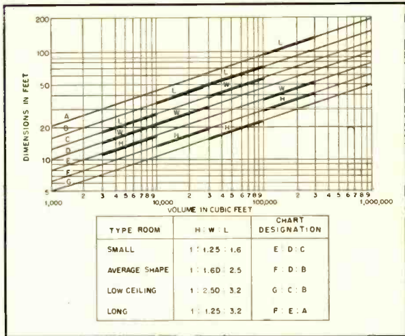
Fig. 7. Preferred studio dimensions and ratios of width and length. (Chart courtesy RCA).
