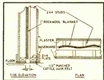
Fig. 3. Detail of staggered-stud wall.
