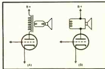
Fig. 2. Conventional single-ended output stage with low-impedance speaker (A) and with high-impedance speaker and no output transformer (B).
