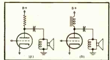
Fig. 3. Capacitance-coupled output stage may be shunt fed using resistor (A) or choke (B).
