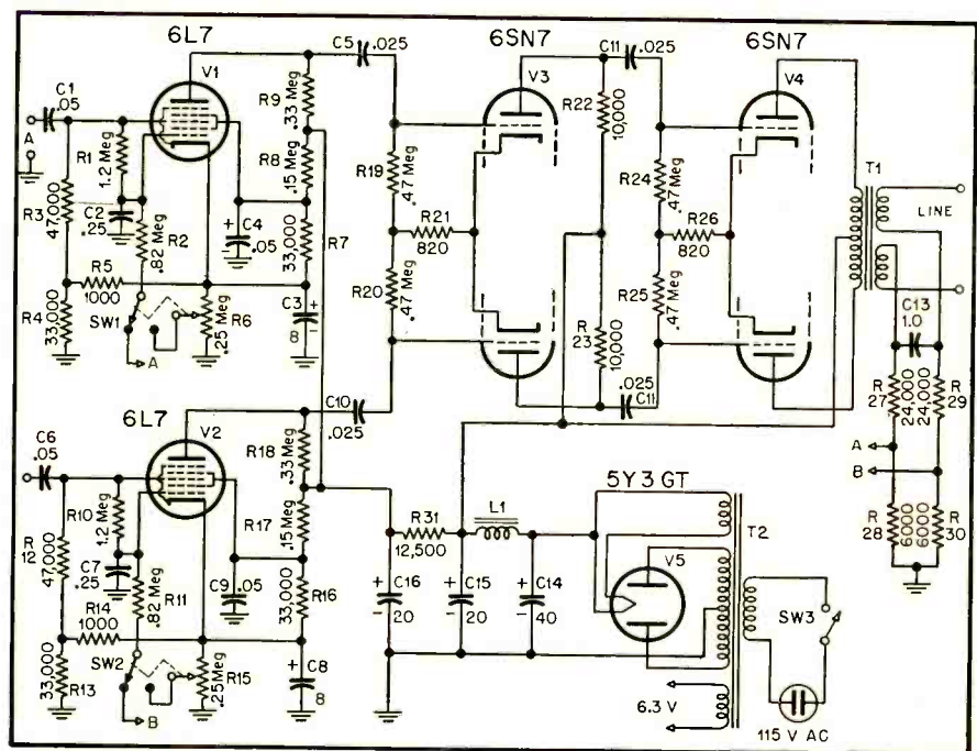
Fig. 1. Circuit schematic for remote gain controlled amplifier.
