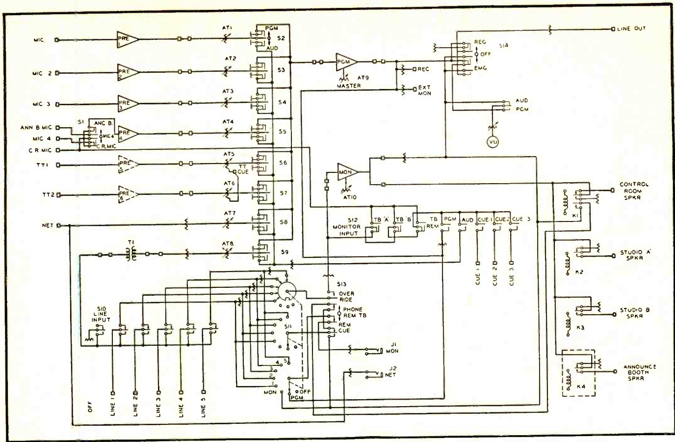
Fig. 3. Simplified block diagram of BC-2B Console.
