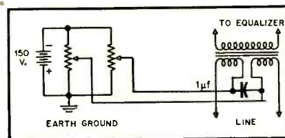
Fig. 3. Suggested connections of studio gain control unit.
