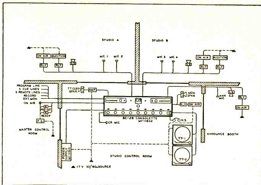
Fig. 4. Simplified diagram showing a typical two-studio station.
