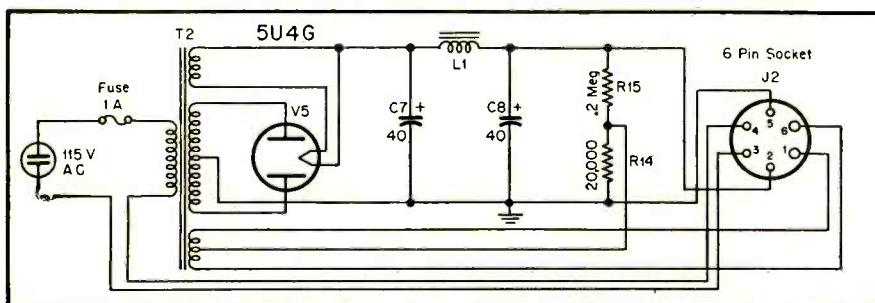
Fig. 3. Schematic of the power supply chassis.
