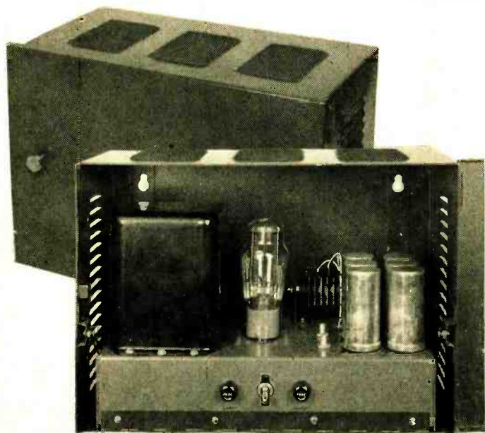
Fig. 5. Power supply used with the console.
