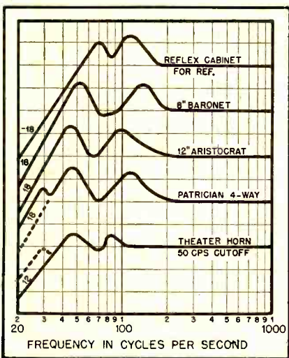
Fig. 6. Typical response curves of reflexed cabinet, several manufactured enclosures, and the folded horn.
