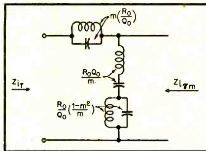
Fig. 8. Series m -derived band-elimination filter half section showing element reactances at center frequency.
