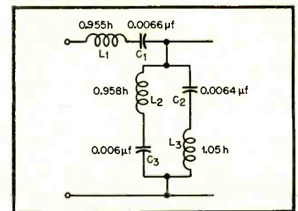
Fig. 10. Band-pass filter half section, series m -derived, showing element values for f_1 = 1950 cps, f_2 = 2050 cps, and R_0 = 1000 ohms.
