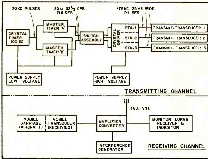
Fig. 3. Block diagram of complete Loran Trainer.
