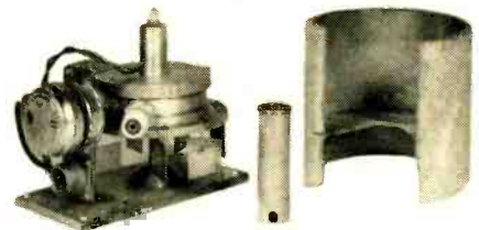
Fig. 7. Transmitting transducer with acoustic shield and projector lens removed to show splitting vanes.
