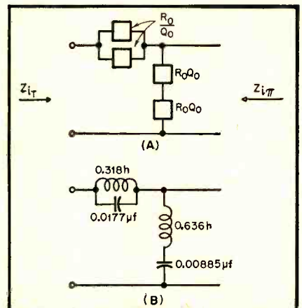
Fig. 6. (A) Basic half section of band elimination filter showing element values at center frequency, and (B) with element values for f_1 = 1500 cps, f_2 = 3000 cps, and R_o = 6000 ohms.
