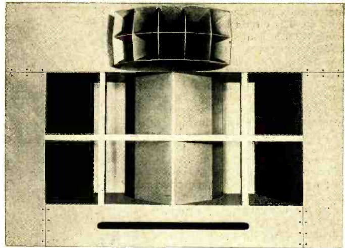
Fig. 5. Front view of typical folded horn.
