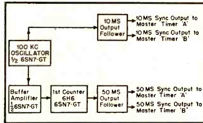
Fig. 4. Block diagram of crystal timer unit.
