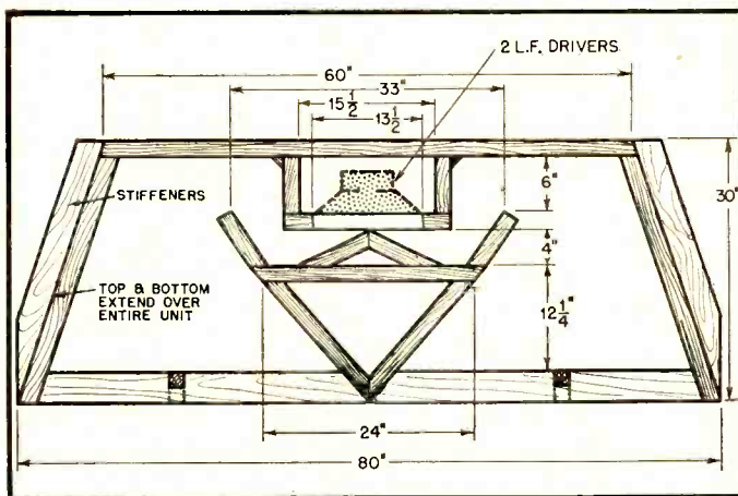
Fig. 4. Cross-section of theatre-type folded horn—the C-5 "bin."
