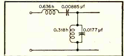
Fig. 5. Band-pass filter half section for 6000-ohm termination and a bandwidth from 1500 to 3000 cps.
