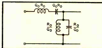
Fig. 4. Band-pass filter half section showing element values of reactances at center frequency.
