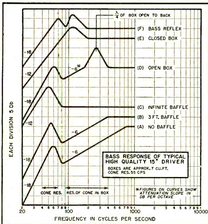
Fig. 2 (left). Comparison low-end response obtainable from various types of speaker mountings. Fig. 3 (right) Optimum size of speaker enclosure for speakers of various diameters and resonant frequencies.
