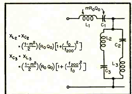
Fig. 9. Band-pass filter half section, series m -derived, showing reactance values in terms of center and upper infinite cut-off frequencies.
