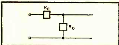
Fig. 1. Basic L section showing element values of reactances at cut-off frequency.
