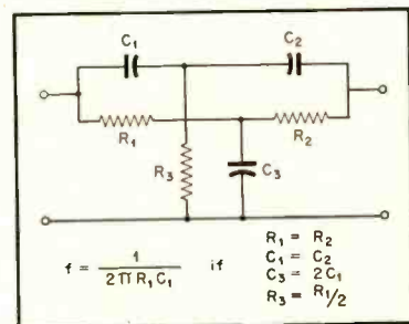
Fig. 4 (above). Parallel-T rejection or null network configuration.
