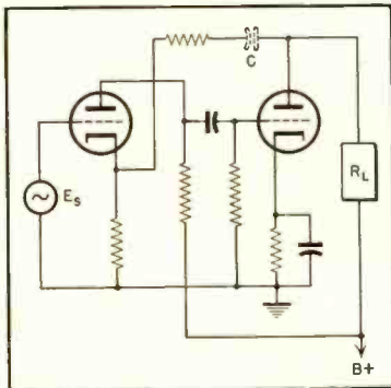
Fig. 6. Conventional feedback amplifier. If AB is equal to that of cathode follower, it will have the same impedance characteristics. Capacitor C may be necessary to maintain proper d.c. relationships.
