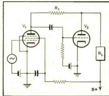
Fig. 4. Suggested drive circuit for Fig. 3B. V_1 is a pentode with R_r \gg R_v .
