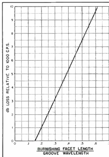
Fig. 2. Generalized effect of burnishing-facet length.
