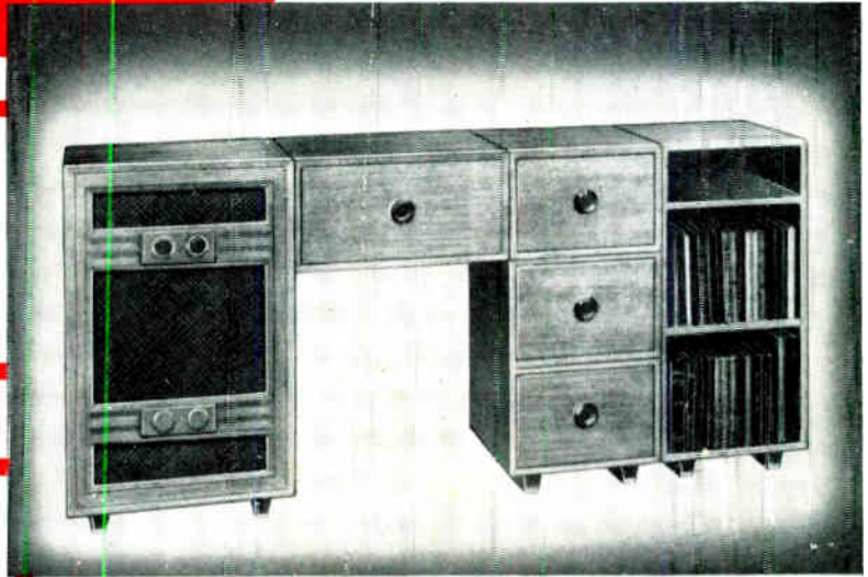
Bass Reflex Reproducer Cabinet for 15" loudspeakers.
