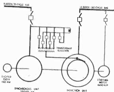
FIG. 3—FREQUENCY CHANGER CONNECTIONS
