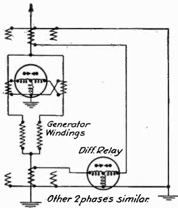
FIG. 10—PARALLEL-WINDING GENERATOR DIFFERENTIAL RELAYS
