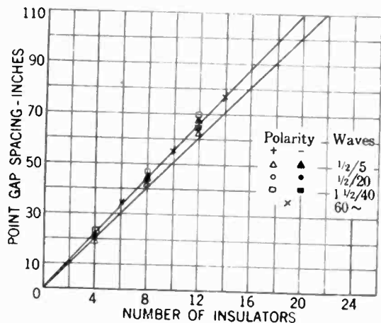
FIG. 14—CURVES SHOWING RESULTS OF PARALLEL TESTS ON STANDARD SUSPENSION INSULATORS ( 5\frac{3}{4} -in. spacing—10-in. diameter) and point-gaps, made to determine equivalent sparkover values. Curves represent range between \beta 0-cycle and 1/2/5 -microsecond waves
