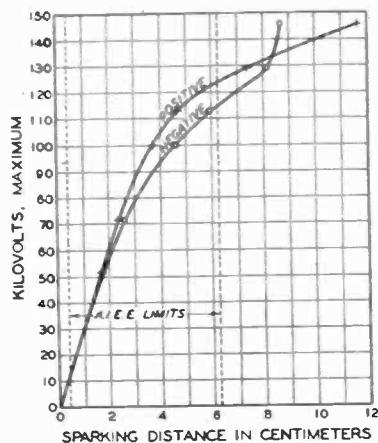
FIG. 6—6.25-CM. SPHERE-GAP IMPULSE SPARK-OVER
