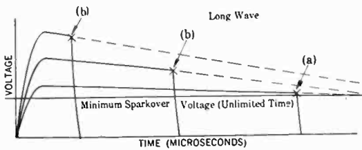
FIG. 3—SPARKOVERS ON TAILS OF WAVES
