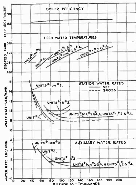
FIG. 6—STATION PERFORMANCE DATA
