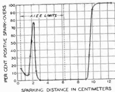
FIG. 5—POLARITY DISTRIBUTION OF 60-CYCLE SPARK-OVERS FOR A 6.25-CENTIMETER SPHERE-GAP
