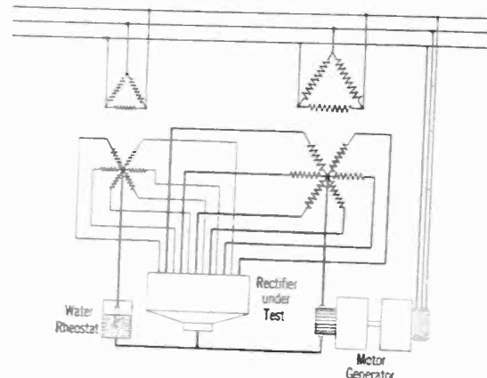
FIG. 3—LOAD TEST OF RECTIFIER—DIAGRAM OF CONNECTIONS
