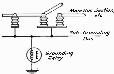
FIG. 8—GROUND PROTECTION
