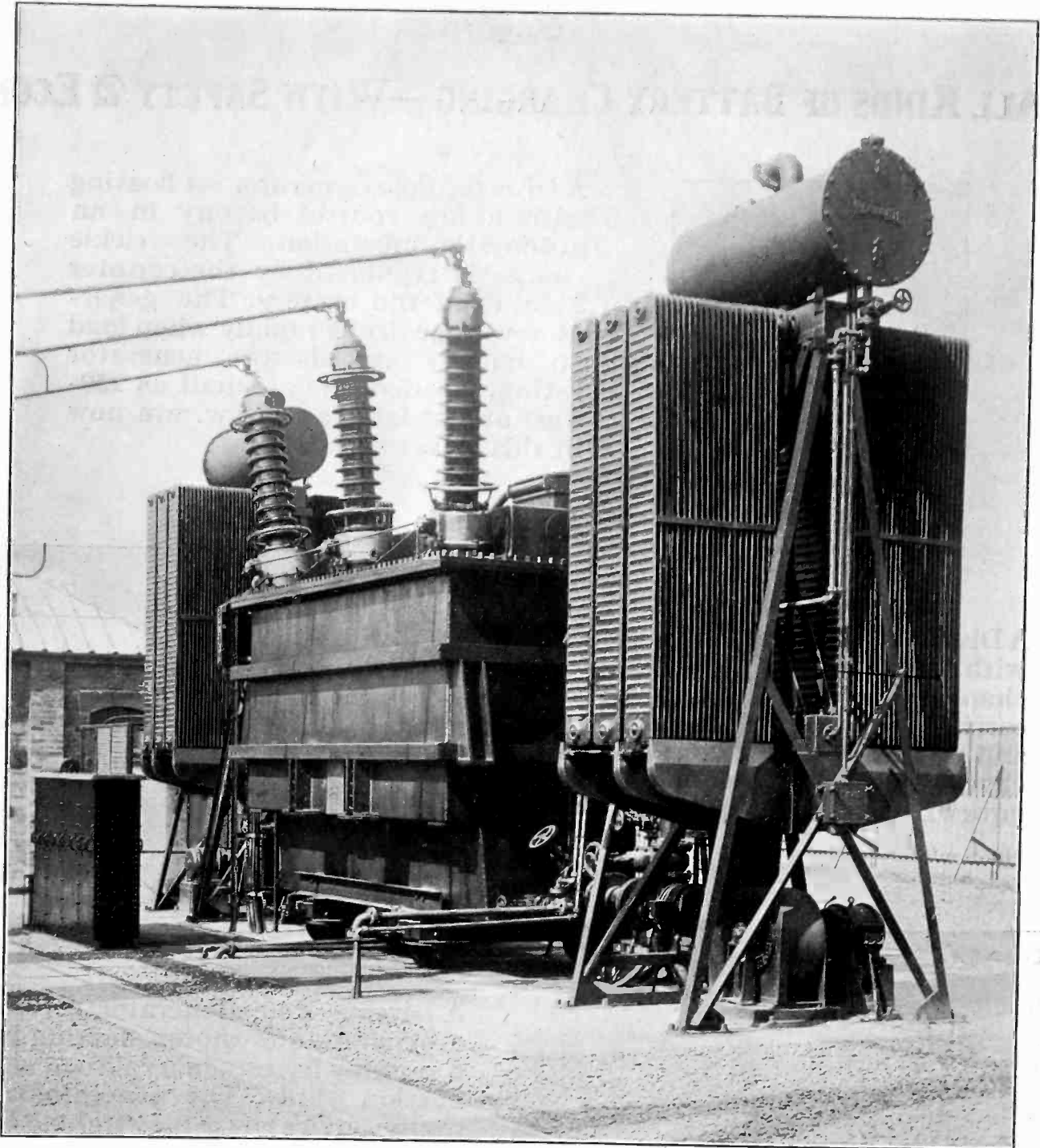
20,000 KV-A., 132 KV., Three-Phase Transformer at Bonnybridge, Scotland
