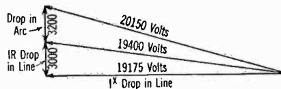
FIG. 6—EFFECT OF RESISTANCE OF AN 8-FT. ARC ON THE IMPEDANCE OF 50 MI. OF SHORT-CIRCUIED 220-KV. LINE
