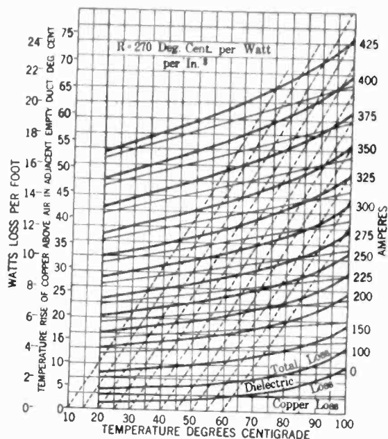
FIG. 7—CHART OF 350,000-CIR. MIL THREE-CONDUCTOR CABLES
