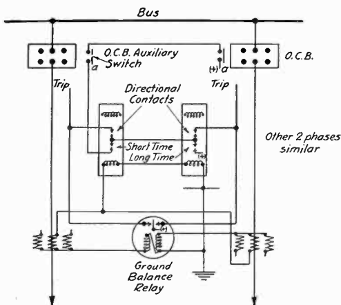
FIG. 3—PARALLEL LINES—CROSS-CONNECTED DIRECTIONAL RELAYS
