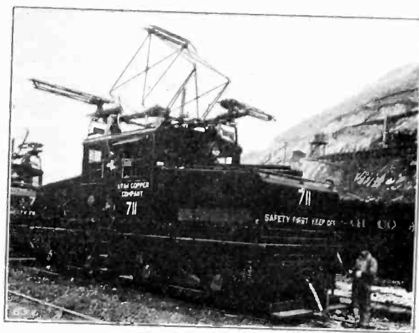
FIG. 7—TYPICAL ELECTRIC LOCOMOTIVE
