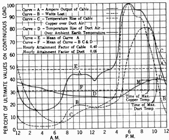
FIG. 10—CHARACTERISTIC TEMPERATURE CURVES
