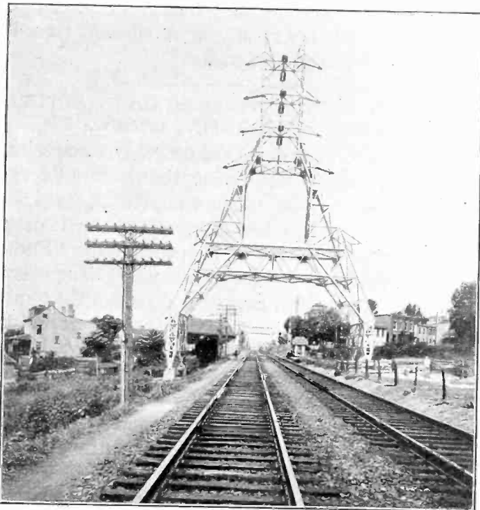
TRANSMISSION LINE TOWERS OVER READING RAILROAD TRACKS
