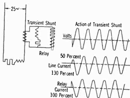
FIG. 1—TRANSIENT SHUNT AND LABORATORY TEST RESULTS
