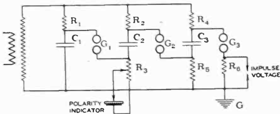
FIG. 4—IMPULSE GENERATOR CIRCUIT
