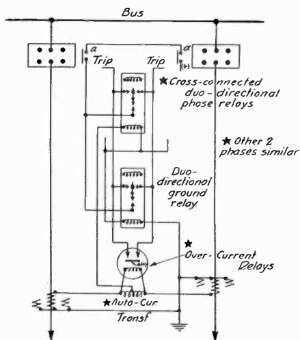
FIG. 4—PARALLEL LINES—CROSS-CONNECTED RELAYS WITH AUTO-CURRENT-TRANSFORMER
