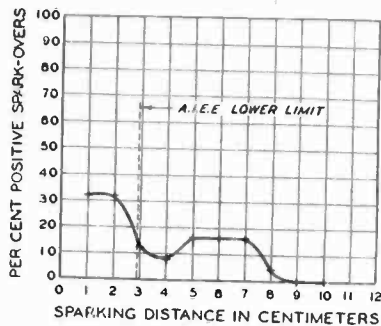
FIG. 7—POLARITY DISTRIBUTION OF 60-CYCLE SPARK-OVERS FOR A 25-CM. SPHERE-GAP
