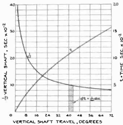
FIG. 7—TIME—TRAVEL CURVE
