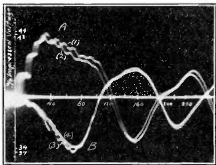
FIG. 8—OSCILLOGRAM SHOWING THE EFFECT UPON THE INTERNAL TRANSFORMER WINDING TRANSIENT SHUNTING NEUTRAL REACTOR WITH SAFETY GAP
