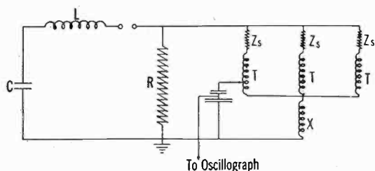
FIG. 2—SCHEMATIC DIAGRAM OF TESTING CIRCUIT
