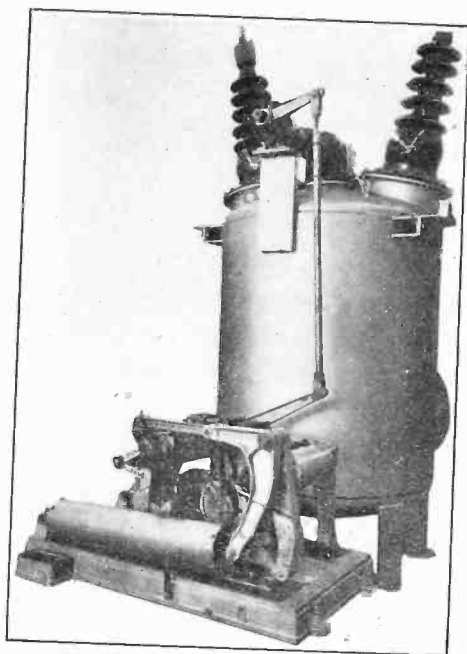
FIG. 1A—OIL CIRCUIT BREAKER WITH CONTROL
