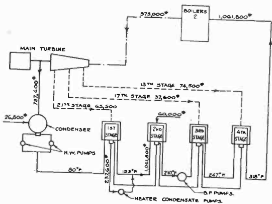
FIG. 4—HEAT BALANCE—UNIT No. 4
