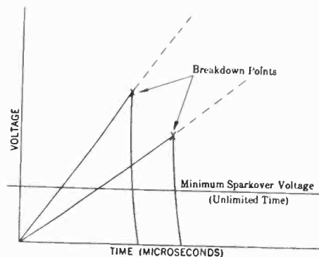
FIG. 2—SPARKOVER ON FRONT OF WAVES OF VARIOUS SLOPES
