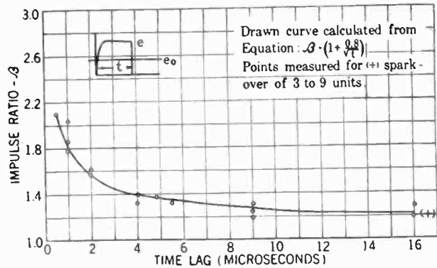
FIG. 5—IMPULSE RATIO-TIME LAG CURVE OF INSULATOR SPARKOVER WITH RECTANGULAR WAVE OF 1/2-MICROSECOND FRONT
