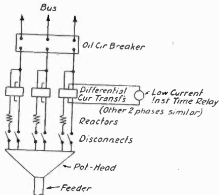
FIG. 1—SPLIT CONDUCTOR
