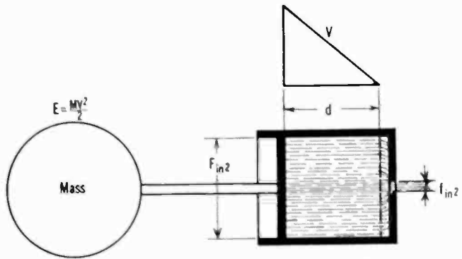
FIG. 11—SCHEMATIC ARRANGEMENT OF DASHPOT
