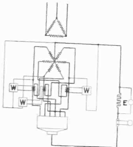
FIG. 2—MEASUREMENT OF RECTIFIER LOSSES—DIAGRAM OF CONNECTIONS
