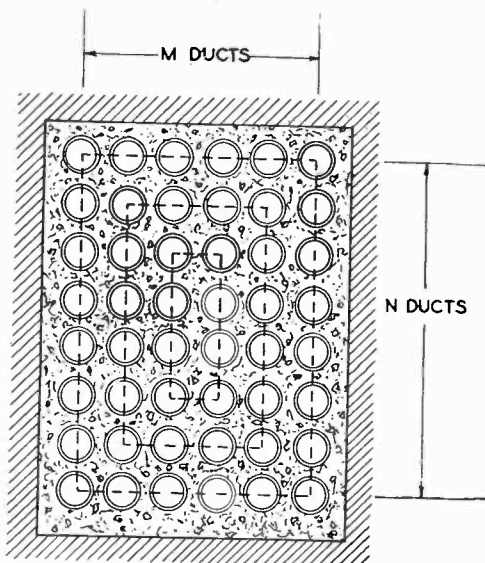
FIG. 12—DUCT BANK SHOWING ASSUMED ISOTHERMAL SURFACES
