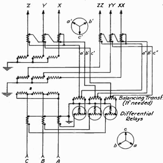
FIG. 9—THREE-WINDING TRANSFORMER
