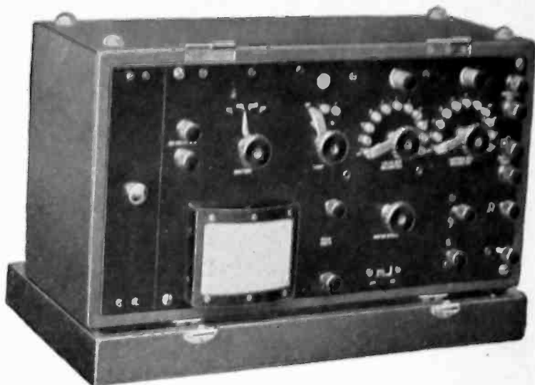
(Left) The Type PM-12 oscillograph with film holder in place for photographing recurrent phenomena
