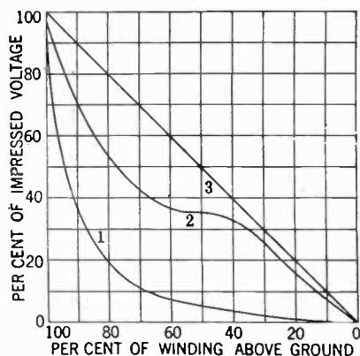
FIG. 3—VOLTAGE-TO-GROUND PRODUCED IN A TRANSFORMER WINDING WITH NEUTRAL SOLIDLY GROUNDED BY A 60-MICRO-SECOND SURGE
