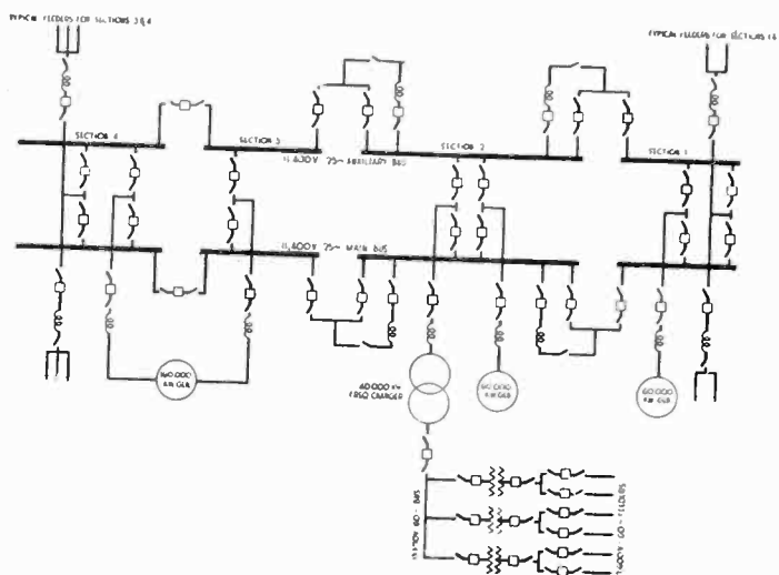
FIG. 5—STATION BUS ARRANGEMENT
