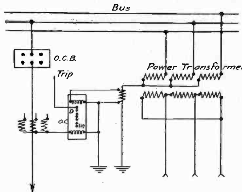
FIG. 5—DIRECTIONAL GROUND RELAY
