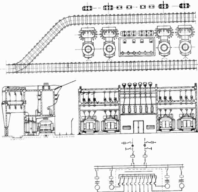
FIG. 8—PROJECT OF LAYOUT OF OUTDOOR RECTIFIER SUBSTATION
