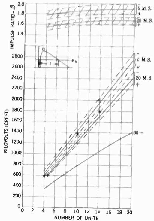
FIG. 12—SPARKOVER VOLTAGES OF SUSPENSION INSULATORS WITH "STANDARD" WAVE—50 PER CENT SPARKING (Standard 5\frac{3}{4} -in. spacing, 10-in. diameter insulators). The full curves should be used for transmission line conditions
