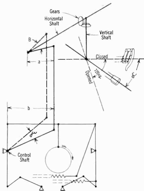
FIG. 3—SINGLE-LINE DIAGRAM OF CONTROL AND BREAKER
