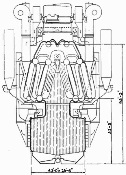
FIG. 1—CROSS-SECTION NEW BOILER UNITS
