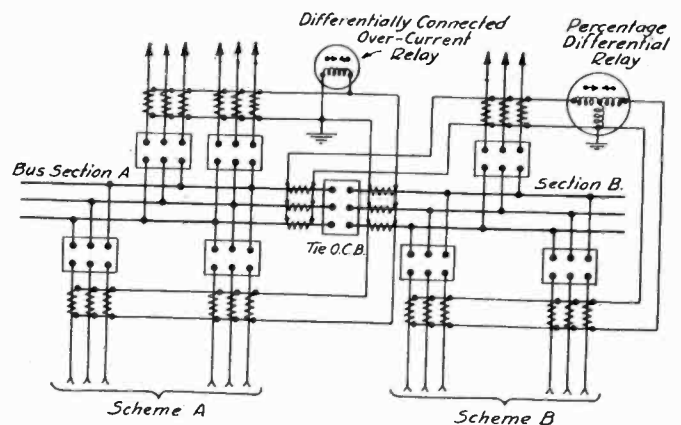
FIG. 7—GROUND PROTECTION NEUTRAL DIFFERENTIAL
