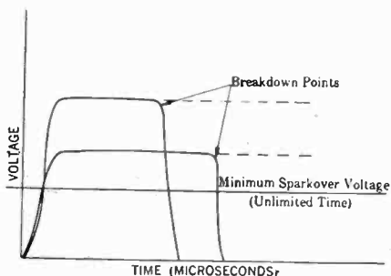
FIG. 1—RECTANGULAR FORM OF IMPULSE WAVE
