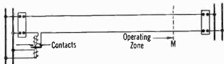
FIG. 3—THE SIMPLE, HIGH-SPEED, IMPEDANCE RELAY
