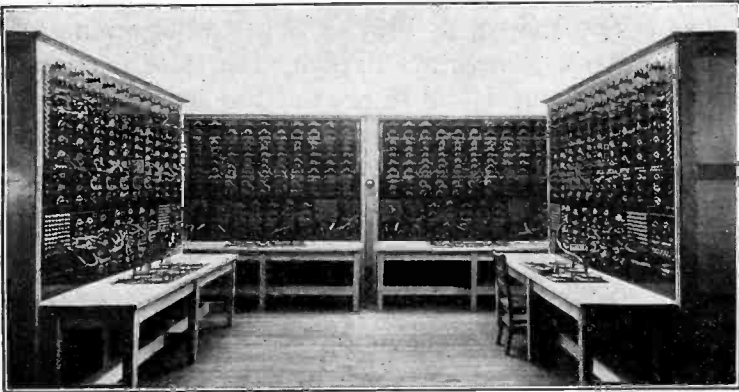
FIG. 1—THE NETWORK ANALYZER
