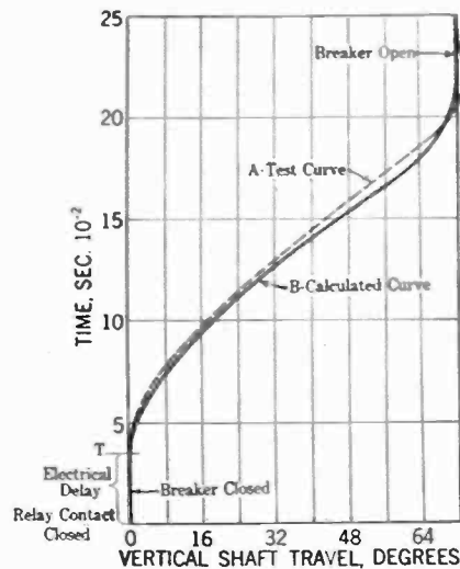
FIG. 14—TRAVEL-TIME CURVES. COMPARISON BETWEEN CALCULATION AND TEST
