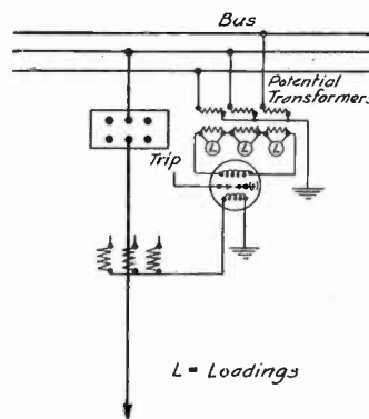
FIG. 6—POWER DIRECTIONAL GROUND RELAYS
