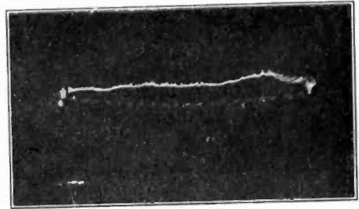
FIG. 7—FLASHOVER OF 22 "B" INSULATORS, STRAIN POSITION
