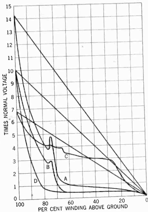
FIG. 14—PROBABLE MAGNITUDE OF INTERNAL VOLTAGES ABOVE GROUND
