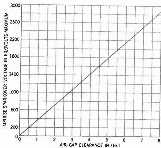
FIG. 5—SPARKOVER VOLTAGE OF AIR-GAPS
