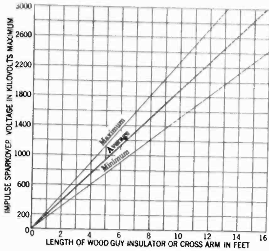
FIG. 4—SPARKOVER VOLTAGE OF WOOD GUY INSULATORS AND WOOD CROSSARMS
