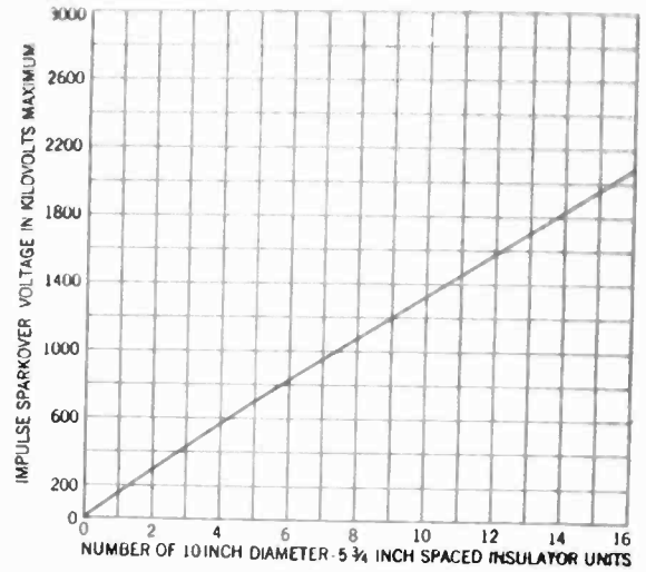
FIG. 6—SPARKOVER VOLTAGE OF SUSPENSION INSULATORS
