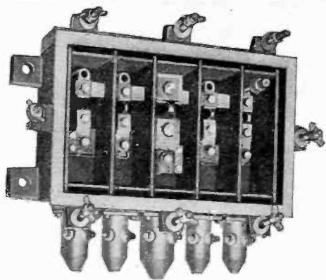
TYPE "FB" BOTTOM ENTRANCE BOX 1500Mcm main—4-500Mcm branches
