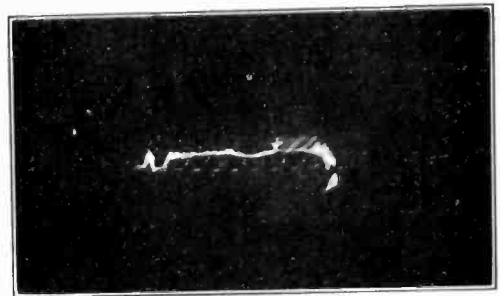
FIG. 8—FLASHOVER OF 10 "A" INSULATORS, STRAIN POSITION
