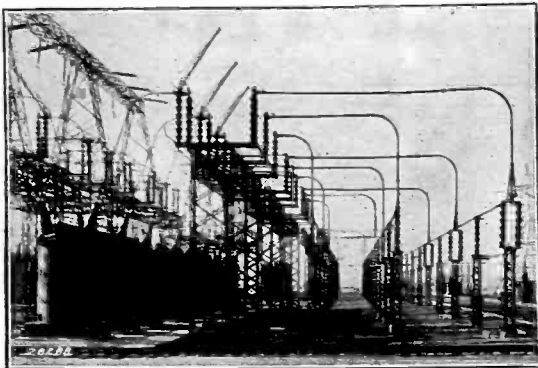
Plymouth Meeting Station of PHILADELPHIA ELECTRIC COMPANY showing installations of Elpeco Monel Metal fitted switches.
