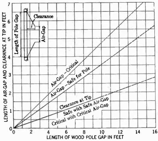
FIG. 10—HORN-GAP PROTECTION OF WOOD POLES
