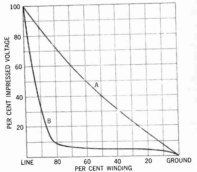
FIG. 7—COMPARISON OF VOLTAGE DISTRIBUTION IN LONG AND SHORT STACKS OF COILS
