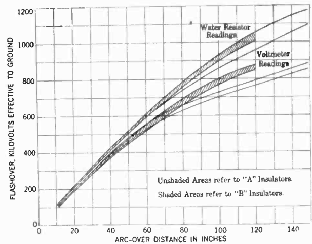
FIG. 1—FLASHOVER OF SUSPENSION INSULATORS, STRAIN POSITION, UNSHIELDED
