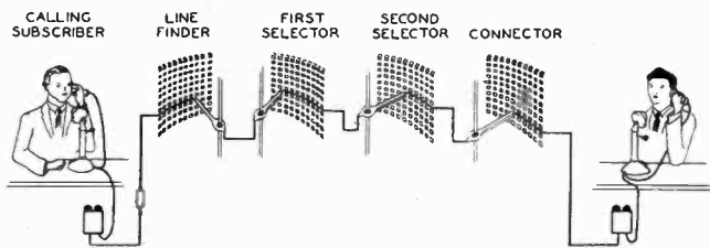
FIG. 7—PATH OF LOCAL CALL—SMALL DIAL OFFICE
