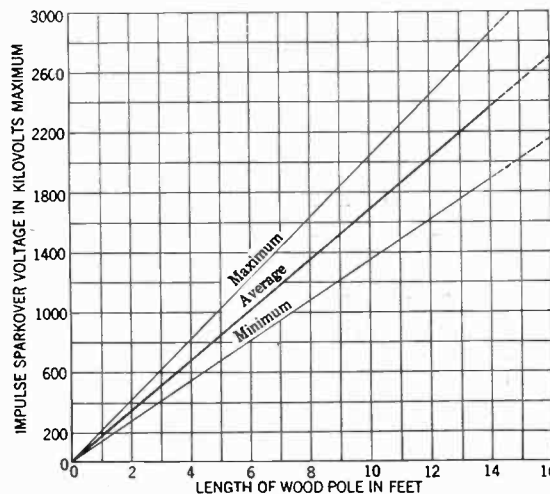
FIG. 3—SPARKOVER VOLTAGE OF WOOD POLES
