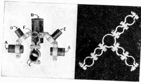
THREE STANDARD BRACES (For Unequal Sizes of Pipe)
