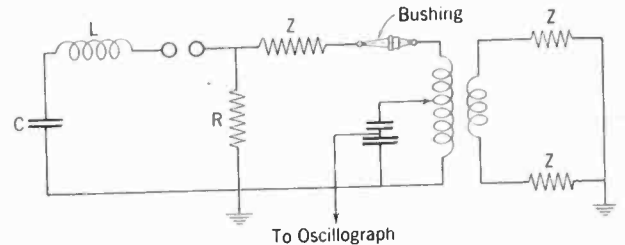
FIG. 5—SCHEMATIC DIAGRAM OF TESTING CIRCUIT
