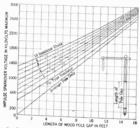
FIG. 8—SPARKOVER VOLTAGE OF INSULATORS AND WOOD POLE
