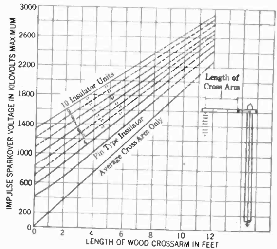
FIG. 7—SPARKOVER VOLTAGE OF INSULATORS AND WOOD CROSSARM
