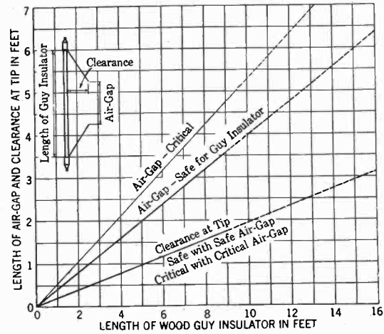
FIG. 11—HORN-GAP PROTECTION OF WOOD-GUY INSULATORS
