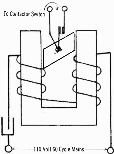
FIG. 8—SCHEMATIC DIAGRAM OF RESONANT RELAY
