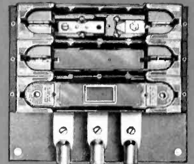
Bottom unit in "on" position, middle unit with head removed showing live parts guarded, top unit with guard removed. Shows connections to busbars and mounting screws.
