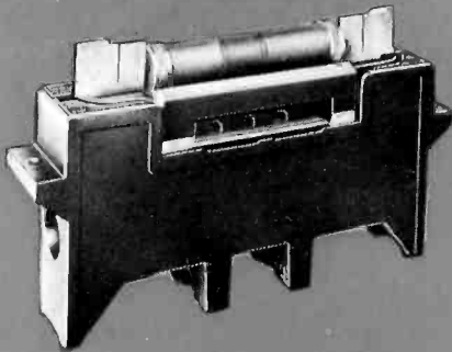
Bull Dog Unit-Versal SAFTOFUSE Unit, 200 Amperes, 600 Volts. In "off" position.
