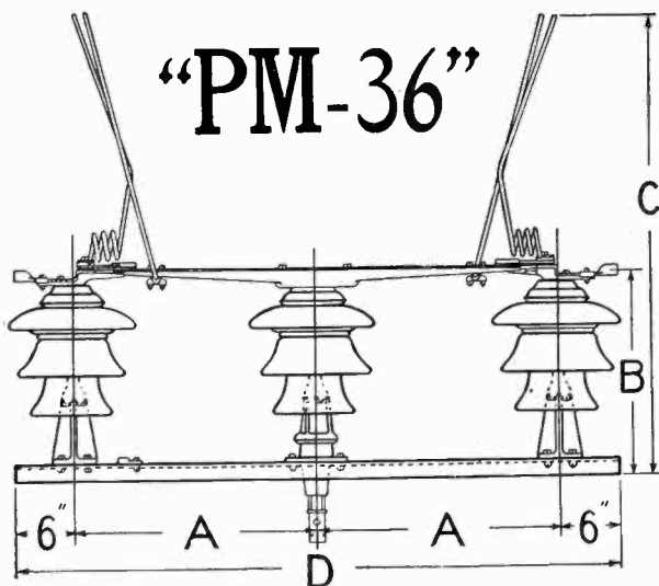
Construction of 50 k. v. and 73 k. v. Switches
