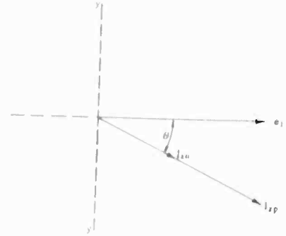
FIG. 9—DIAGRAM ILLUSTRATING THE PRINCIPLE OF REFLECTION
