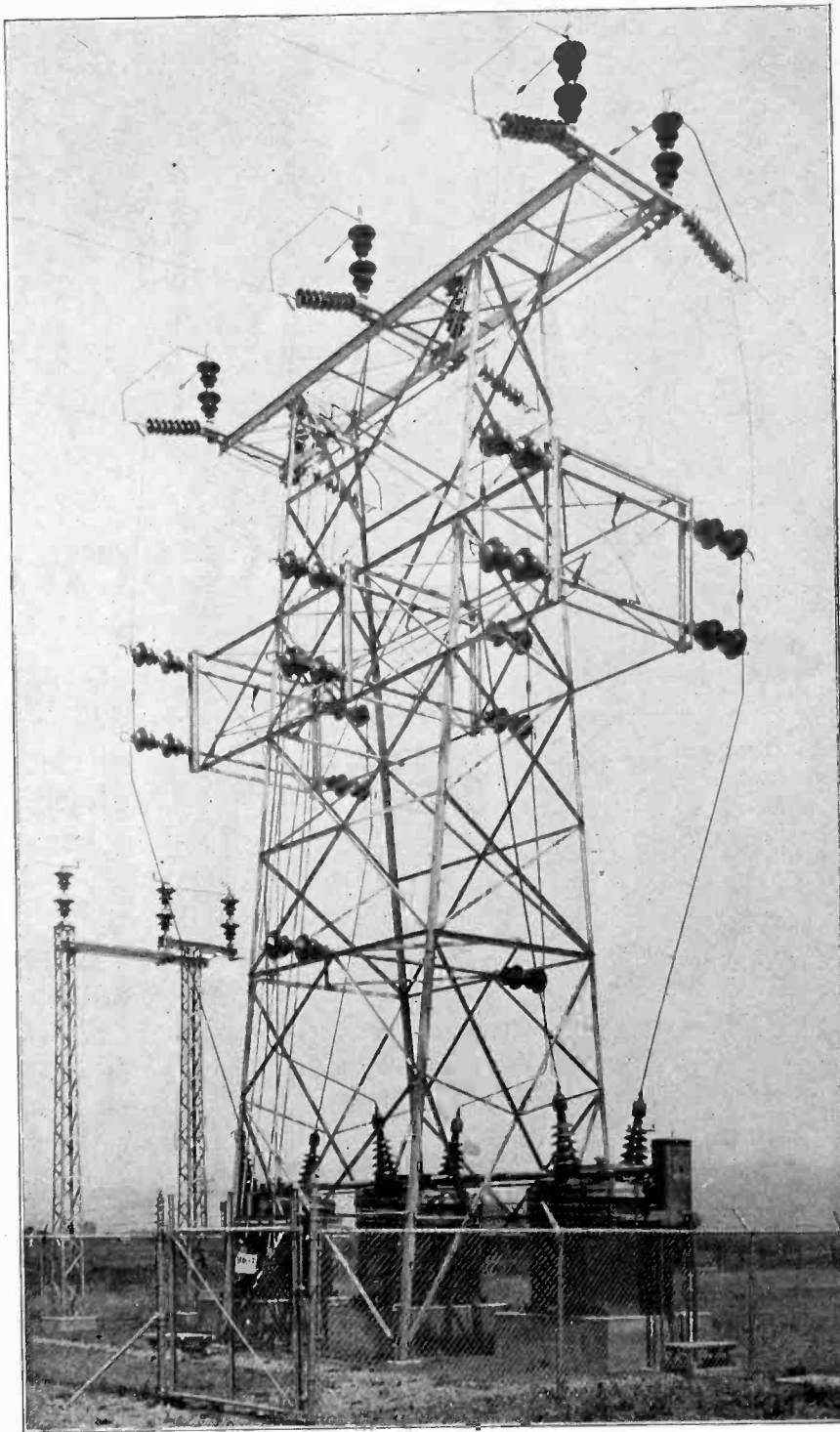
Pacific Type "R," 110 Kv., 400 Amp., Oil Circuit Breaker installation at Tie-in of Pacific Gas & Electric Company with Coast Valleys Gas & Electric Company (Byllesby Engineering and Management Corporation), Salinas, California.
