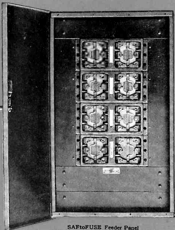
SAFtoFUSE Feeder Panel 30-60 Amperes, 250 Volts; 3-3 Wire Units.
