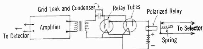
FIG. 4—SCHEMATIC SHOWING METHOD OF OPERATING POLARIZED RELAY
