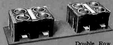
Double Row Double Branch Panel Unit with Plug Fuse Branch Connections.
