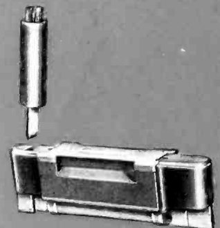
Head of motor testing SAFTOFUSE Unit. Shows motor-testing head and test jack.
