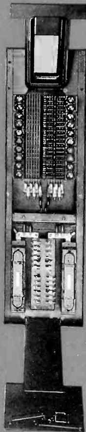
Bull Dog Unit-Versal Rigid Type Metering Panel combined with SAFToFUSES, closed and with hinged cover plates open.
