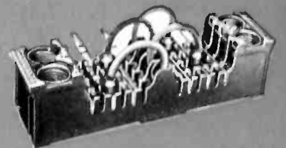
Flexo type metering panel unit, without locking bars.
