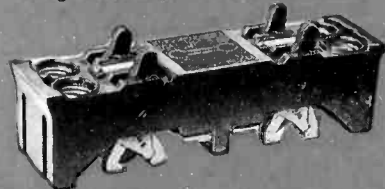
Double Branch Panel Unit with 4 Heavy Duty, single pole Bull Dog Toggle Switches and Plug Fuse Connections—4 circuits.
