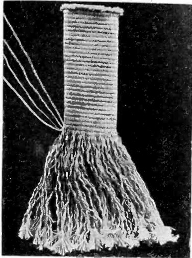
Hazard Spiralweave covering before treating with weatherproof compound.
