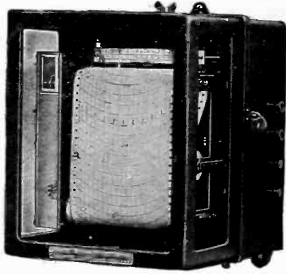
Bristol's Recording Wattmeter Strip Chart type; for single, two or three phase current.
