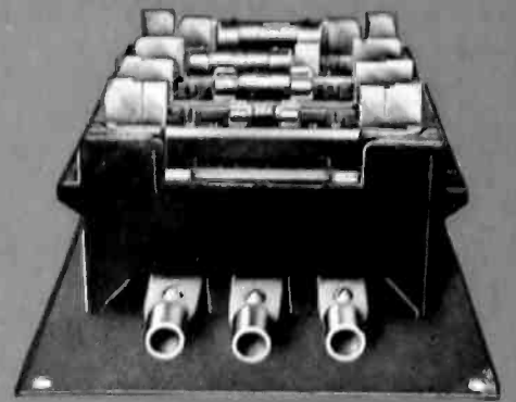
SAFTOFUSE Units, convertible, same unit arranged for 30, 60, 100 or 200 ampere, 250 volt fuses. All units "off."
