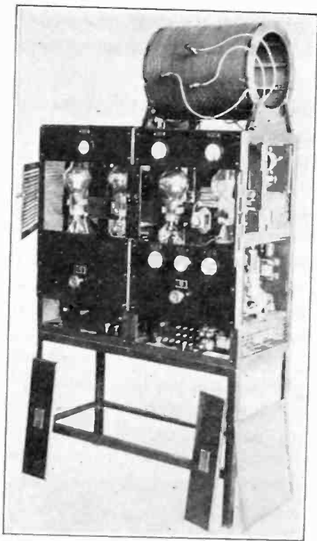
FIG. 2—TYPE OF TRANSMITTER INSTALLED AT KOKOMO
