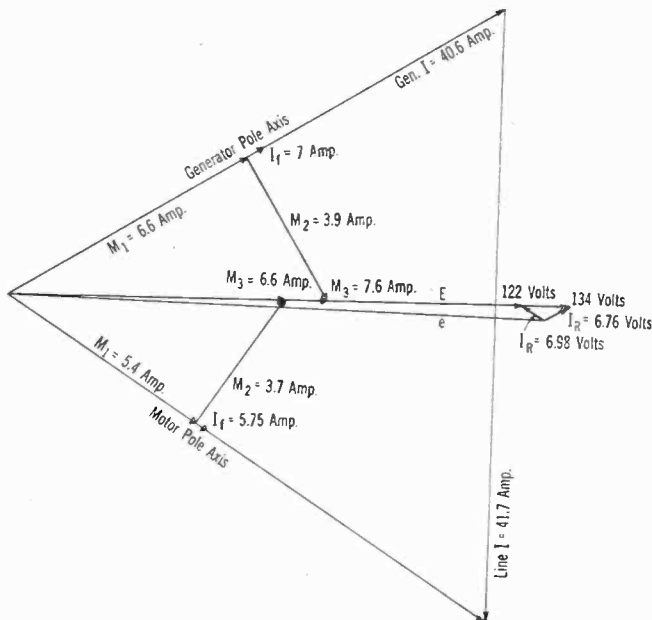
FIG. 2—COMPLETE SOLUTION BY VECTOR DIAGRAM
