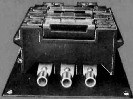
Bull Dog Unit-Versal SAFTOFUSE Units mounted on busbars. In "on" position.
