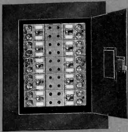
Bull Dog Unit-Versal Lighting Panel Cabinet. 5 Double Branch Units with 10 double pole Toggle Switches and Plug Fuse Connections—10 circuits.
