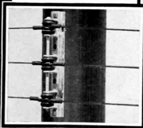
Installation of Peirce No. 3746 Secondary Rack on a pole. Two 3/8-inch Through Bolts are used for making this installation.
