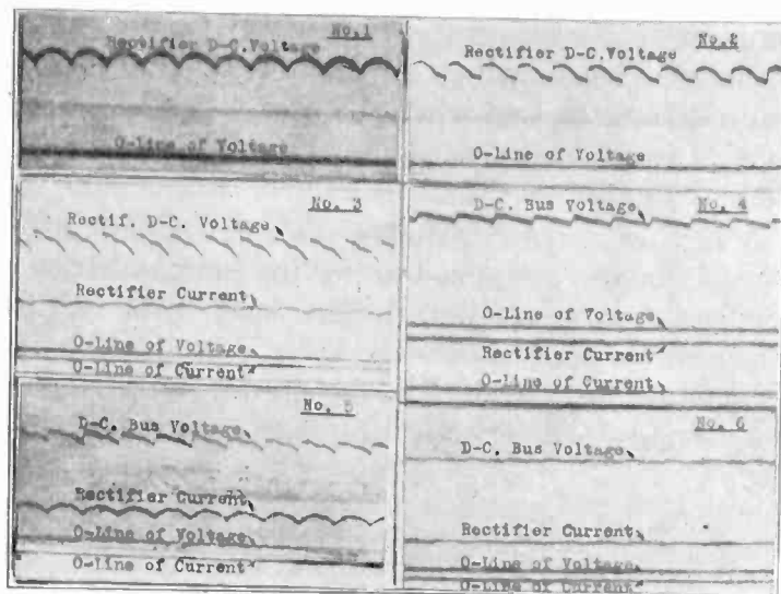
FIG. 13—OSCILLOGRAMS OF VOLTAGES AND CURRENTS OF A 1500-Kw., 1500-VOLT RECTIFIER
