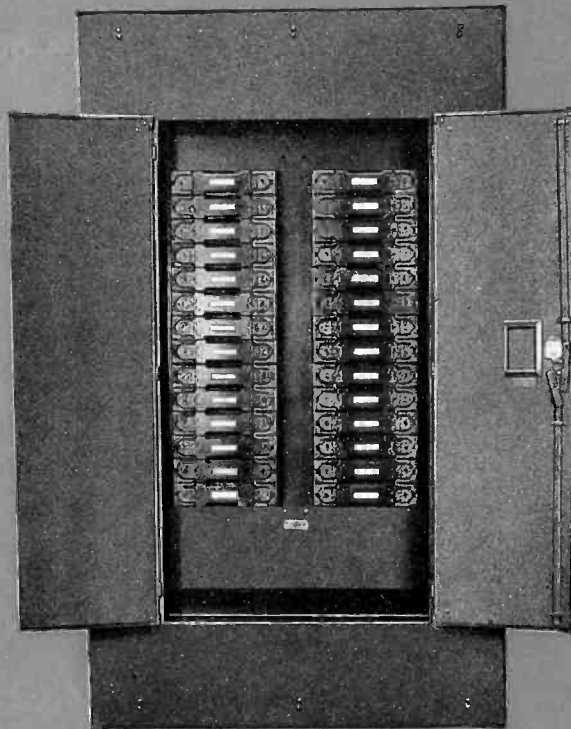
Double Row SAFtoFUSE Panel built for Detroit Edison Company.
