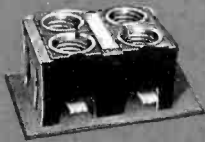
Double Branch, Bull Dog Lighting Panel Unit, with Plug Fuse Branch Connections.
