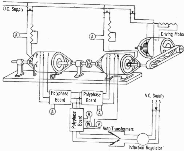
FIG. 1—INDUCTION REGULATOR
