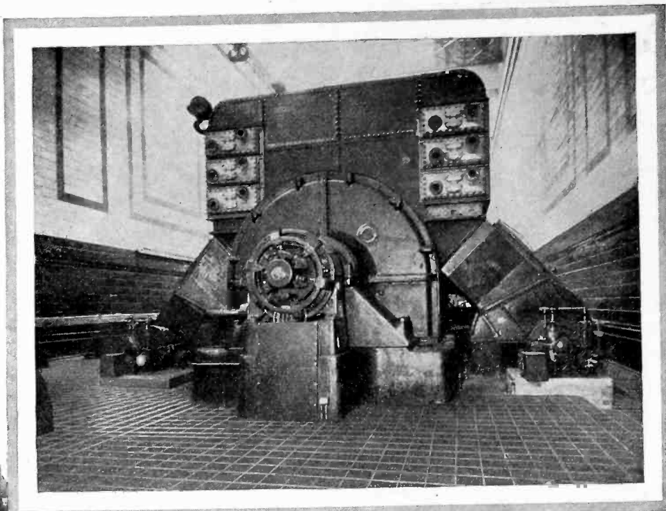
50,000-kw. G-E turbine-generator, East River Station, New York Edison Company. Surface air coolers are mounted on the generators—a suitable location where space is not available below the machine
