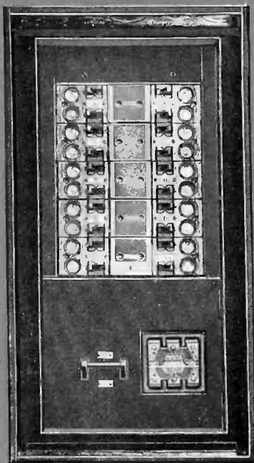
Bull Dog Unit-Versal Lighting Panel. 5 Double Branch Units, Main Toggle Switch and SAFtoFUSE. 20 single pole branch Toggle Switches and Plug Fuse Connections—20 circuits.
