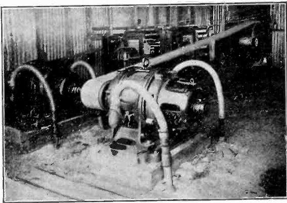
FIG. 3—INSTALLATION OF TWO 15/35-H. P. PUMPING MOTORS FOR CABLE-TOOL DRILLING
