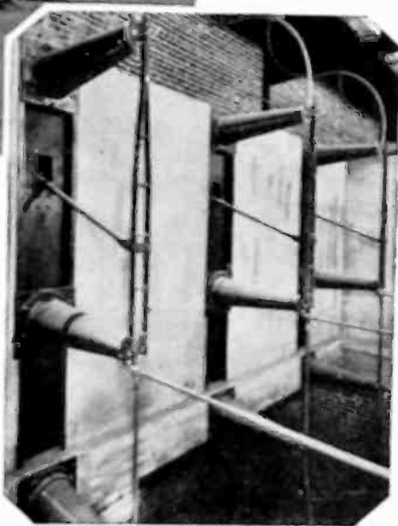
Motor-operated disconnecting switches at La Gabelle. O-B post insulators.
