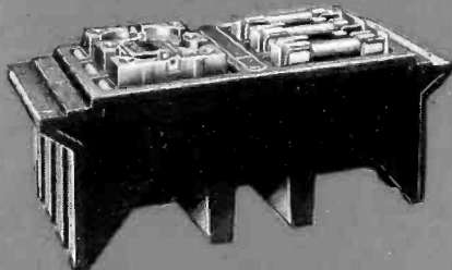
Double Branch, 3-3 Wire SAFTOFUSE Unit, 30 or 60 ampere branches; one unit "on" and one unit "off".
