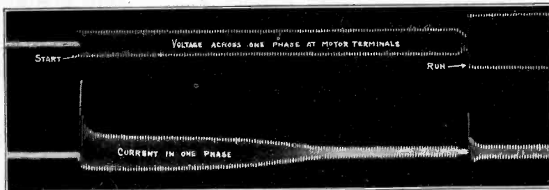
This oscillogram illustrates the serious current inrush drawn by a compensator when first thrown on the line, due to the excessive magnetizing current required for the compensator core.
