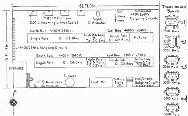
FIG. 1—FIRST FLOOR PLAN OF AUTOMATIC SUBSTATION “E”, KANSAS CITY POWER & LIGHT CO.
