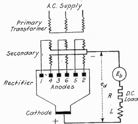
FIG. 7—SIX-PHASE RECTIFIER WITH GENERALIZED D-C. LOAD
