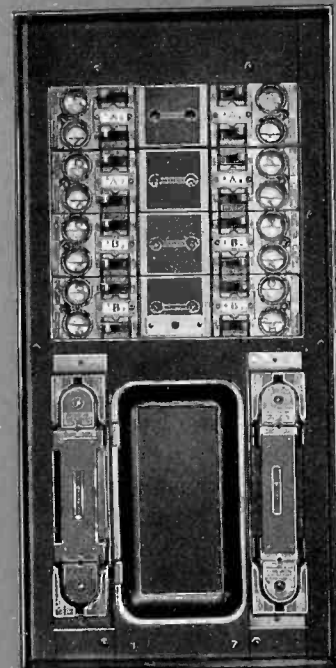
Bull Dog Unit-Versal Lighting Panel. 4 Double Branch Units and 2 Main SAFtoFUSES. 16 Bull Dog Toggle Switches and Plug Fuse Connections—16 circuits.
