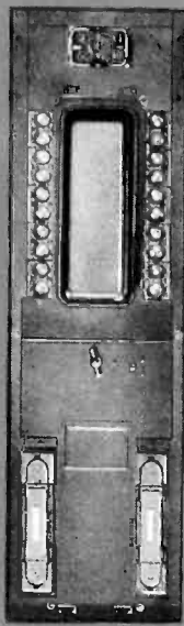
Rigid bar type metering panel unit, with insulating guards and meter bar connections.
