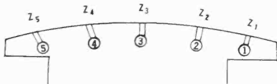
FIG. 2—SYMMETRICAL GROUP OF DAMPER BARS
