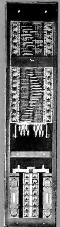
Bull Dog Metering Flexo Type Panels combined with lighting panel and SAFToFUSE Units, cover plates removed.
