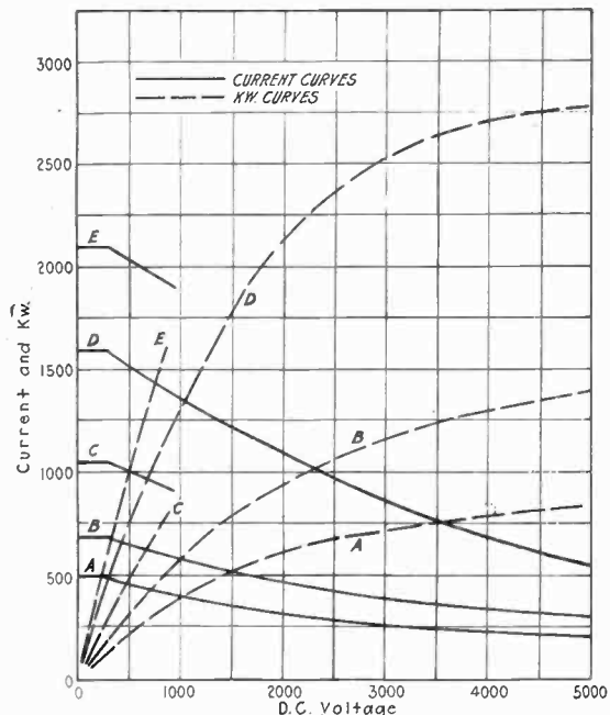
FIG. 6—LOAD CURVES OF BROWN BOVERI RECTIFIERS SHOWN IN FIG. 4
