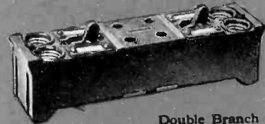
Double Branch Panel Unit with 2 Heavy Duty, Double Pole Toggle Switches and Plug Fuse Connections—2 circuits.
