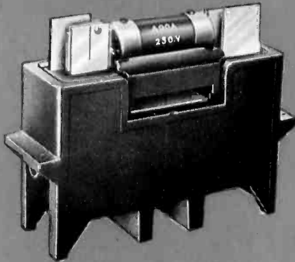
Bull Dog Unit-Versal SAFTOFUSE Unit, 400 Amperes, 250 Volts. In "off" position.
