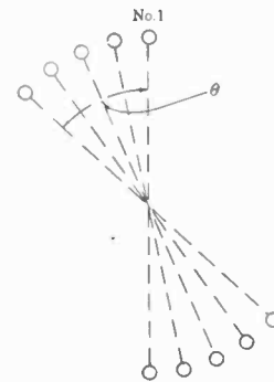
FIG. 4—M. M. F. PRODUCED BY A NUMBER OF COILS DISTRIBUTED OVER ANGLE \theta TO THE LEFT OF COIL NO. 1
