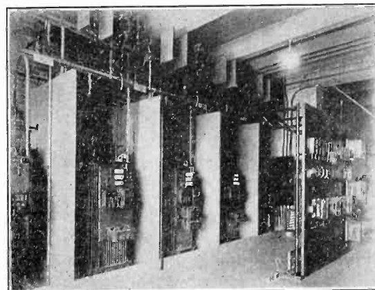
FIG. 3—SECTION OF SINGLE-PHASE REGULATORS AND PANEL FOR RECLOSING OIL CIRCUIT BREAKER EQUIPMENT
