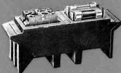
Double Branch, 3-2 Wire SAFTOFUSE Unit, 30 or 60 ampere branches; one unit "on" and one unit "off".
