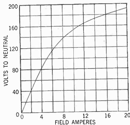
FIG. 5—SATURATION CURVE
