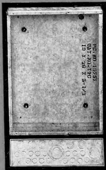
Standardized Panelboard Boxes furnished in various sizes. Width 19 inches, 4-inch wiring gutters. 128 knockouts in each.
