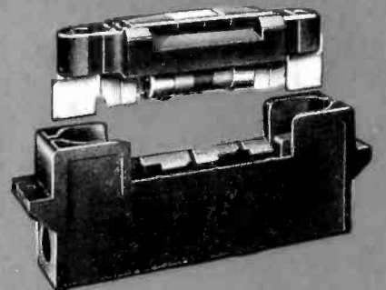
Bull Dog Unit-Versal SAFTOFUSE Unit. Flat type used on lighting panelboards. Shows head of unit drawn out of body.
