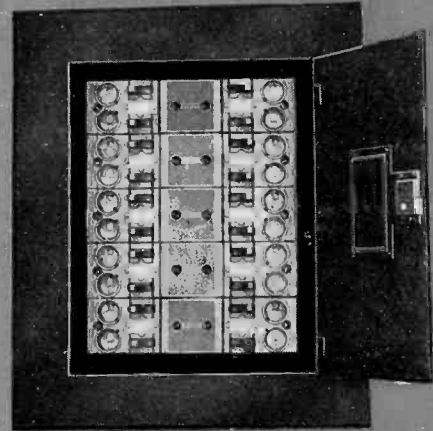
Bull Dog Unit-Versal Lighting Panel Cabinet. 5 double Branch Units with 20 Bull Dog Toggle Switches and Plug Fuse Connections—20 circuits.
