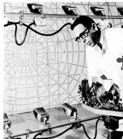
11. RCA broadcast equipment at a new uhf station in Trenton.
