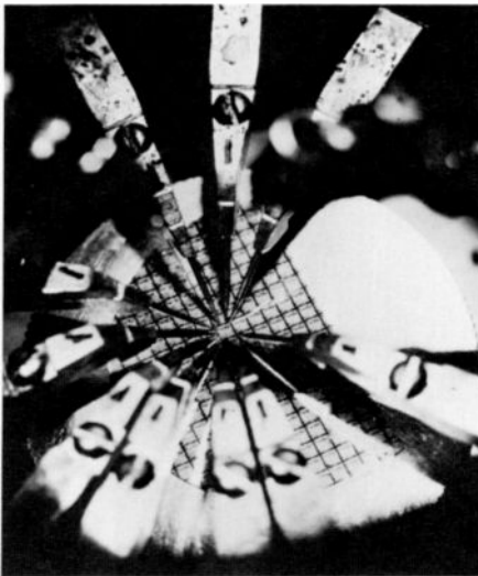
1. The assembly area in RCA's 250,000-square-foot equipment facility at Marlboro, Mass.
