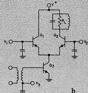
Fig. 8—Tuner-amplifier configurations of the basic differential amplifier.
