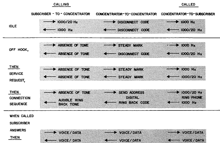
Fig. 4—Call-sequence diagram.
