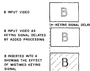
Fig. 3—Uncorrected video delay results in substandard edge and insert.
