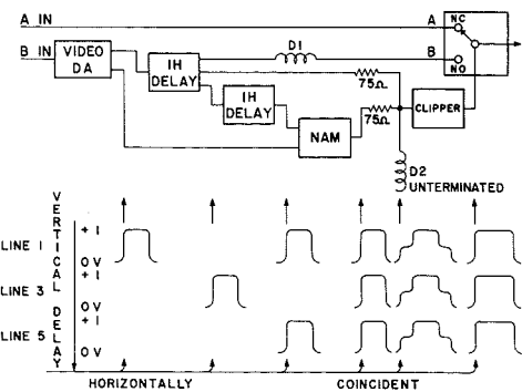
Fig. 6—Implementation of the 6-element matrix.
