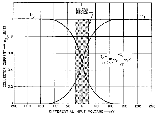
Fig. 12—Limiting characteristic of a differential amplifier.
