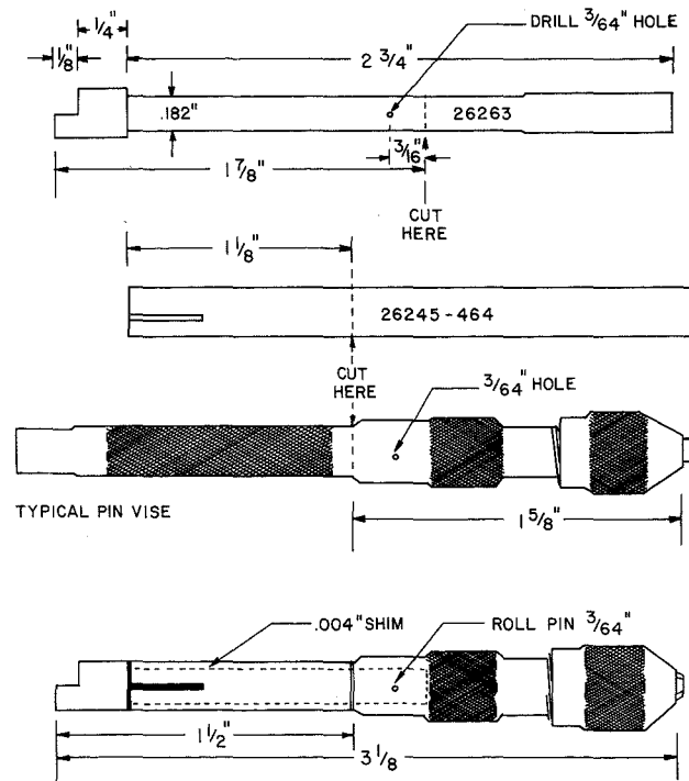
ASSEMBLED DRILL CHUCK BIT
