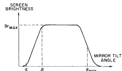
Fig. 4a—Screen brightness versus tilt of target plane: \alpha \approx amount by which stop size exceeds source size; \beta \approx collimation angle of incident light; and \theta_{max} \approx acceptance angle of projection lens.
