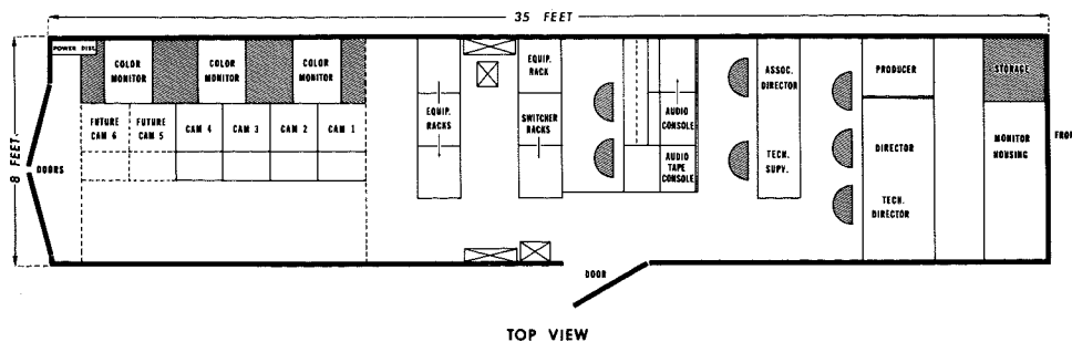
Fig. 4—CG-3 mobile unit interior layout.
