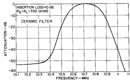
Fig. 6—Typical response curve for a ceramic filter.
