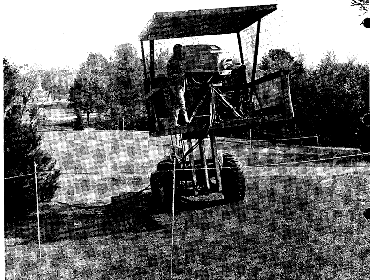
Fig. 4—Right, NBC color camera on a fork lift at Firestone Country Club at Akron, Ohio.
