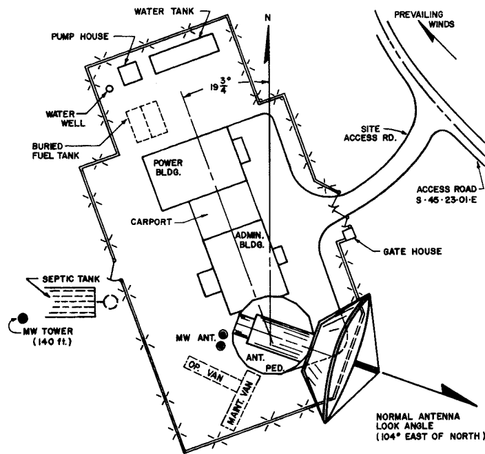
Fig. 2—Earth station site plan.
