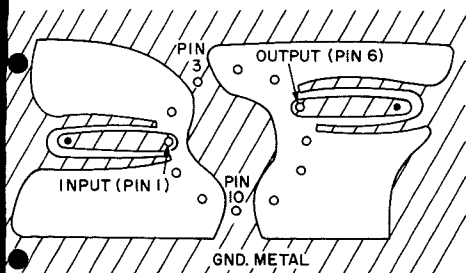
SHADED REGIONS ARE PC-BOARD METAL AREAS
