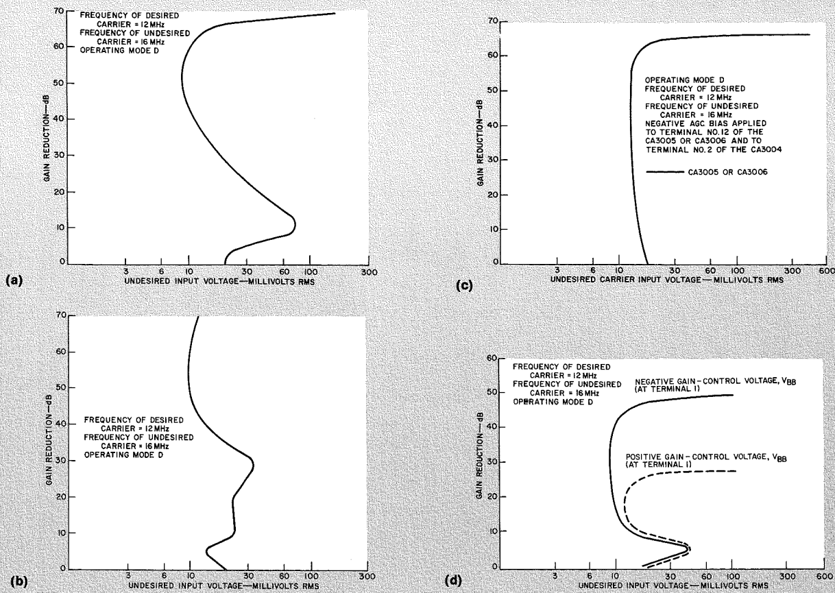
Fig. 11—AGC characteristics of the basic IC amplifiers using CA 3005: a) cascode mode with negative AGC applied to the base of transistor Q_3 ; b) cascode mode with AGC applied to turn on transistor Q_1 ; c) differential amplifier operation with AGC applied to base of Q_3 ; d) forward and reverse AGC.
