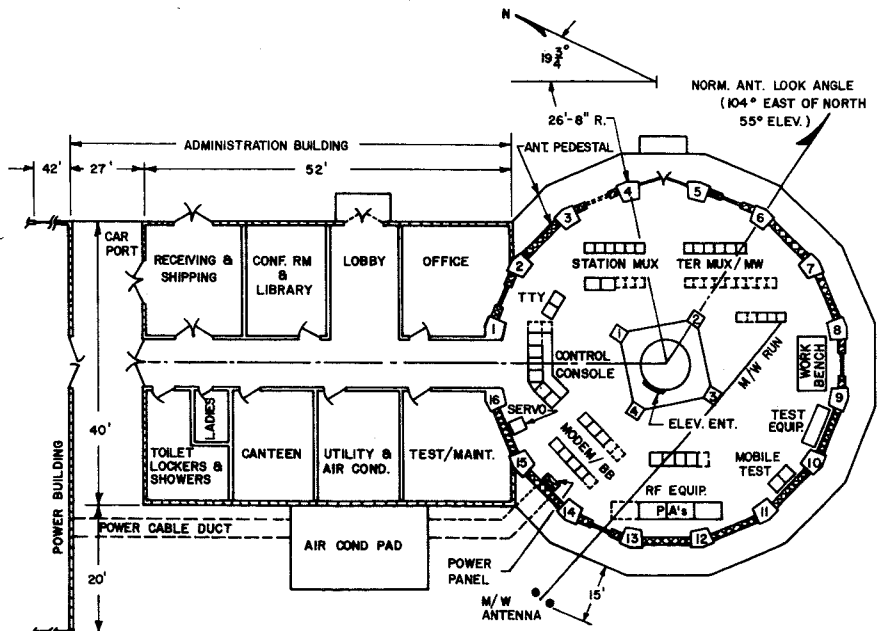
Fig. 3—Equipment facilities layout.
