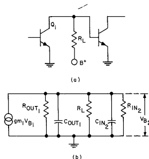
Fig. 4—a) Transistor interstage network and b) its equivalent circuit.
