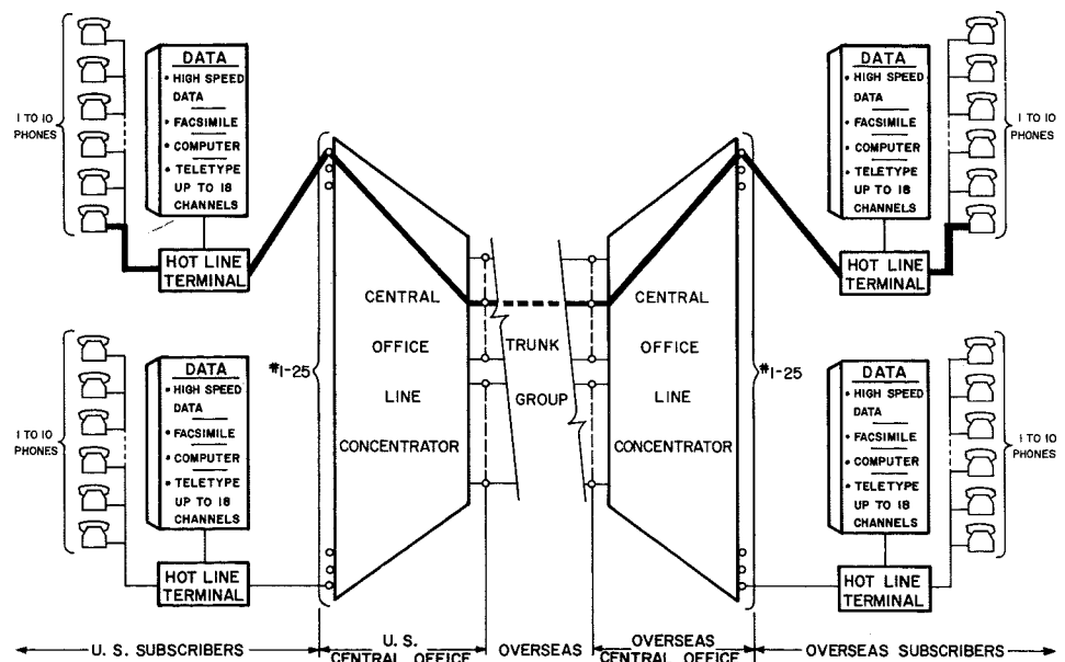
Fig. 1—System configuration.
