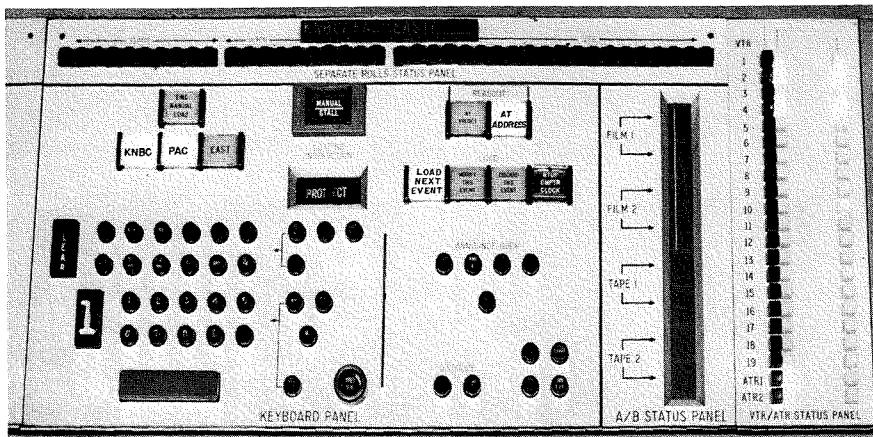
Fig. 1—Switching-central keyboard.
