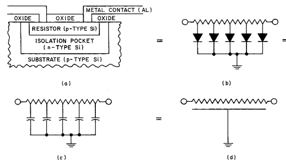
Fig. 5—Integrated-circuit resistor and its equivalents.
