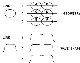
Fig. 5b—A 6-element matrix where the picture element is larger than two times border width.
