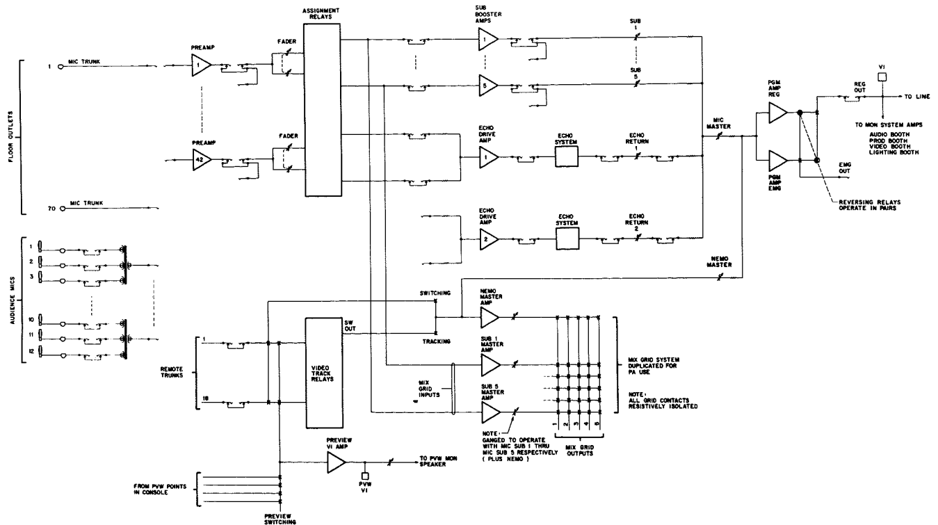
Fig. 8—Simplified block diagram of the audio control system.
