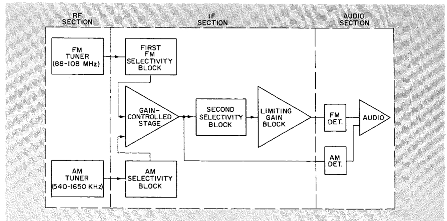
Fig. 3—Block diagram of AM/FM receiver.
