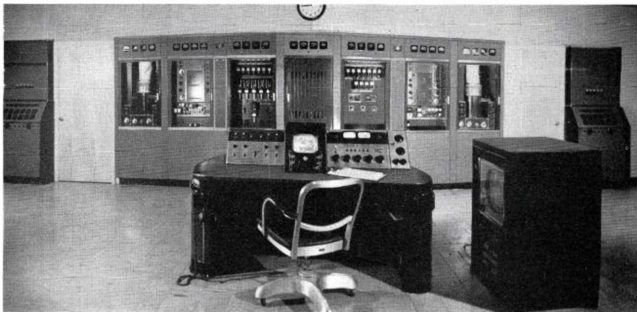
FIG. 2. WISH-TV TT-50AH Transmitter showing in-line arrangement of final amplifiers with driver units. (Distortion in picture is due to use of two negatives.)
