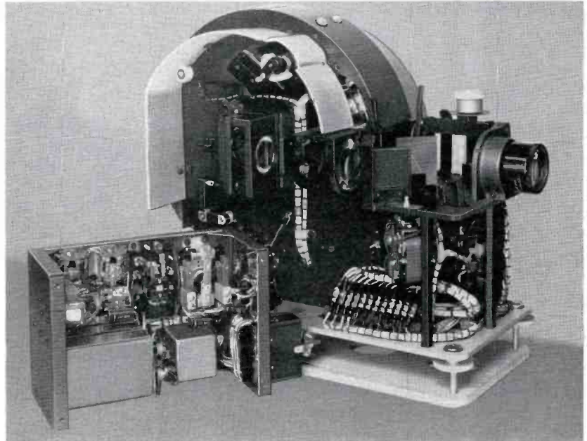
FIG. 11. A plexiglass shield in close proximity to the internal diameter of the drum collects spill-over light to provide slide check viewing.
