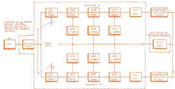
SIMPLIFIED BLOCK DIAGRAM—BTA-50G TRANSMITTER
