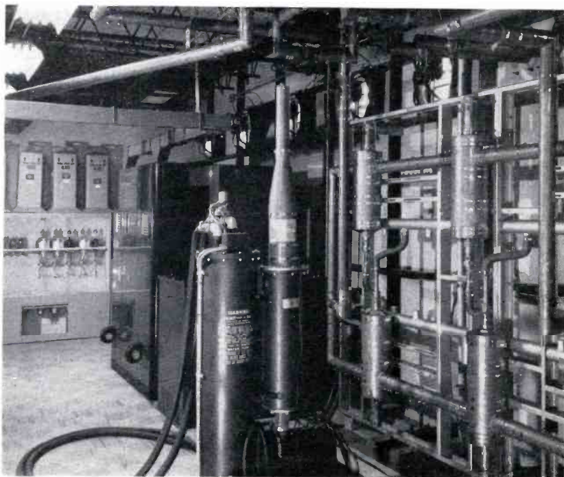
FIG. 4. Area behind TV transmitter. Left to right, spare tube cabinet, high-voltage rectifier, dummy load, and portion of vestigial sideband filter.
