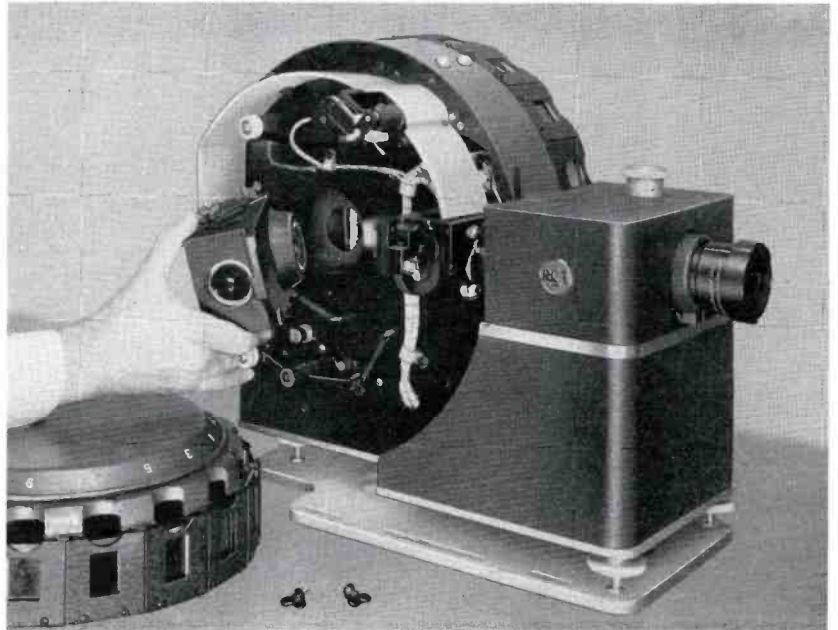
FIG. 12. Drums, drum covers and optical assemblies are easily accessible for cleaning. Projector can be kept dust free with minimum effort.
