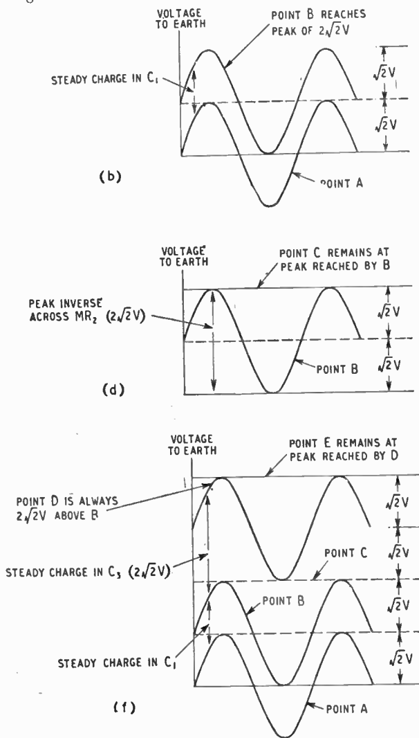
Fig. 6. Principle of operation of the Cockcroft-Walton voltage multiplier.
