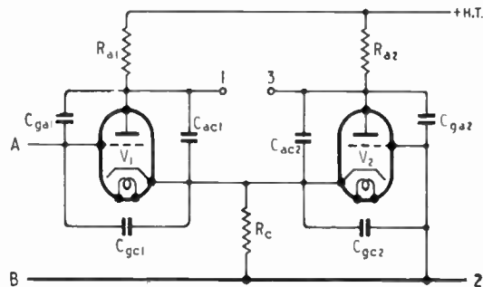
Fig. 29. This diagram shows the various inter-electrode capacitances of the valves, which influence the performance at high frequencies.
