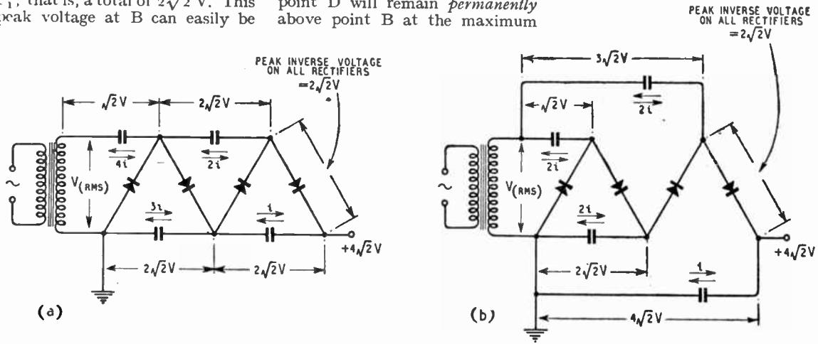
Fig. 7. (a) Series-fed multiplier; all capacitors, except the first, charge to equal voltages, but must carry different currents. (b) Parallel-fed multiplier; all capacitors, except the last, carry equal currents, but must withstand different voltages
