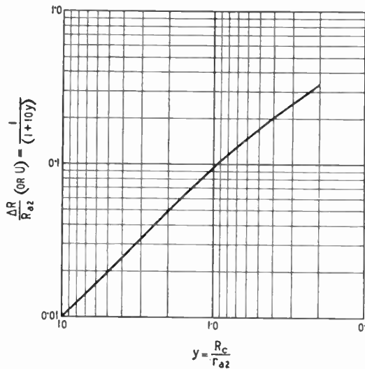
Fig. 26. This curve shows the relation between unbalance for equal values of R_{a1} and R_{a2} or the fraction by which R_{a1} must be less than R_{a2} for balance as a function of y=R_c/r_{a2} for the condition \mu_2=29 and R_{a2}/r_{a2}=2 .
