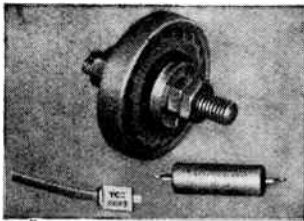
T.C.C. Micadisc lead-through capacitor for radio-heaters, CE70B 30- \mu\text{F} , 15-V electrolytic, and midget silvered-mica by-pass capacitors.
