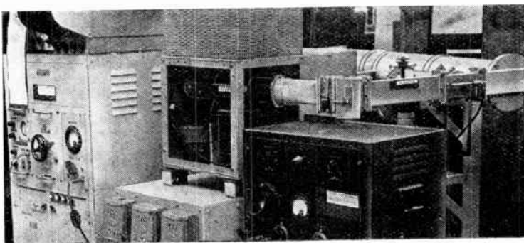
Pulsed magnetron (left) and wave-guide system energizing multi-cell cylindrical resonator for accelerating electrons in the range 5 to 20 Mev (G.E.C. Research Labs).
