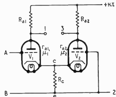
Fig. 24. Cathode-coupled circuit reduced to its simplest form.
