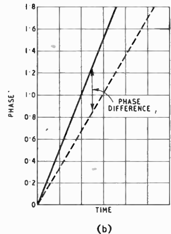
Fig. 4. Graph of progressive phase difference between two similar waves of different frequency, Fig. 2(a) and (d), according to two different definitions of phase difference.
