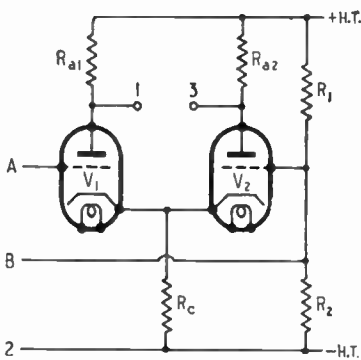
Fig. 27. Bias can be obtained from a voltage divider R_1, R_2 across the H.T. supply.
