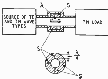
Filter designed to pass transverse magnetic waves.
