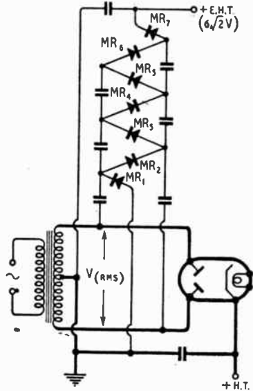
Fig. 11. The multiplier of Fig. 10 may be directly connected to a transformer which is already supplying H.T. through a normal rectifier (shown in heavy lines). Both E.H.T. and H.T. supplies then have a common earthed negative pole.
