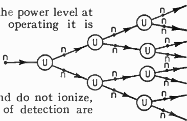
Fig. 9. Diagrammatic representation of a chain reaction illustrating the growth of the neutron n population by the fission of uranium atoms (U) on the assumption that two neutrons are emitted at each fission.
