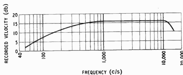
Proposals for standardization of groove, reproducing stylus and recording characteristic put forward by Mr. Mittell.
