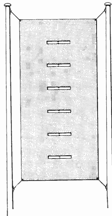
Fig. 4. Suggested stack of slots to give directional gain in the vertical plane with vertically polarized radiation.
