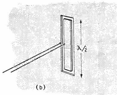
Fig. 3. Folded dipole diagram (a) with the corresponding folded slot (b)
