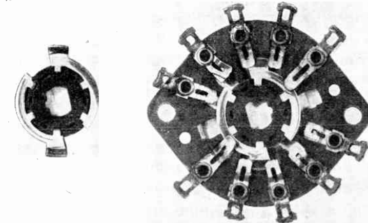
Photograph of typical wafer switch, subjected to mechanical life test after cleaning with carbon tetrachloride.
