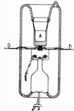
Grounded-grid triode.
