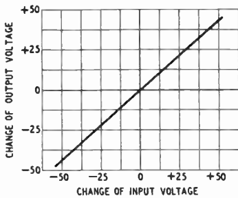
Fig. 13. Dynamic characteristics of the phase-splitter.
