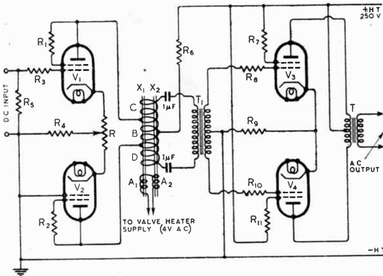
Fig. 4. Practical circuit with values suitable for use with KT41 valves throughout, R_1, R_2, R_7, R_{11} = 200\Omega ; R_3, R_8, R_{10} = 0.03 M\Omega ; R_4 = 100\Omega ; R_5 = 0.5 M\Omega ; R_6 = 8000\Omega ; R_9 = 50\Omega . Potentiometer R = 30\Omega .
