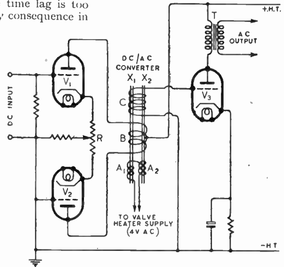
Fig. 2. DC/AC converter with high-impedance valve input circuit.
