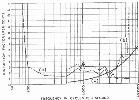
Fig. 1. Harmonic distortion in 12-inch cone loudspeaker (a) with single variable frequency, (b) with constant 60 c/s input and a variable frequency of equal power, (c) calculated FM distortion. Curve (b) represents the sum of both cross-modulation and FM distortion.
