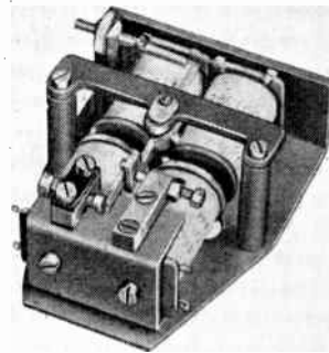
Four-coil polarised relay of specially sensitive type ( Automatic Telephone and Electric Company ).
