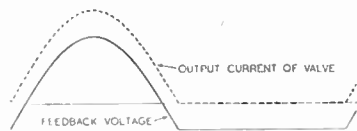
Fig. 1. Output current of valve biased to cut-off with sine wave input.
