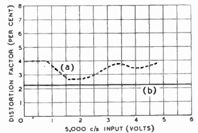
Fig. 3. Distortion in a 12-inch speaker with constant 60 c/s input and variable 5000 c/s input. (a) Observed total distortion, (b) calculated FM distortion.
