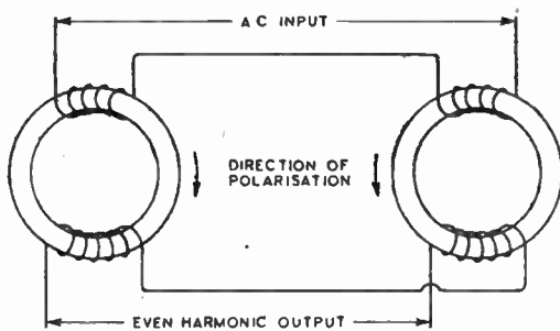
Fig. 1. Circuit for separation of even harmonics.
