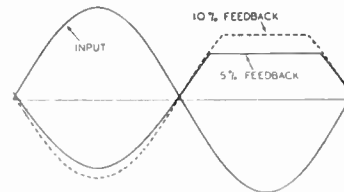
Fig. 2. Output of valve biased to cut-off with AC negative feedback.
