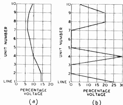
Courtesy "Journal I.E.E." Fig. 5. Potential distribution on 10-unit insulator string. (a) Relative humidity 42% (b) Relative humidity 95%.
