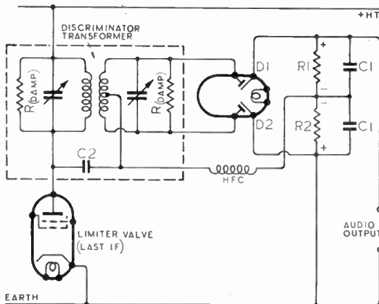
Fig. 1. Type of discriminator circuit used in modern American frequency-modulation receivers.
