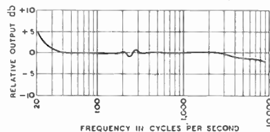
Fig. 3. Response curve of finished pick-up taken with HMV DB4037 and Decca EXP55 and corrected for recording characteristic. Zero db corresponds to about 15 mV.
