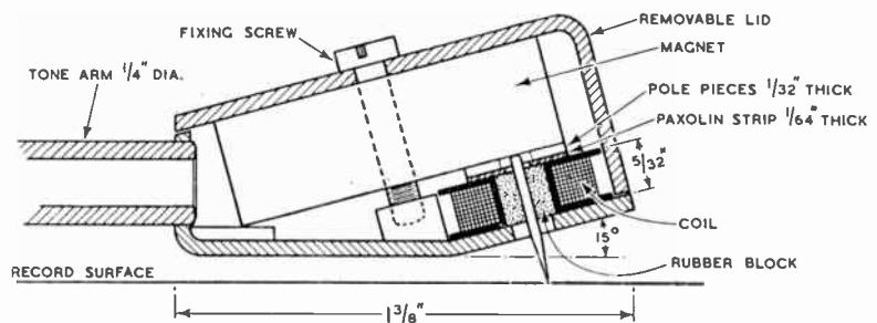
Fig. 1. Lay-out and approximate dimensions of pick-up.
