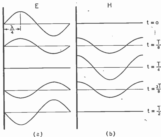
Fig. 1. Instantaneous diagrams of the way in which the amplitude of stationary waves varies with distance from a metallic reflector situated at the left-hand edge of each curve.
