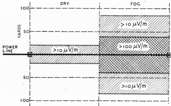
Fig. 8. Interfering field contours in dry weather and in fog at 1,000 kc/s.
