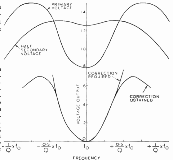
Fig. 7. Correction curve giving the voltage necessary to correct for the non-linearity of the basic frequency/output curve shown in Fig. 6. This compensation is obtained with a transformer coupling 1.5 times critical which gives the double humped response curves shown.
