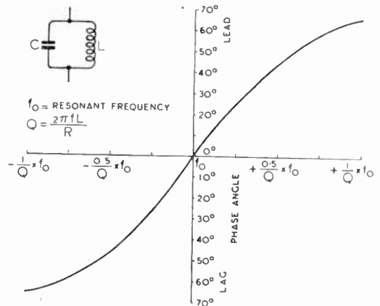
Fig. 2. Universal frequency/phase angle curve for a parallel tuned circuit. It will be noted that there is a substantially linear relation between frequency and phase, provided the band \pm 40 to \pm 45 degrees is not exceeded.
