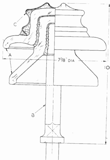
Fig. 3. 11-kV pin-type insulator with metal cap (Pilkington Bros.) A, toughened glass shells; B, steel pin; C, copper or aluminium cap.
