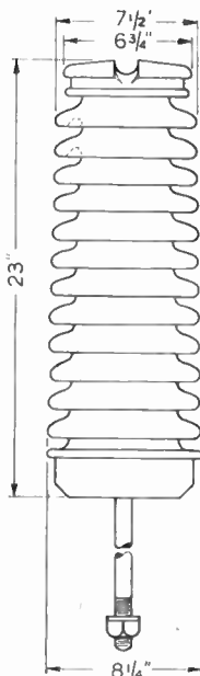
Fig. 4. Line post insulator (Lapp Insulator Company, U.S.A.)
