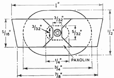
Fig. 2. Details of pole pieces and coil. The coil has approximately 3,000 turns of 47 SWG enamelled wire.
