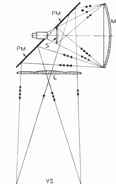
Large-screen television.
