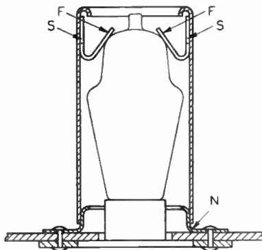
Valve location.
