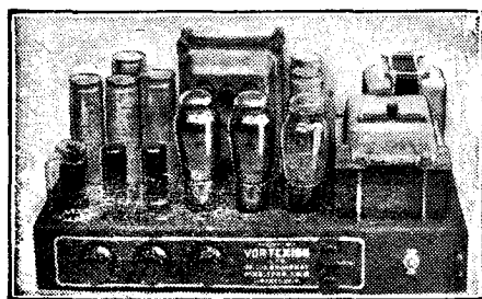
A pair of matched 6L6's with 10 per cent. negative feed-back is fitted in the output stage, and the separate HT supplies to the anode and screen have better than 4 per cent. regulation, while a separate rectifier provides bias.
