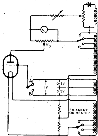
Fig. 6. Simplified circuit of a valve tester using alternating supplies to provide the working voltages for measurement of mutual conductance.
