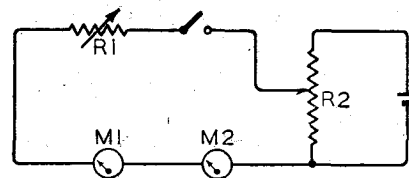
Fig. 2. Circuit for testing the movement of a milliammeter. M1 is a standard meter; M2 the meter under test. R1 provides fine control of current and R2 is the coarse control.
