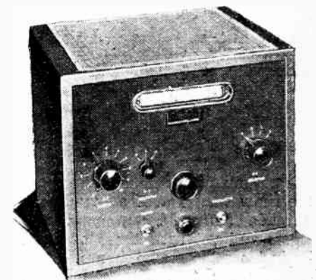
S.B. modulated oscillator in which the A.C. power pack may be used for external testing.
