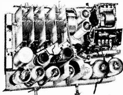
A rear view of the all-steel rubber mounted chassis, which gives some idea of its skilful design and fine engineering construction.
