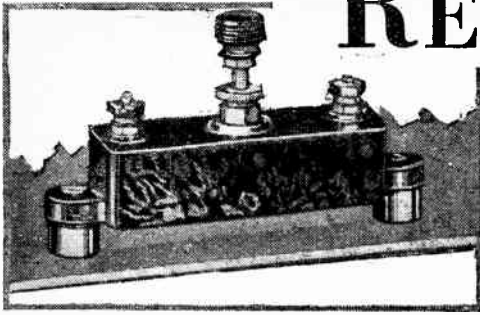
Reducing stray capacity by mounting a compression type of condenser above a metal base.
