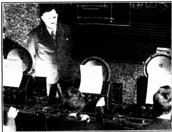
ELECTRICAL MUSIC. So high an authority as the Berlin State Academy of Music has now recognised the possibilities of the thermionic valve as a musical instrument. The photograph shows a Trautwein class under the direction of the inventor, Dr. Trautwein.
