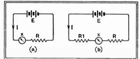
Fig. 2.—Measurement of resistance with a milliammeter and a battery of known voltage E . The circuit is shown at (a). The resistance of the milliammeter x must be allowed for. To guard against a possible short circuit in the resistance R a safety resistance R_1 should be inserted temporarily as shown at (b) and explained in the text.
