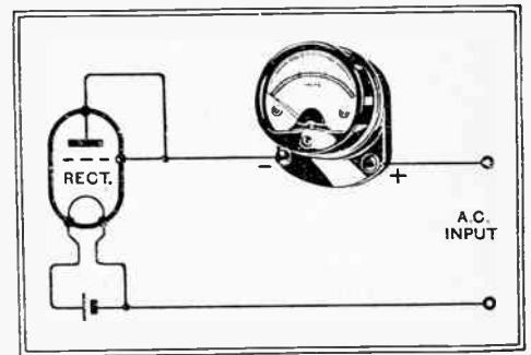
Fig. 2.—In order to read A.C. voltages on a D.C. voltmeter, a rectifier may be inserted in series.
