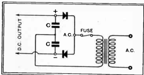
Fig. 1.—A conventional "voltage-doubling" circuit; the reservoir condensers C should be chosen with regard to the periodicity of the mains supply.
