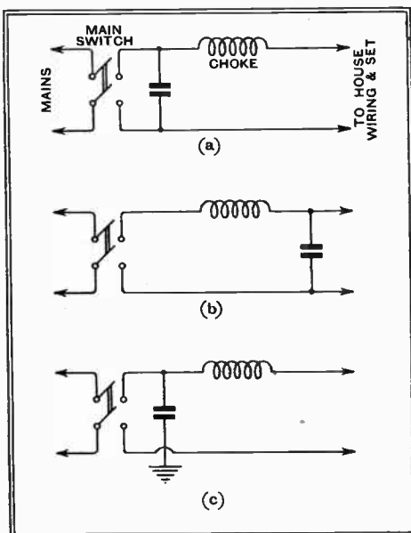
Fig. 1.—Simplified mains filters with a single choke.
