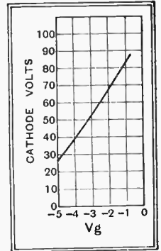
Fig. 4.—The variation in cathode potential for various grid bias voltages is shown here.
