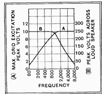
Fig. 5.—Operating conditions for a pentode derived from the curves of Fig. 4.
