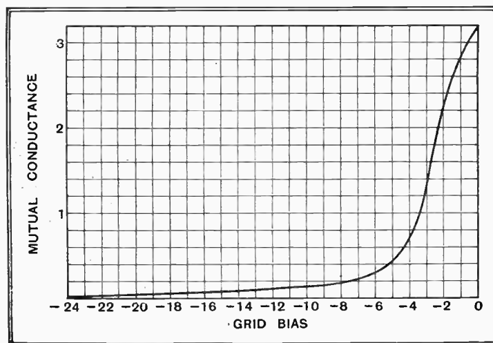
Fig. 2.—The mutual conductance of the V.P.4 valve for any bias voltage can be read off from this curve.
