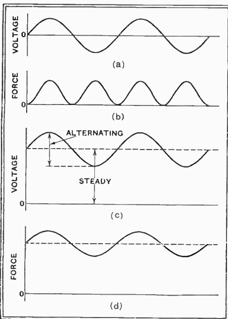
Fig. 3.—Without a polarising voltage, frequency doubling would occur in an electrostatic loud speaker.
