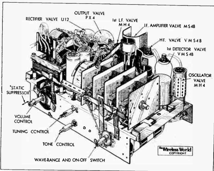
For a seven-stage circuit the chassis is remarkably compact.
