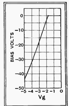
Fig. 5.—This curve shows the A.V.C. bias voltage available for various grid voltages on the MHD4
