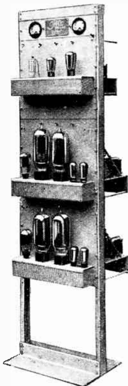
Rack-built receiver-amplifier by Tannoy.
