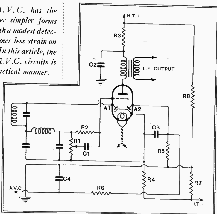
Fig. 1.—The duo-diode-triode can be connected to give delayed amplified A.V.C. The anode A2 is negatively biased in the absence of a signal and is non-conductive. With a strong signal the anode-cathode path becomes conductive and the anode assumes practically the same potential as the cathode.
