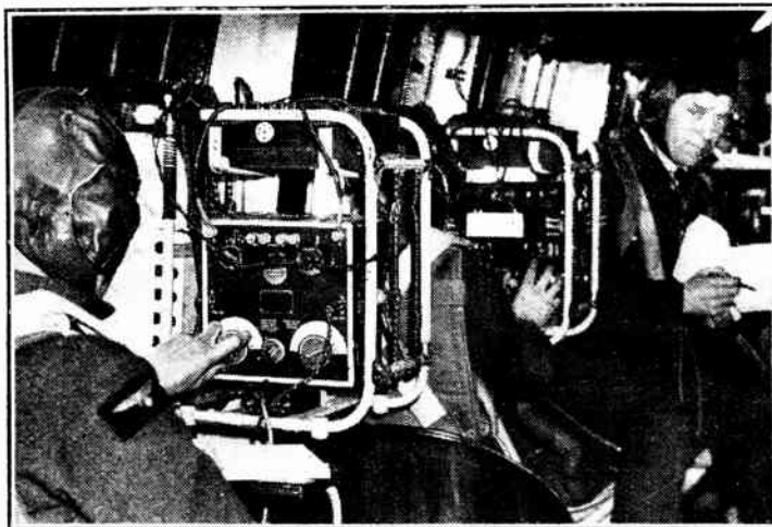
"HIGH-CLASS" RECEPTION. An aircraft cabin fitted as a classroom for the wireless instruction of R.A.F. pupils at the Electrical and Wireless School at Cranwell.
