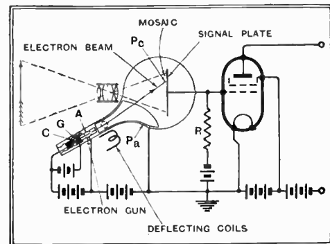
Fig. 1.—Elements of the Iconoscope device.
