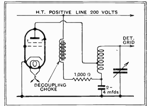
Fig. 2.—Reducing voltage loss: decoupling for a tuned-anode H.F. stage.
