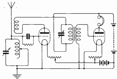
Circuit Diagram of Mr. Baldry's Set.
