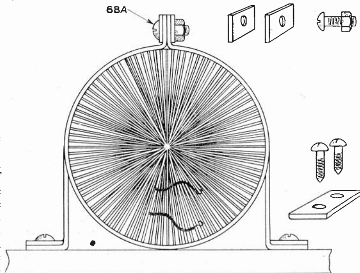
Fig. 4. End view of Transformer when mounted.
