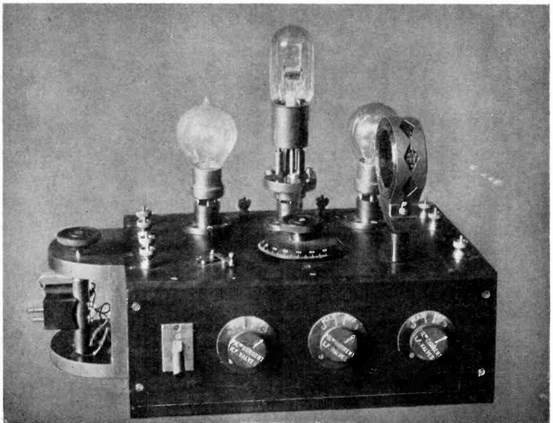
Fig. 1. The complete instrument.
