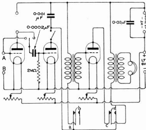
Fig. 3. Simplified circuit diagram.
