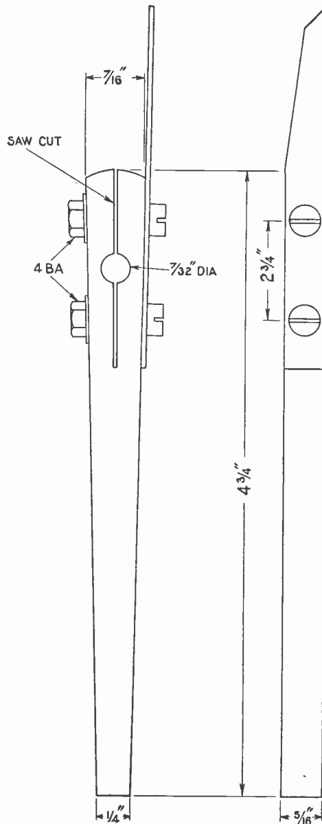
Fig. 4. Handle and Pointer.
