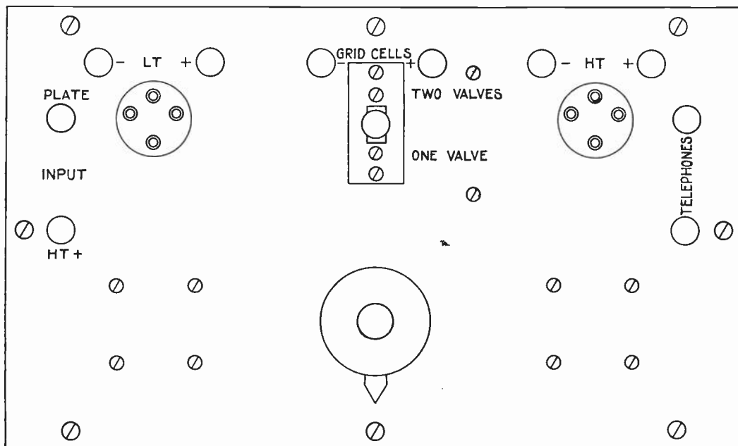
Fig. 2. The lay-out of the panel.
