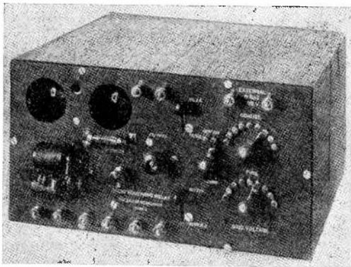
Fig. 4. Type A Relay Recorder for use with Batteries.
