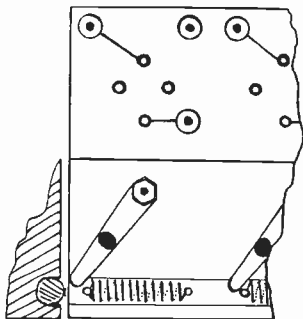
Fig. 6. Valve panel mounting.
