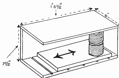
Fig. 3. The box in which coils are mounted.
