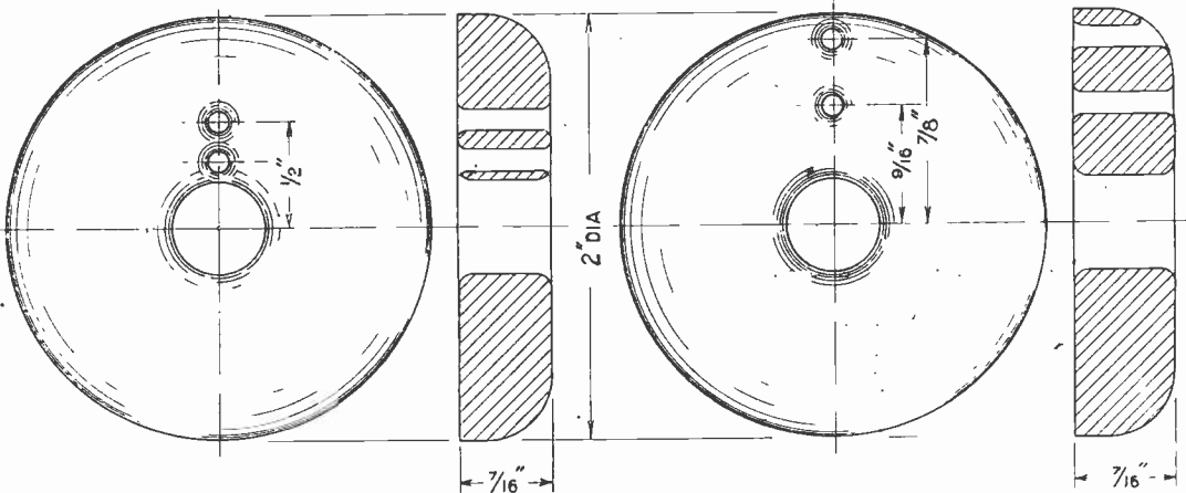
Fig. 1. Ebonite end plates with rounded corners.
