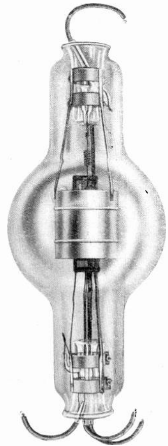
Type T250. Requires an Anode Voltage of 2,000, and dissipates \frac{1}{4} -kW. Overall length 280 mm.
