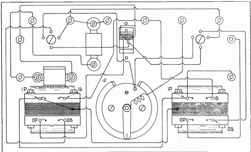
Fig. 3. Wiring of the instrument.
