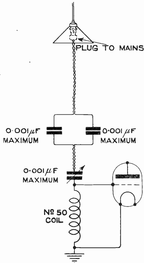
Diagram, showing Circuit.
