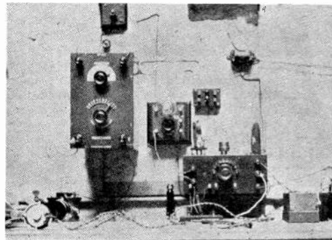
Eastbourne College Receiving Set.
