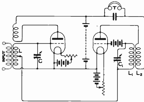
Fig. 4. A practical two-valve circuit.
