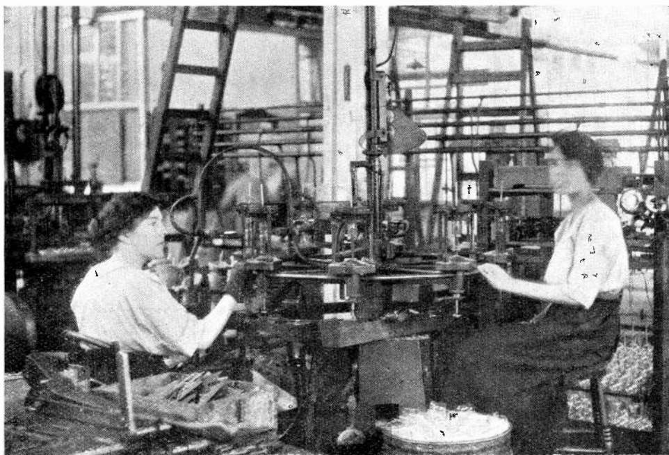
Machine for sealing in the mounted electrodes.
