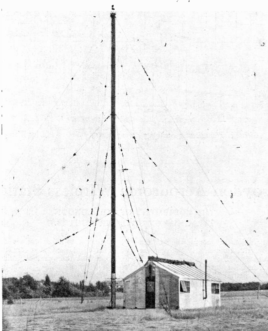
Fig. 1. The Mast carrying the D.F. Aerials.
