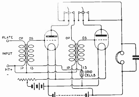
Fig. 4. The Circuit diagram.
