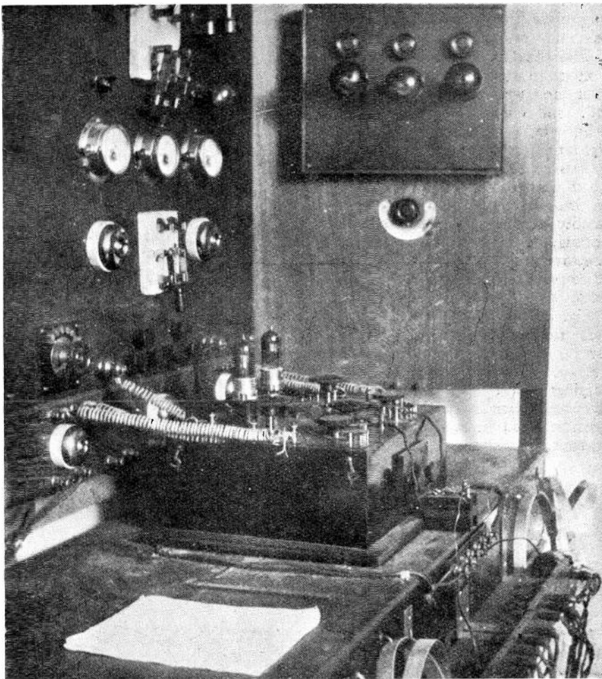
The complete Receiver, showing Plugs and Jacks.
