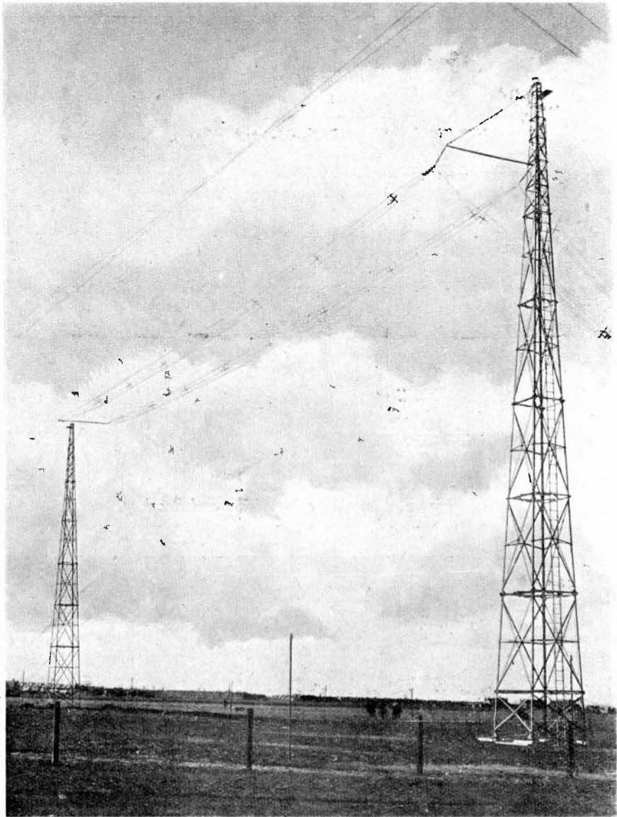
Fig. 4. The Aerial and Mast of the Transmitter.
