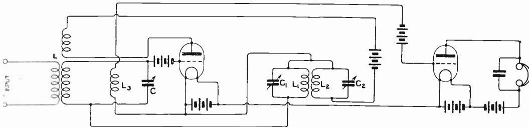
Fig. 3. A combination of the methods shown Figs. 1 and 2.
