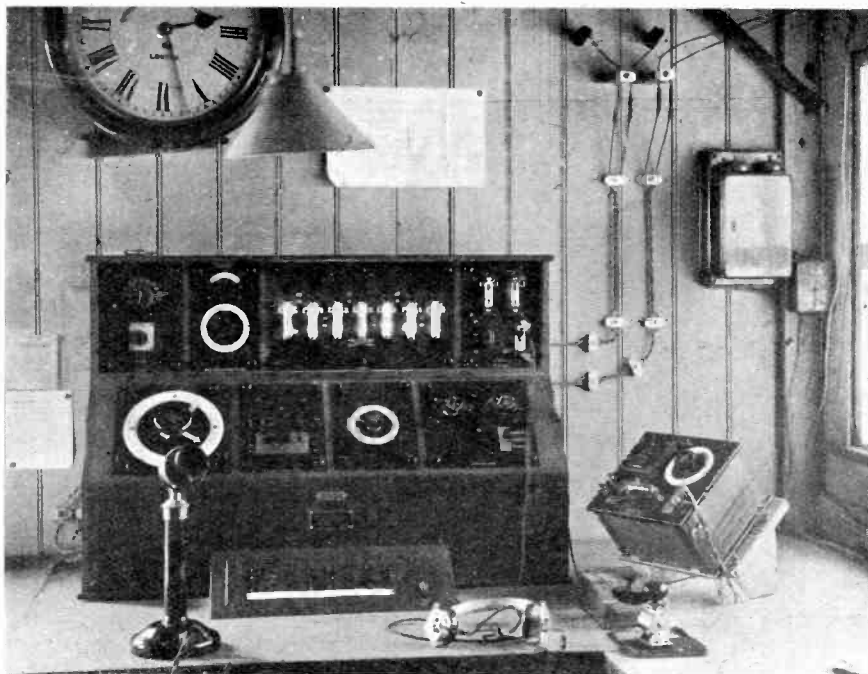
Fig. 2. The Direction Finder and Receiver.
