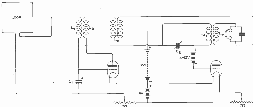
Diagram of the Armstrong Super-regenerative Circuit referred to above.
