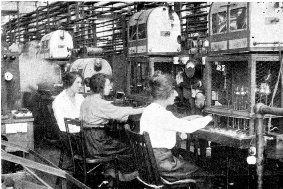
Valves of the "R" type connected to the pump whilst the operator controls the potentials applied to the electrodes.
