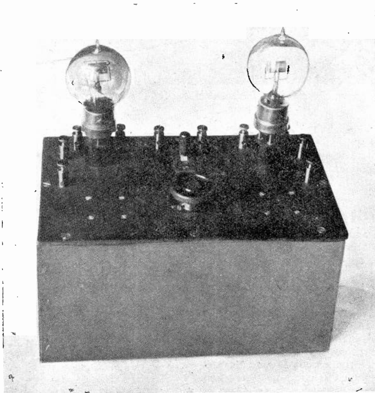
Fig. 1. Photograph of the two-valve amplifier.
