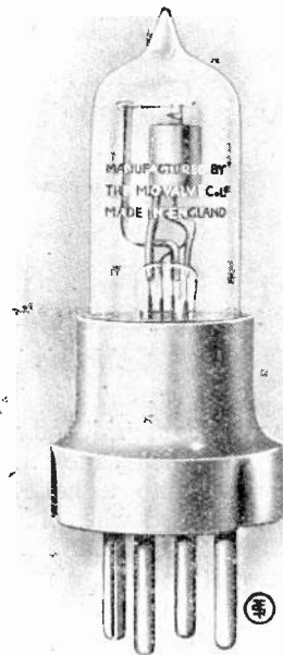
Low Temperature Emitter, Type L.T.3. Requires a filament potential of only 1.8 volts and passes a current of 0.11 amperes. An efficient detector, oscillator, high and low frequency amplifier.
