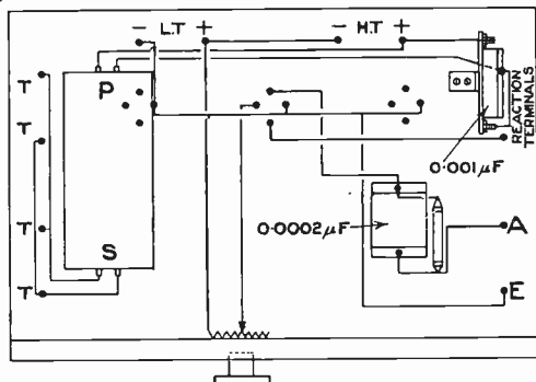
Fig. 2b. Single valve wiring diagram.
