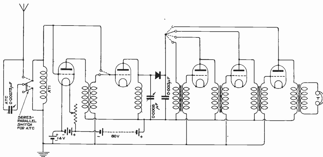
Fig. 8. Circuit diagram.
