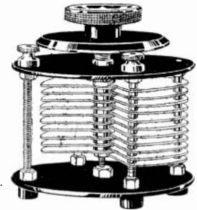
“LESMAC.” CONDENSER
