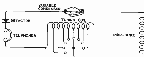
Fig. 2. Receiving Circuit with Variable Condenser and Auxiliary Tuning Coil.
