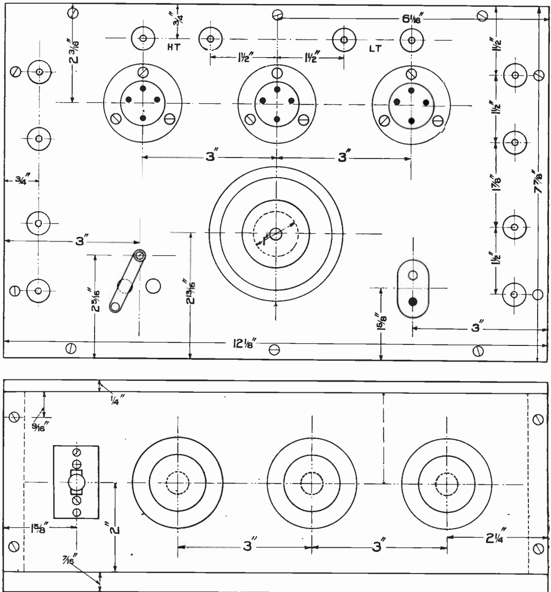
Fig. 4. Dimensions of the panels (top and front).
