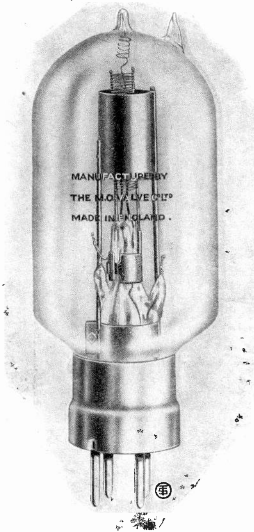
Type T30. A low power Transmitting Valve dissipating 30 watts.
