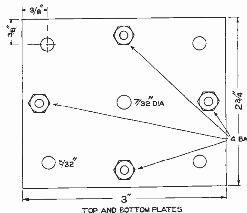
Fig. 1. Ebonite end plates, Thickness \frac{3}{8} ". Three of the nuts are on the rods carrying the plates and the other holds the steadying rod.
