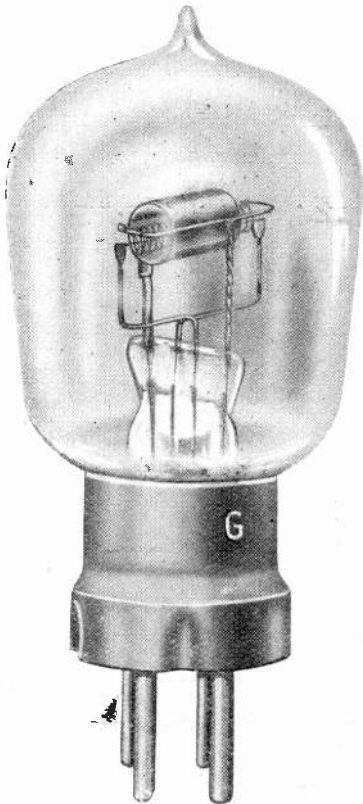
Detector Valve, Type R.A.B. Filament volts 3.8, filament amps. 0.65. Normal anode volts, 50/70. Designed for use as a detector or low frequency amplifier.
