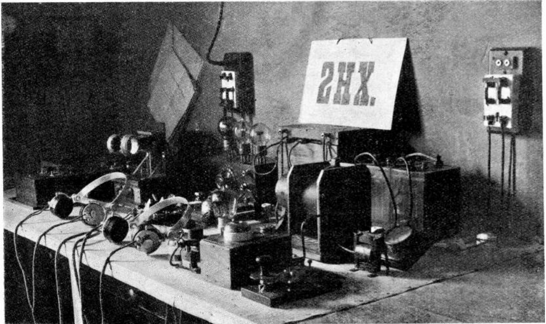
2 HX, an Amateur Station at Guildford.
