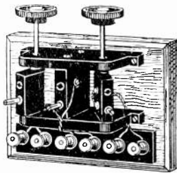
TUNING STANDS on Polished Mahogany base, 22/6. Supplied less Terminal Board & base, 19/- Long Tuning Handles supplied if desired, same price.
