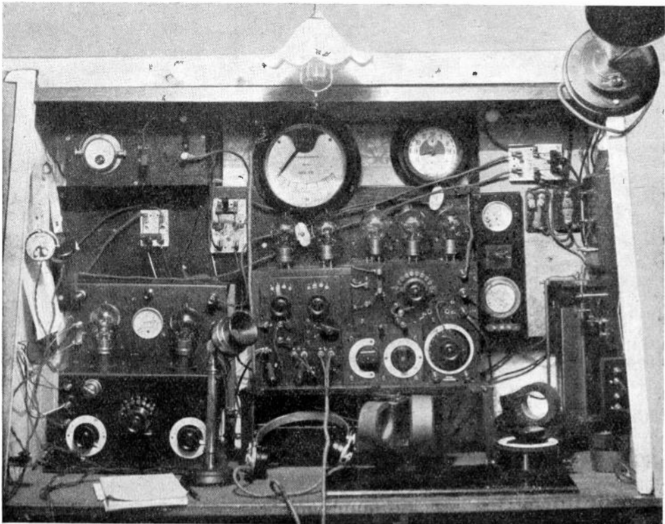
Fig. 1. The Receiving and Transmitting set of 2 KU
