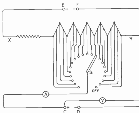
Fig. 2. General arrangement of a Shunt Switchboard
