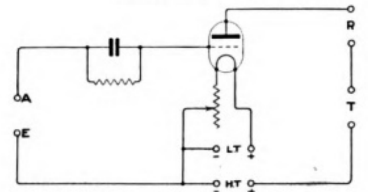
Circuit drawn in the form usually adopted in wireless circuit diagrams. The condenser across the telephone terminals is omitted.
