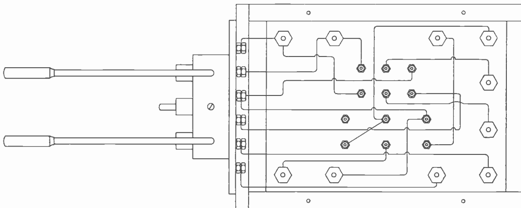
Fig. 4. Under side of panel to show wiring.
