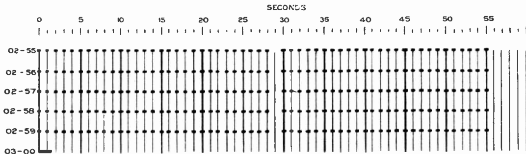
Fig. 2. American Time Signal System.
