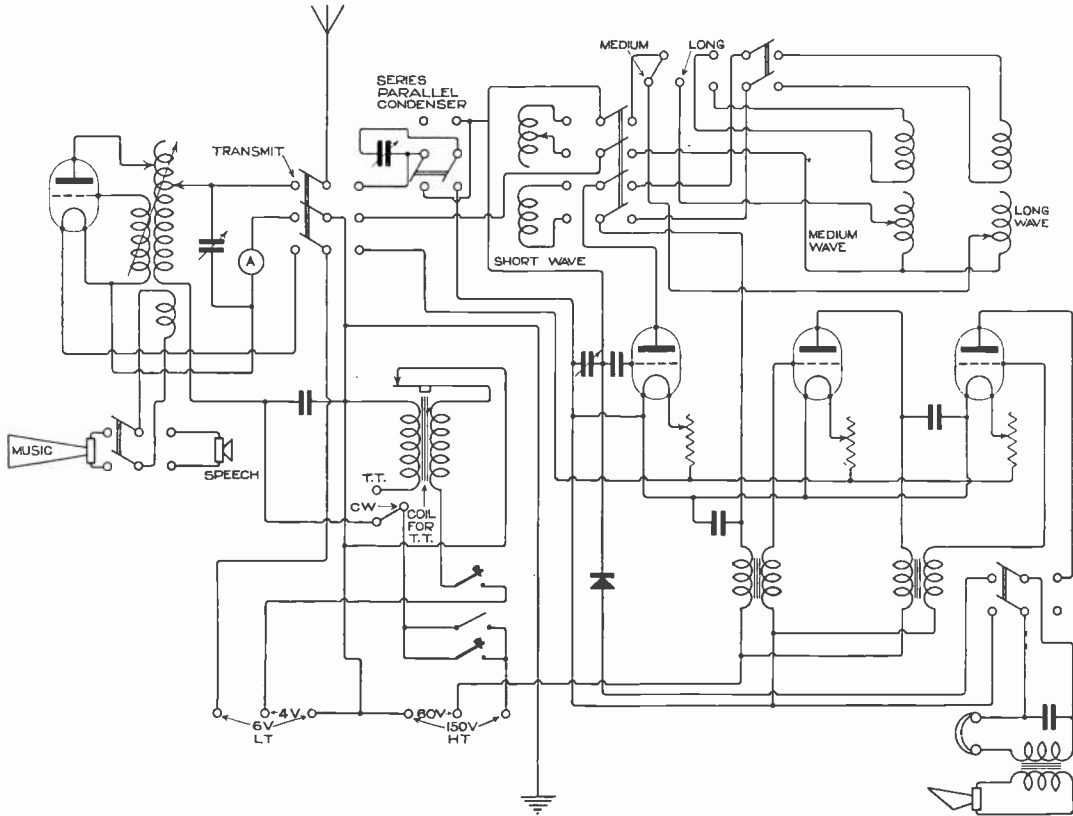
Fig. 2. Circuit diagram of 2 UV.
