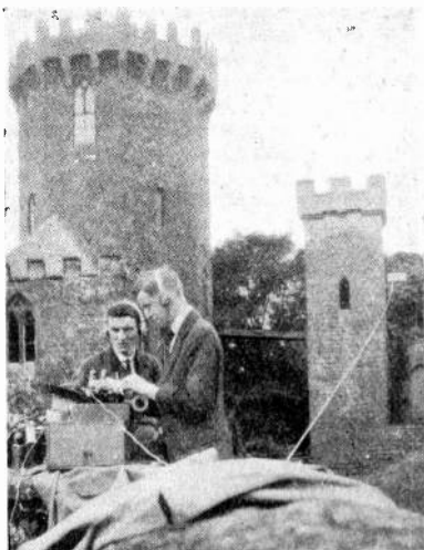
Portable Set used by Warwick School Society. The aerial is seen attached to the tower in rear.
