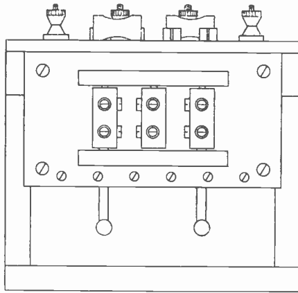
Fig. 3. End view showing three-coil holder.
