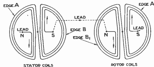
Fig. 6. Showing the connections of the Coils in the Variometers.
