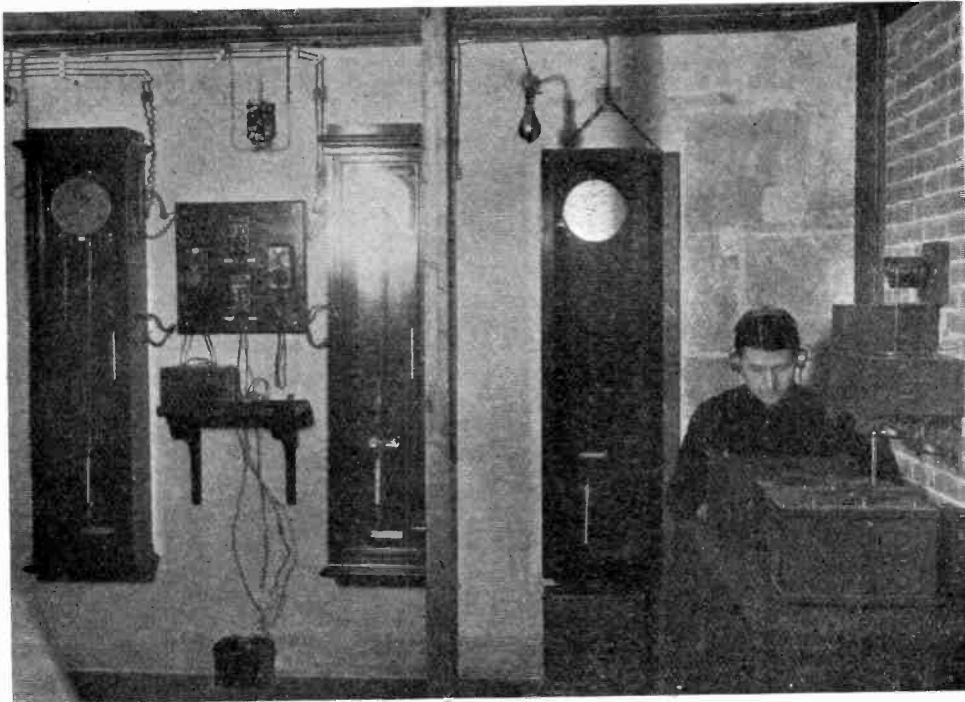
Fig 8. After adjusting the pendula the lag due to the automatic transmission apparatus interposed between the pendulum and the aerial is measured before the time signal is sent out.
