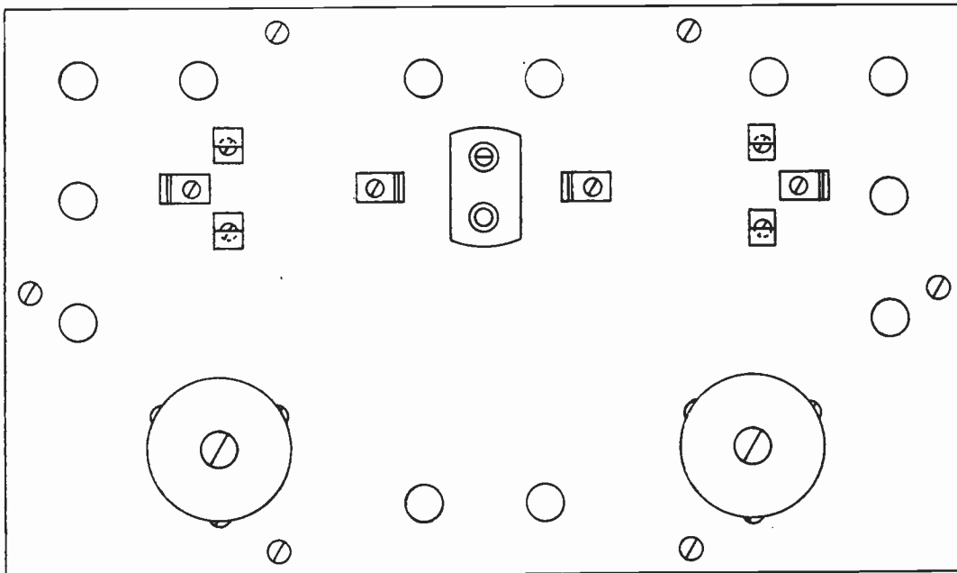
Fig. 2. Layout of Panel. Terminals on the left are for "Input." [On the top row they are for reaction, reactance condenser, and H.T. respectively; the pair on the right side being for L.T., and those at the front for telephones or note magnifier unit.
