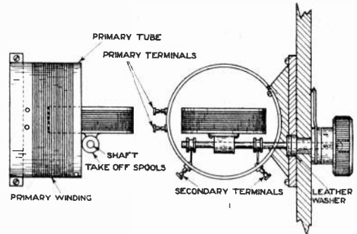
Fig. 2. The Loose-coupler, showing constructional details.
