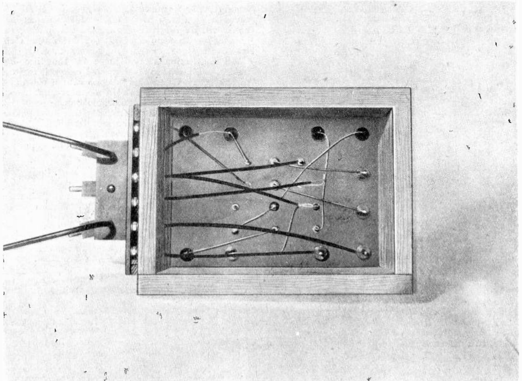
Fig. 5. A photograph of the under side of the tuner, with bottom of box removed.
