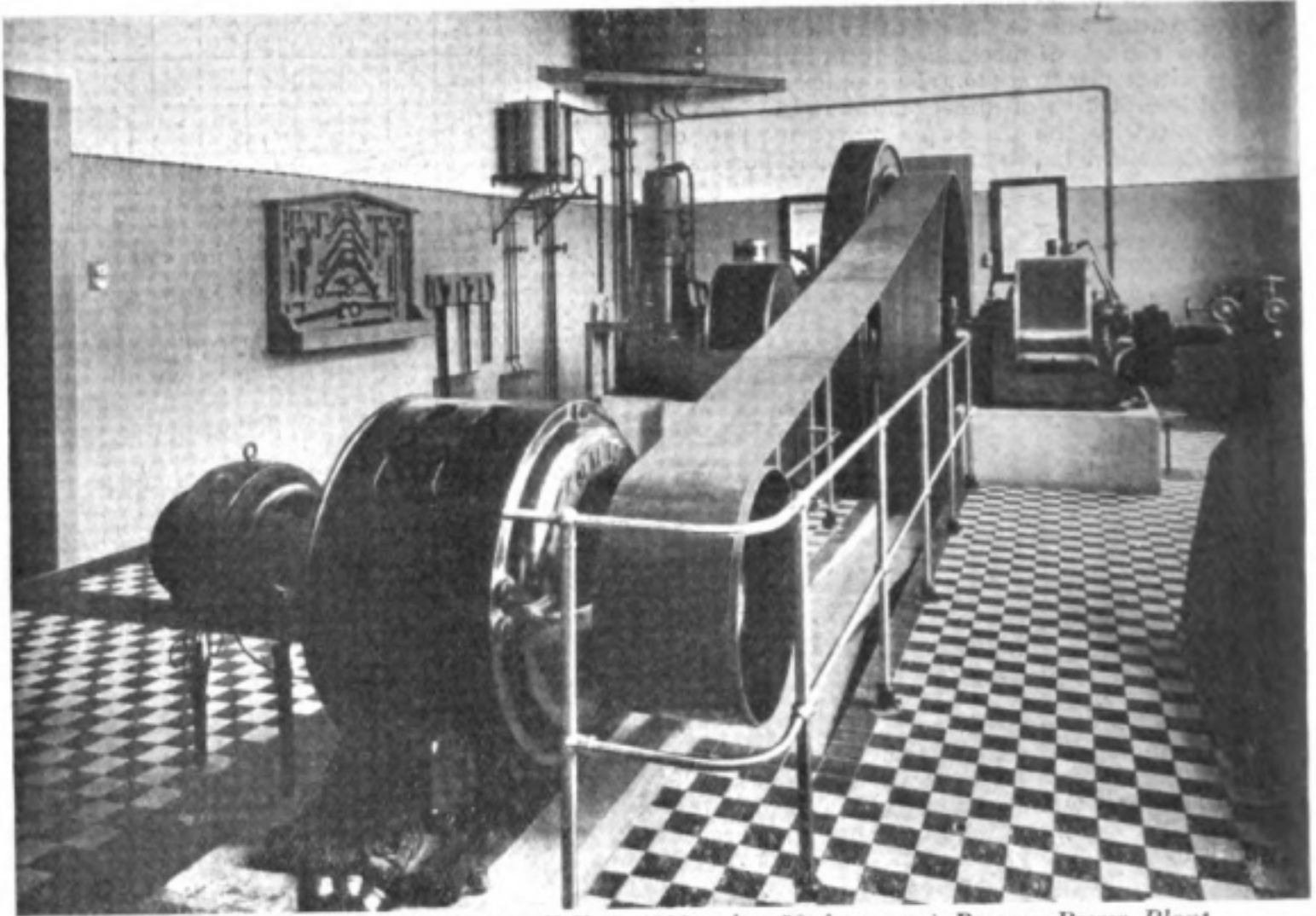
Fig. 7. Engine Room shewing 50 K.V.A. (500 volts, 50 frequency) Reserve Power Plant.
