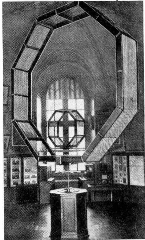
Installation at the Paris Observatory for the comparison of Time Signals received from Eiffel Tower, Lyons, Bordeaux, Annapolis, Nauen and other stations with the pendulum of the Observatory clock. Signals received on the frame aerial shown in the photograph are thus compared by aural methods and by self-registering apparatus shown near the window.
