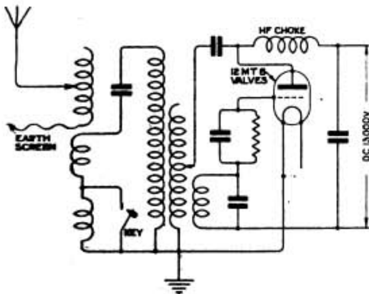
Fig. 4. The Aerial Circuit showing signalling arrangement and also the Oscillator Valve Circuit.
