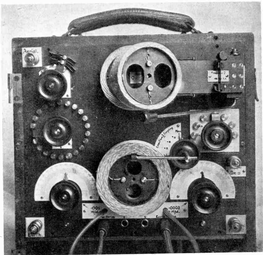
Fig. 3. General Arrangement.
