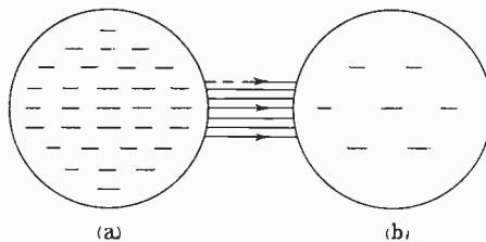
Fig. 3. Represents two atoms (a) possessing a negative charge or surplus of electrons. (b) possessing a positive charge or deficiency of electrons; if brought near together, electrons fly across to the atom with the positive charge.
