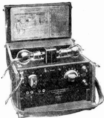
B. Mark II. Detector Amplifier Set. Price (less valves), £6 5 0. Price with Variable Condenser included, £7 5 0.
