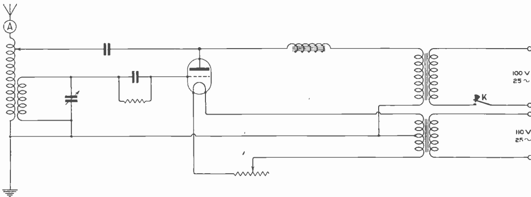
Fig. 4. The final circuit used.
