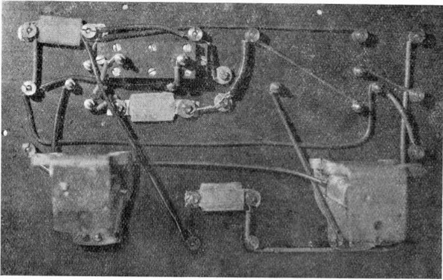
Fig. 3. The underside of the panel, showing the wiring connections.
