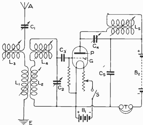
Fig. 1. Circuit diagram of Receiver.
