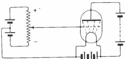
Fig. 6. Valve circuit with grid connected to the centre of the potentiometer and so having no charge on it. The grid here does not interfere with the normal flow of electrons.
