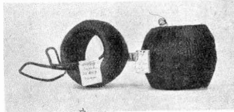
Fig. 2.—H.F. Auto-transformers. Left: 2,000 turns 28 S.W.G. enamelled copper. Right: 2,000 turns 26 S.W.G. enamelled copper. Internal diameter 2 1/4".
