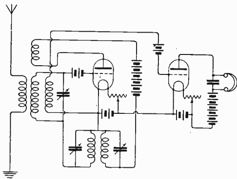
Fig. 3. The Super-Regenerative Circuit, by means of which both negative and positive resistance is acted upon. The second valve acts merely as a detector.
