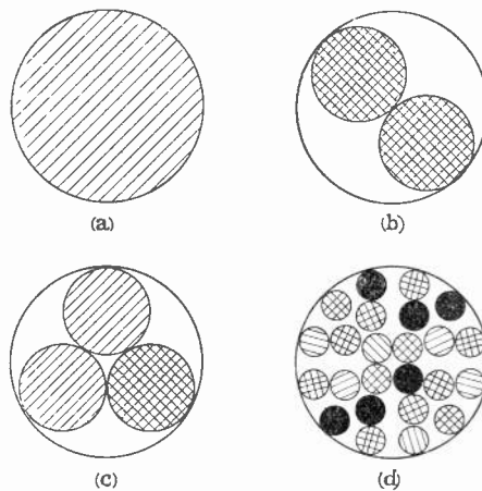
Fig. 1. Diagrammatical representation of (a) A molecule of Hydrogen consisting of one atom. (b) A molecule of Oxygen consisting of two atoms. (c) A molecule of Water consisting of two atoms of Hydrogen and one of Oxygen. (d) A molecule of Sugar consisting of six atoms of Carbon, twelve atoms of Hydrogen and six atoms of Oxygen.
