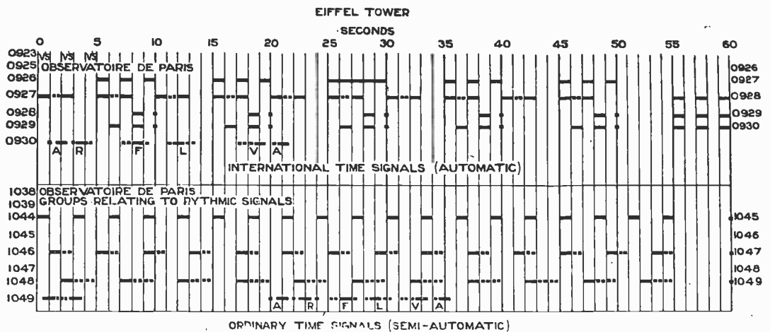
Fig. 3. Method of transmitting time signals from Eiffel Tower.
