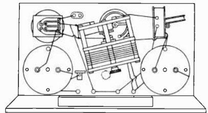
Fig. 3. Rear view of the set. The secondary variometer and condenser are mounted at right angles to those in the other circuits.
