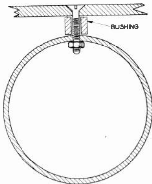
Fig. 6. One end of the inductance former.
