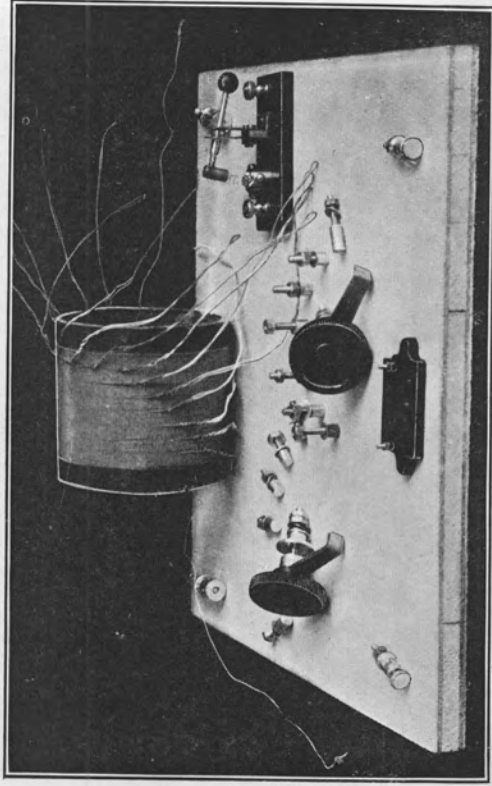
FIG. 18.—PARTS OF RECEIVING SET ROUGHLY ASSEMBLED READY FOR FIXING
