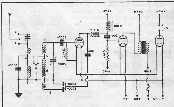
The theoretical circuit of the Telsen "Conqueror" 3.
