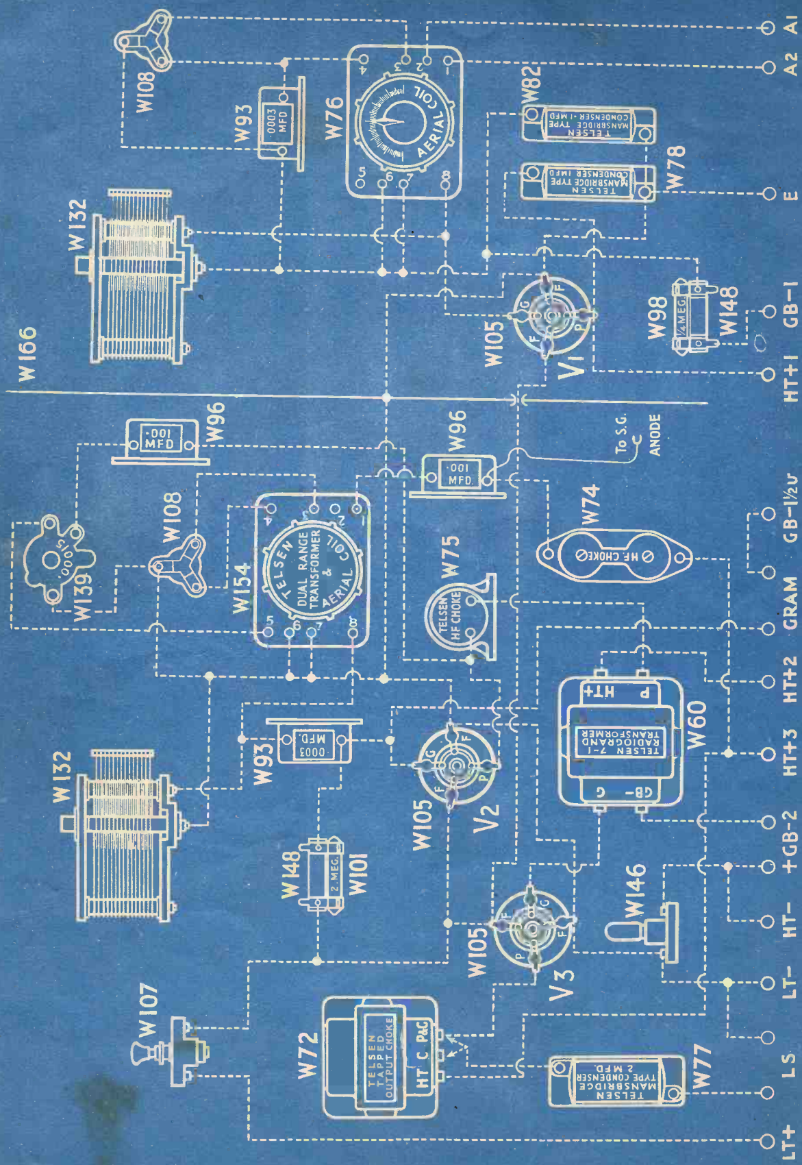
WIRING DIAGRAM
