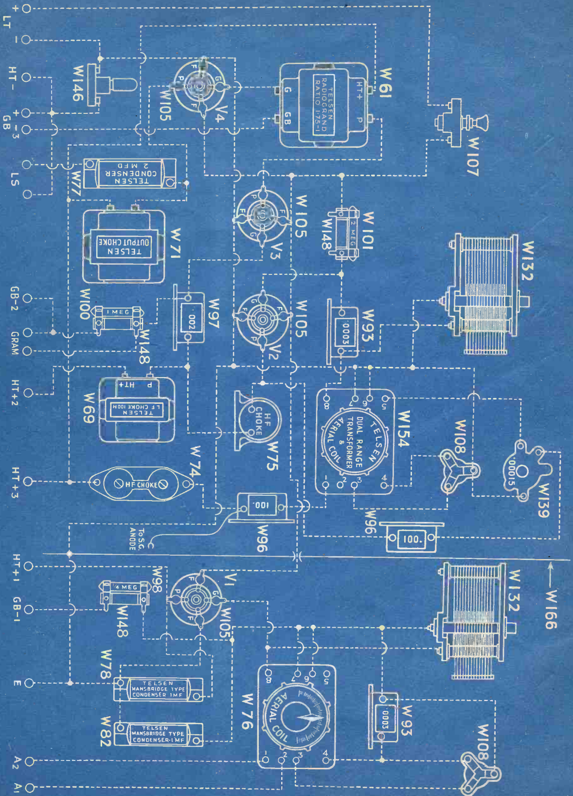
WIRING DIAGRAM
