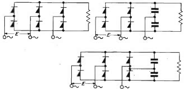
Fig. 3(a). Three-phase bridge rectifiers Fig. 3(b). Three-phase voltage-doubler rectifier Fig. 3(c). Three-phase bridge-doubler rectifiers
