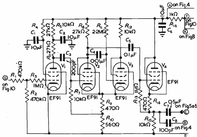
Fig. 3. Trigger generator
