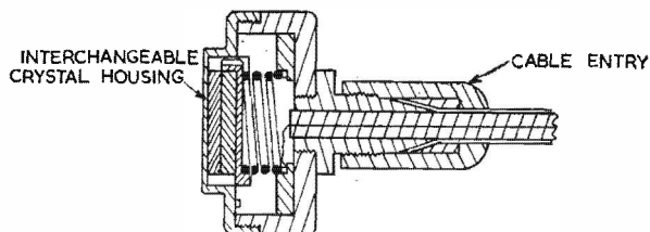
Fig. 11. Transducer with 200kc/s quartz crystal assembly
