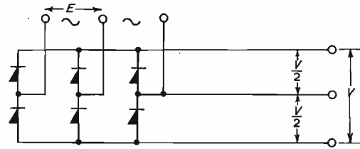
Fig. 6. Emergency method of obtaining half-voltage from three-phase bridge rectifier when supply neutral is not obtainable
