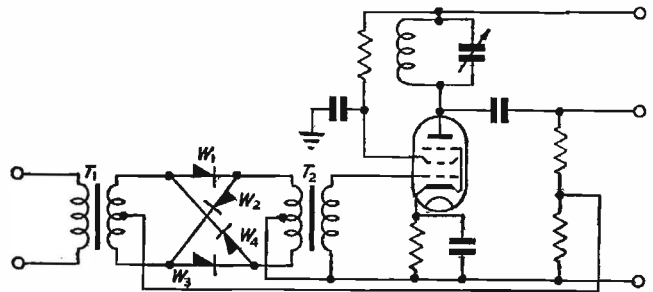
Fig. 1. Balanced-modulator divider
