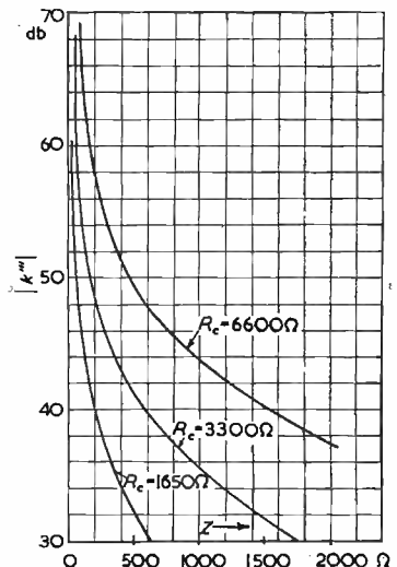
Fig. 9. Effect of Introduction of Common H.T. Impedance when
