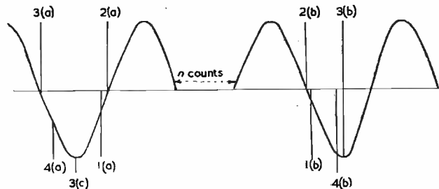
Fig. 3. The switching error
