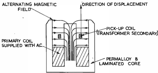
Fig. 1. The Principle of Operation. The voltage induced in the pick-up coil varies with its displacement
