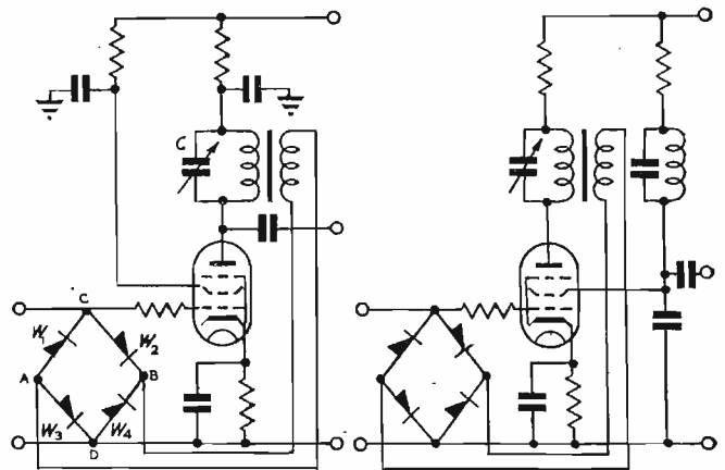
Fig. 3. New single valve divider
