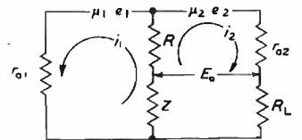
Fig. 8. Equivalent circuit with common H.T. impedance
