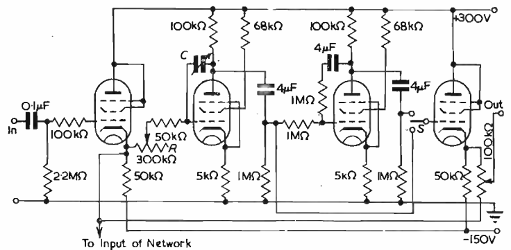
Fig. 5. Complete circuit diagram
