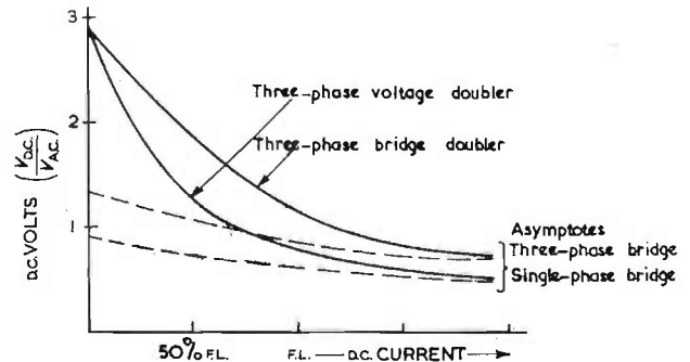
Fig. 4. Comparative regulation curves of various three-phase rectifier arrangements
