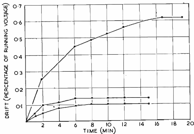
Fig. 11. Curves showing typical initial drifts of CV188 glow-discharge tubes
