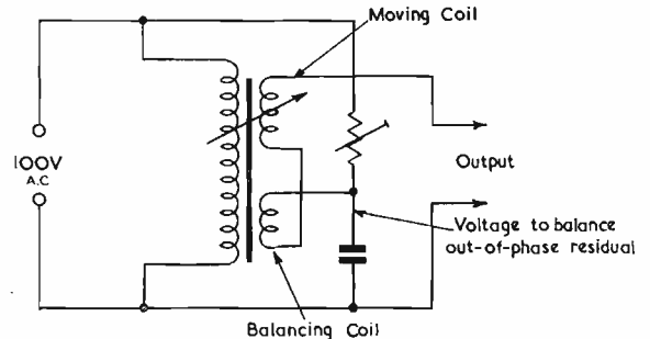
Fig. 5. Arrangement to give a balanced output, allowing the use of amplification to increase the sensitivity
