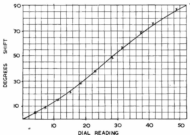
Fig. 4. Relation between dial reading and phase-angle
