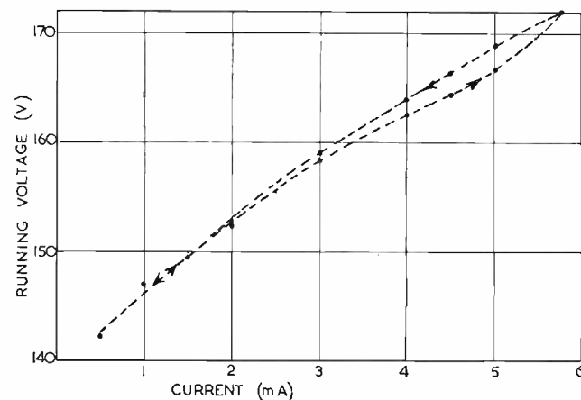
Fig. 5. Typical current-voltage characteristics of glow-discharge voltage-regulator tube type CV71 for increasing and decreasing currents
