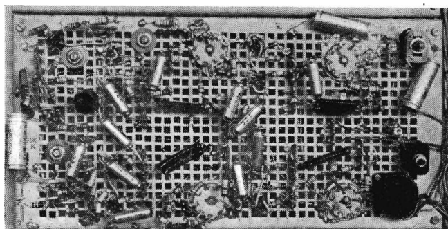
A close-up view of a chassis, illustrating the method of construction
