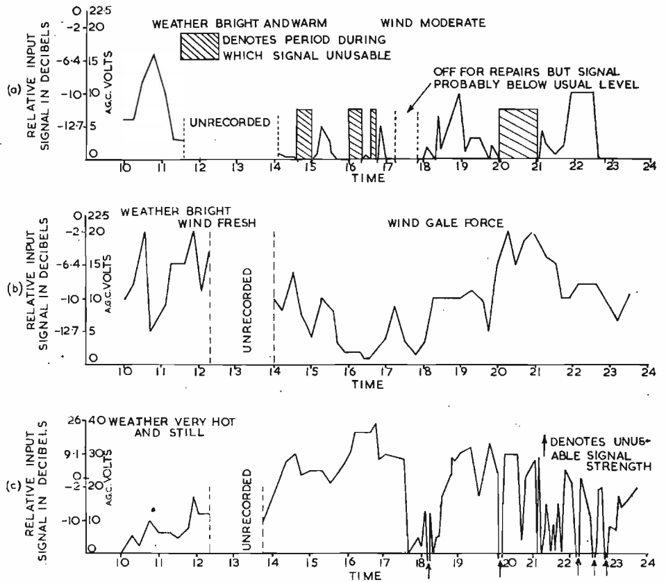
Fig. 2. Field Strength on Alembon-Swingate Link (a) July 9, 1952. (b) July 8, 1952. (c) July 1, 1952.
