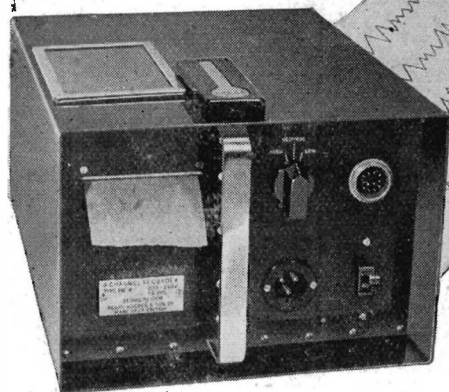
The equipment comprises three Units. The Oscillators and Power Supply Unit, the Bridge and Amplifier Unit, and that shown, the Recording Unit.
