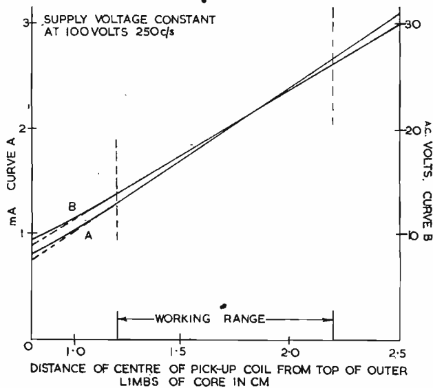
Fig. 4. Calibration curves
