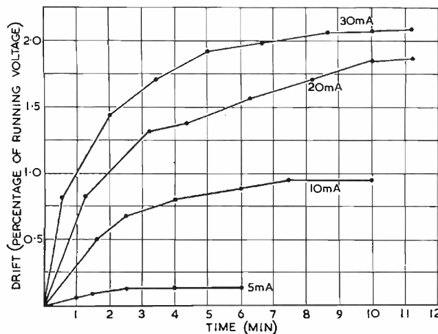
Fig. 13. Curves showing the initial drifts of a typical G120/1B glow-discharge tube at various currents
