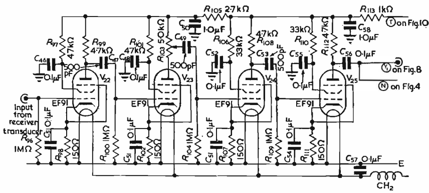
Fig. 7. Receiver amplifier
