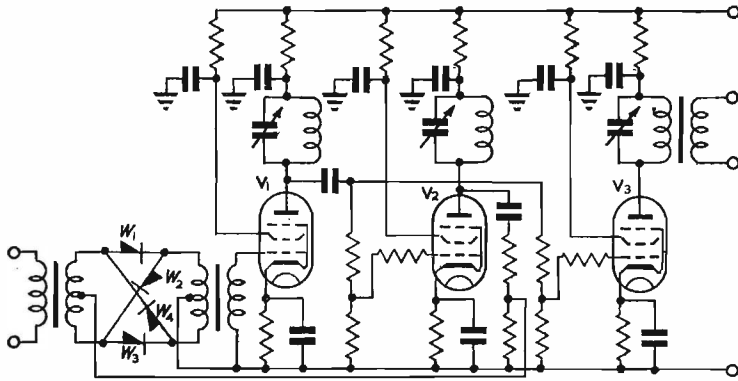
Fig. 2. Divider for ratios greater than 2 : 1
