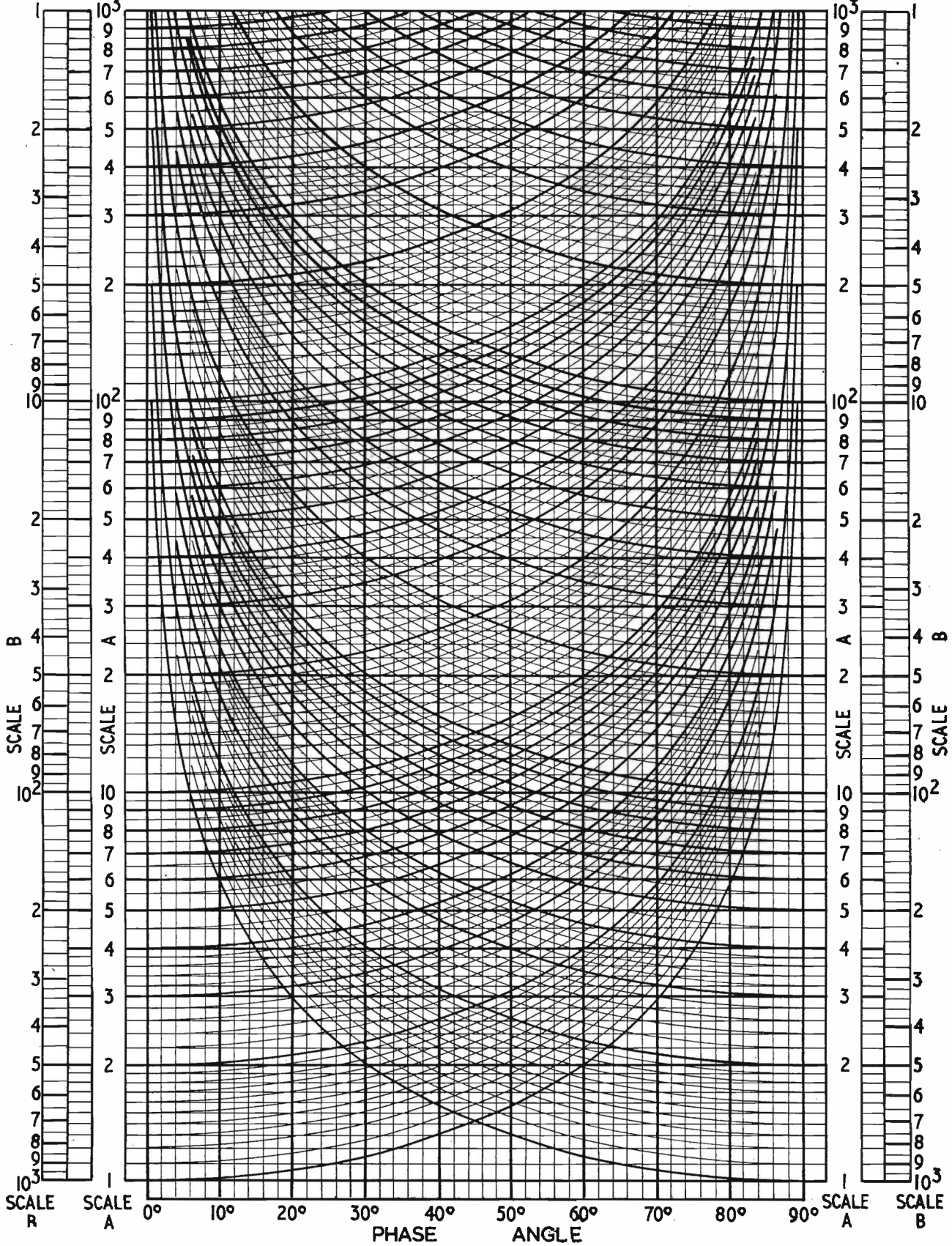
Chart for the resolution of complex quantities
