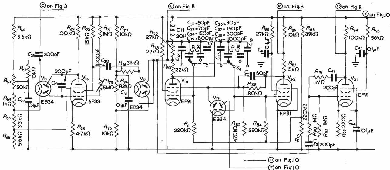
Fig. 6. Delayed time-base sweep generator
