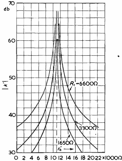
Fig. 6. Effect of Variations of r_{a1} when E_2/E_1 = \gamma/a
