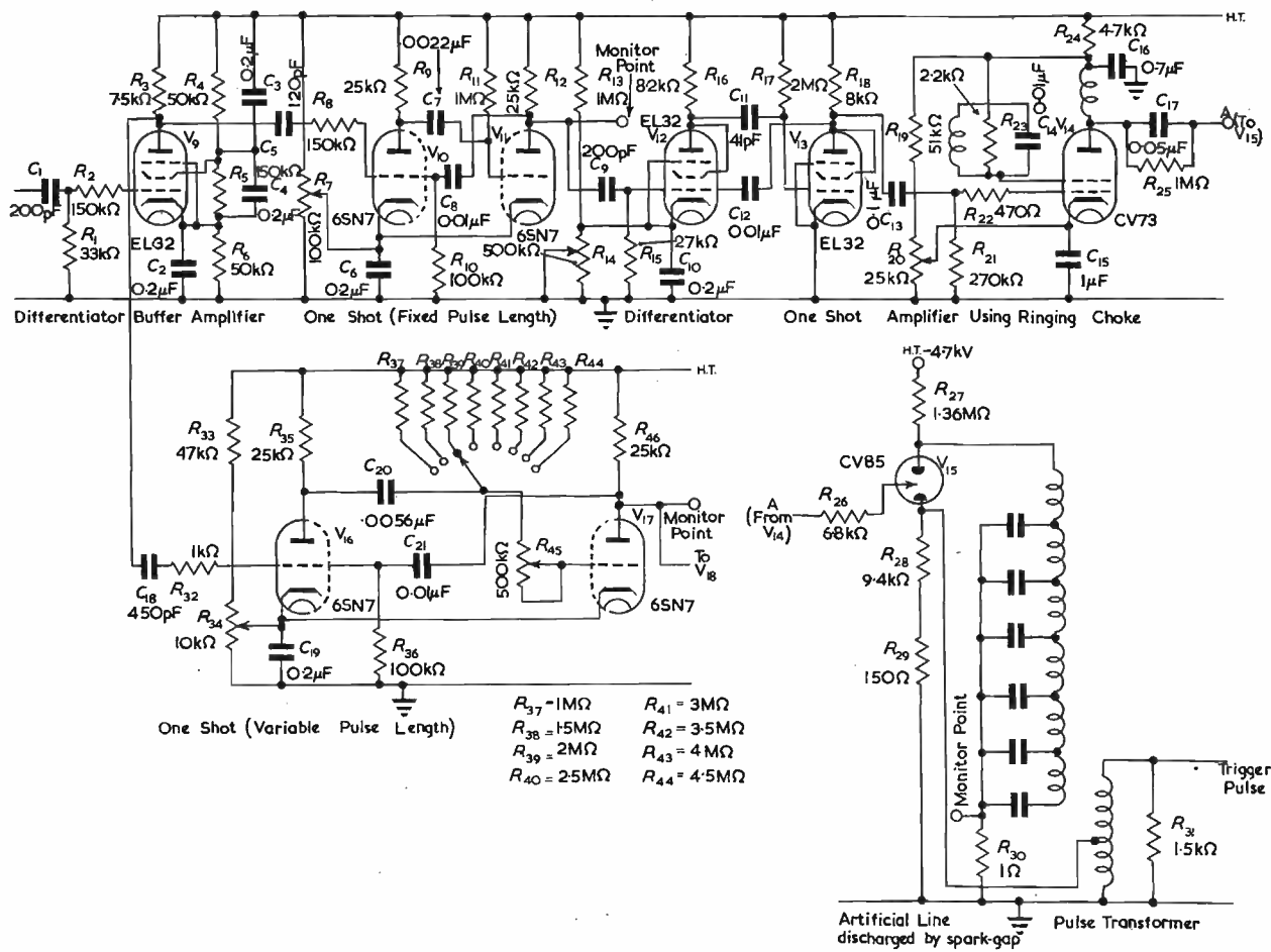
Fig. 3. The timing circuit—section 2 The circuit of V 18 to V 21 is identical to that of V 12 to V 15
