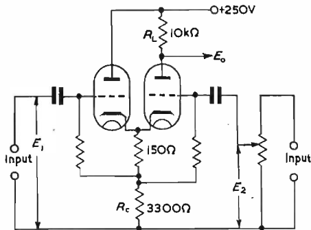
Fig. 4. Typical circuit arrangement
