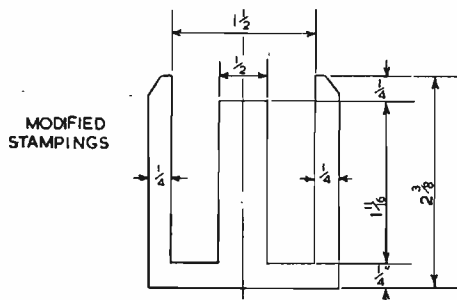
Fig. 2. Dimensions of the Component parts of the Pick-up
