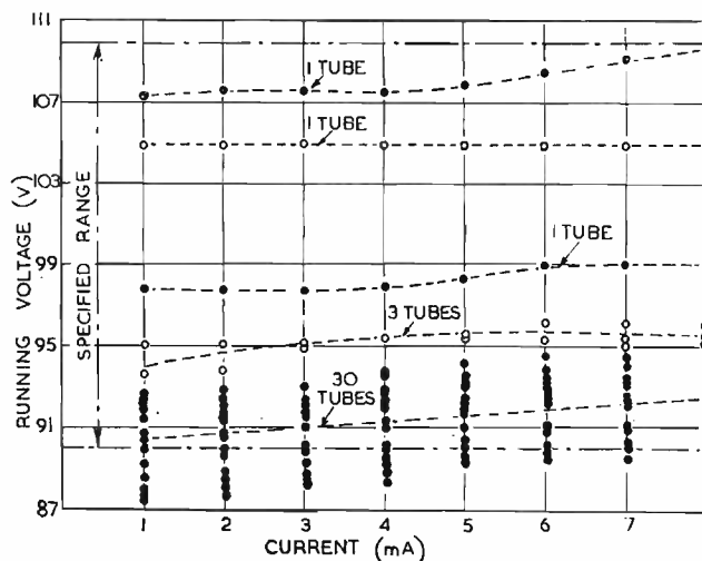
Fig. 1. Current-voltage characteristics of glow-discharge voltage-regulator tubes, type CV1070
