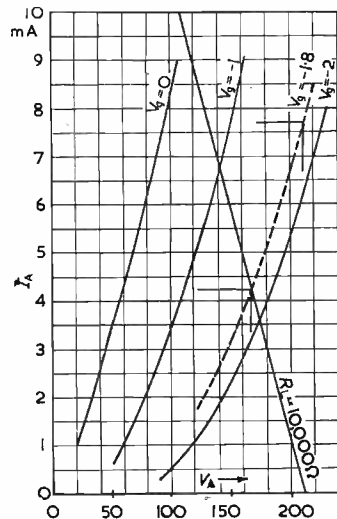
Fig. 5. Characteristics of the 12AT7
