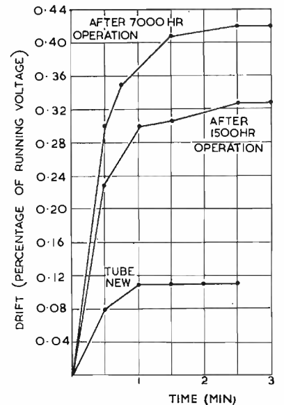
Fig. 14. Curves showing the initial drifts of a typical 85A1 glow-discharge tube at various stages throughout its life
