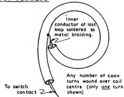
Fig. 3. Detail of the screened links, which in this application are Faraday shields, based upon an idea by G2HJT in the January 1956 issue of "Short Wave Magazine." This method adapts standard coax cable for the purpose of constructing the screened link.
