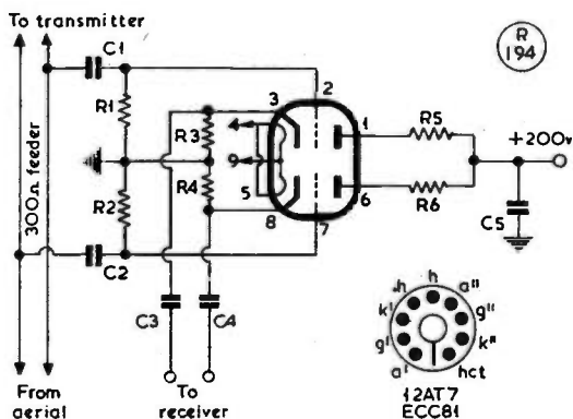
Fig. 2. A TR switch for VHF, when 300-ohm balanced feeders are used. Values are given in the table. Good results are claimed for this circuit.
