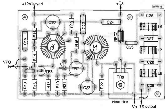
Fig. 2.2a: Component overlay of the power amplifier
