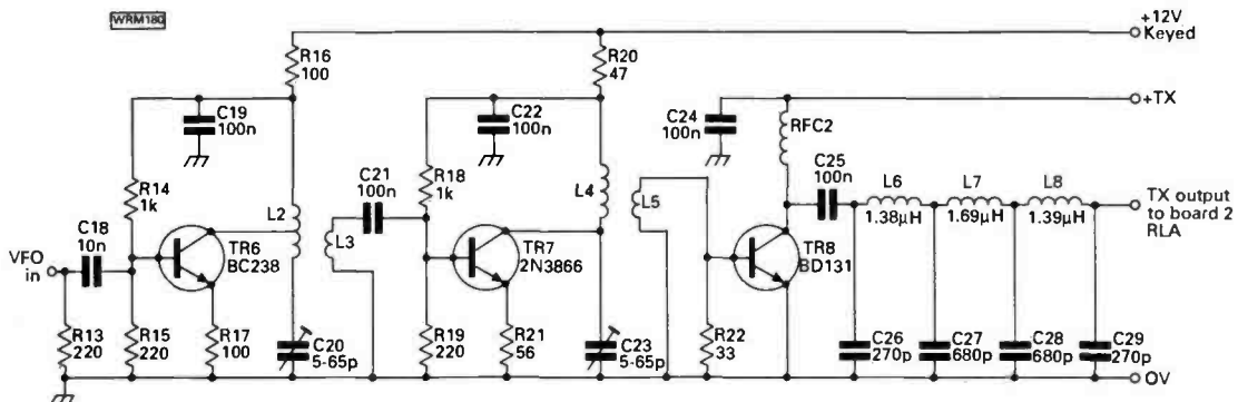
Fig. 2.1: Circuit diagram of the PW Irwell power amplifier
