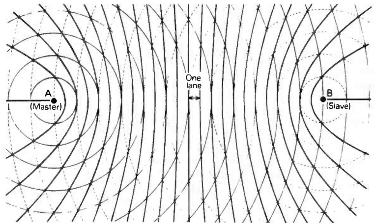
Fig.2 Position-line pattern generated by synchronised c.w. transmissions
