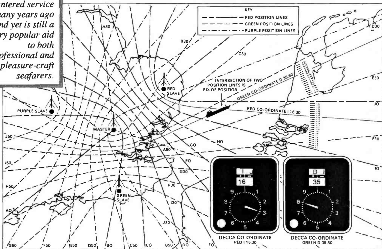
The layout of the English chain showing how a fix is obtained from the readings of the two decometer indicators
