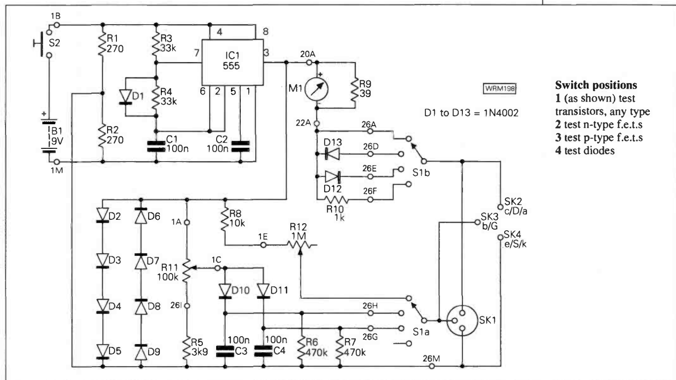
Fig. 1: Circuit diagram of the unit, simple yet belying its capabilities
