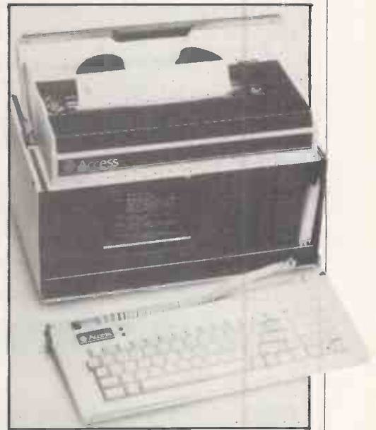
Typical of the modern American portable, the Access has built-in Modem with both acoustic and direct plug-in connection to the phone system, a built-in printer, discs and 7in. amber screen, all contained in a hefty 33lb. package.
