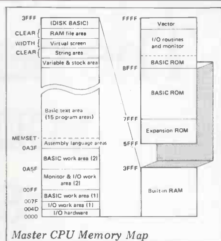
Master CPU Memory Map
