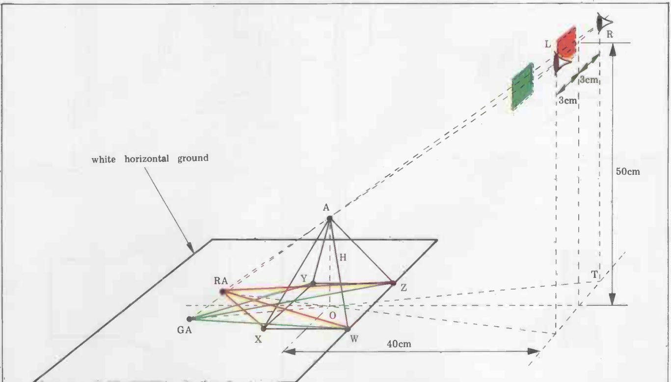
Fig 1. Basic geometry to produce red and green images on a horizontal page or VDU screen.
