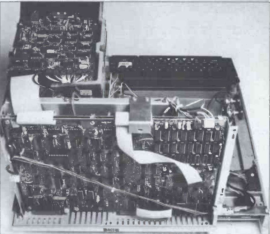
Two inside views of the Model III
