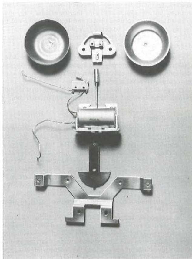
FIG. 13—Exploded view of bell unit
