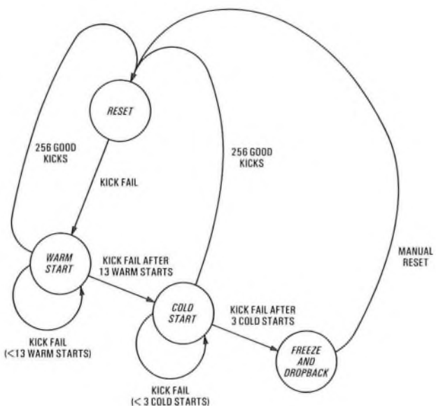
FIG. 7—Simplified diagram of the operation of watchdog
