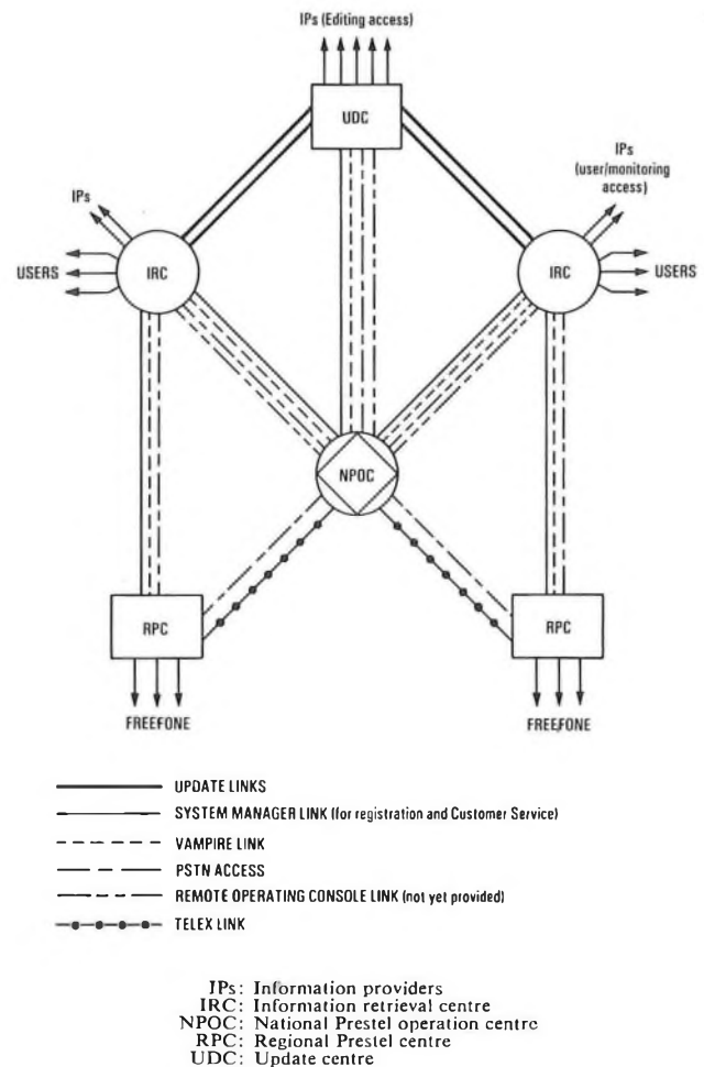
FIG. 5—Prestel management network
