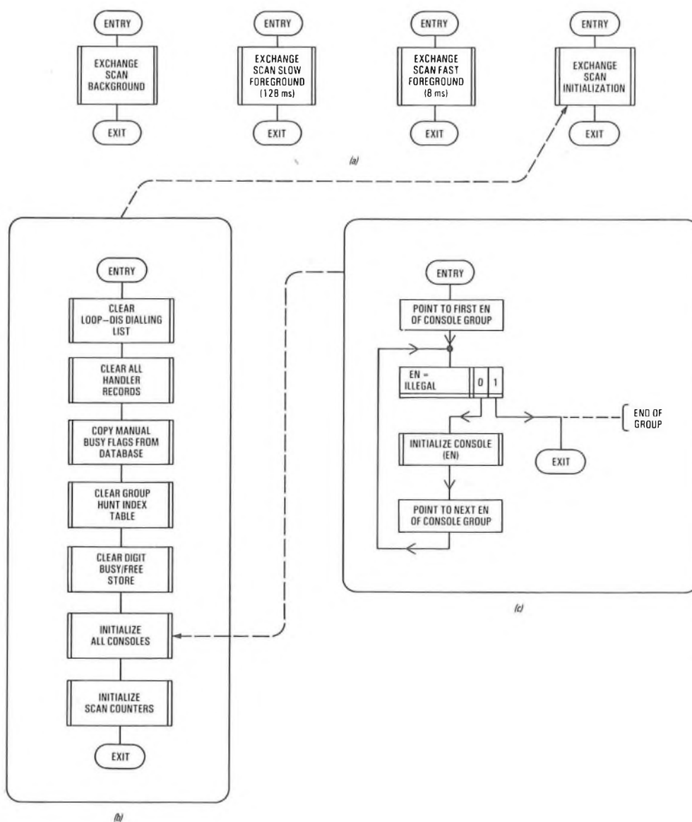
(a) Exchange scan overview (b) Exchange scan initialization (c) Console initialization EN: Equipment number LOOP-DIS: Loop-disconnect
