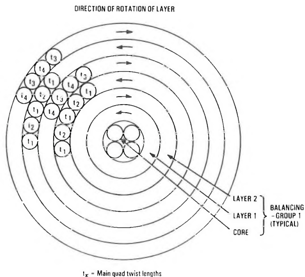
FIG. 3—Quad cable construction
