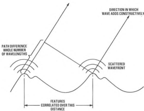
FIG. 4—Contribution of correlated errors to sidelobe gain
