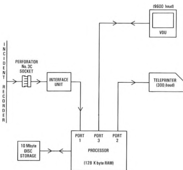
FIG. 7—Computer hardware
