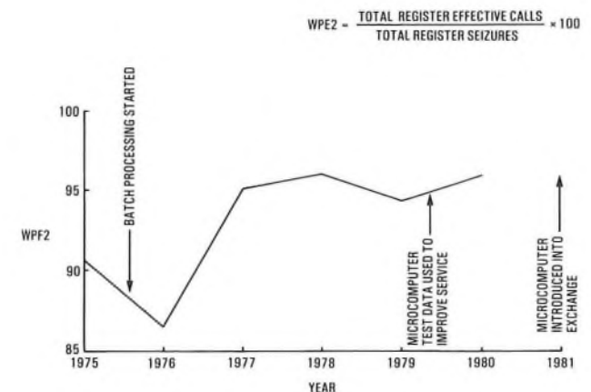
FIG. 6—Cambridge TXK4 weekly percentage figures (WPFs)
