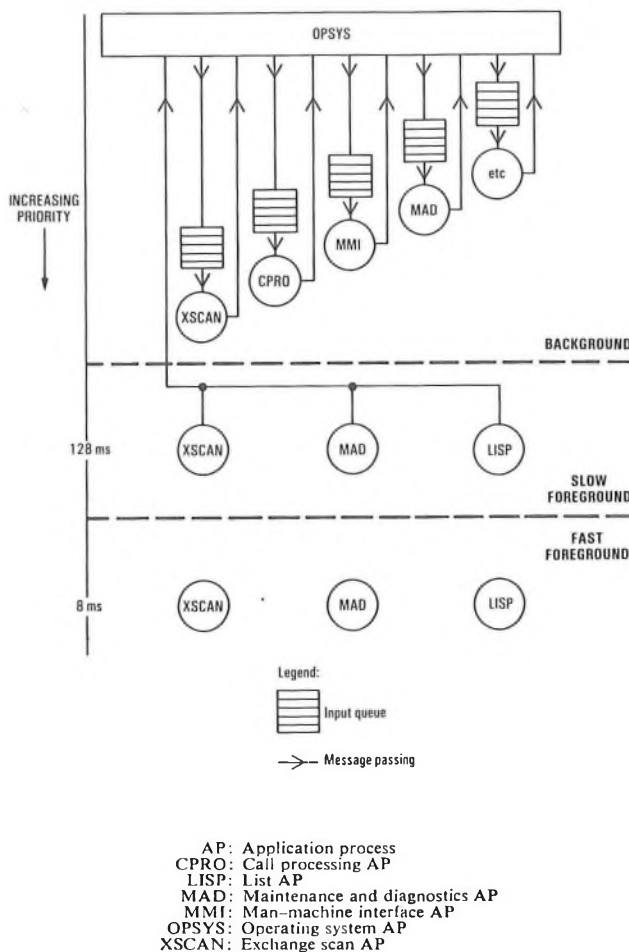
FIG. 1—Software organization
