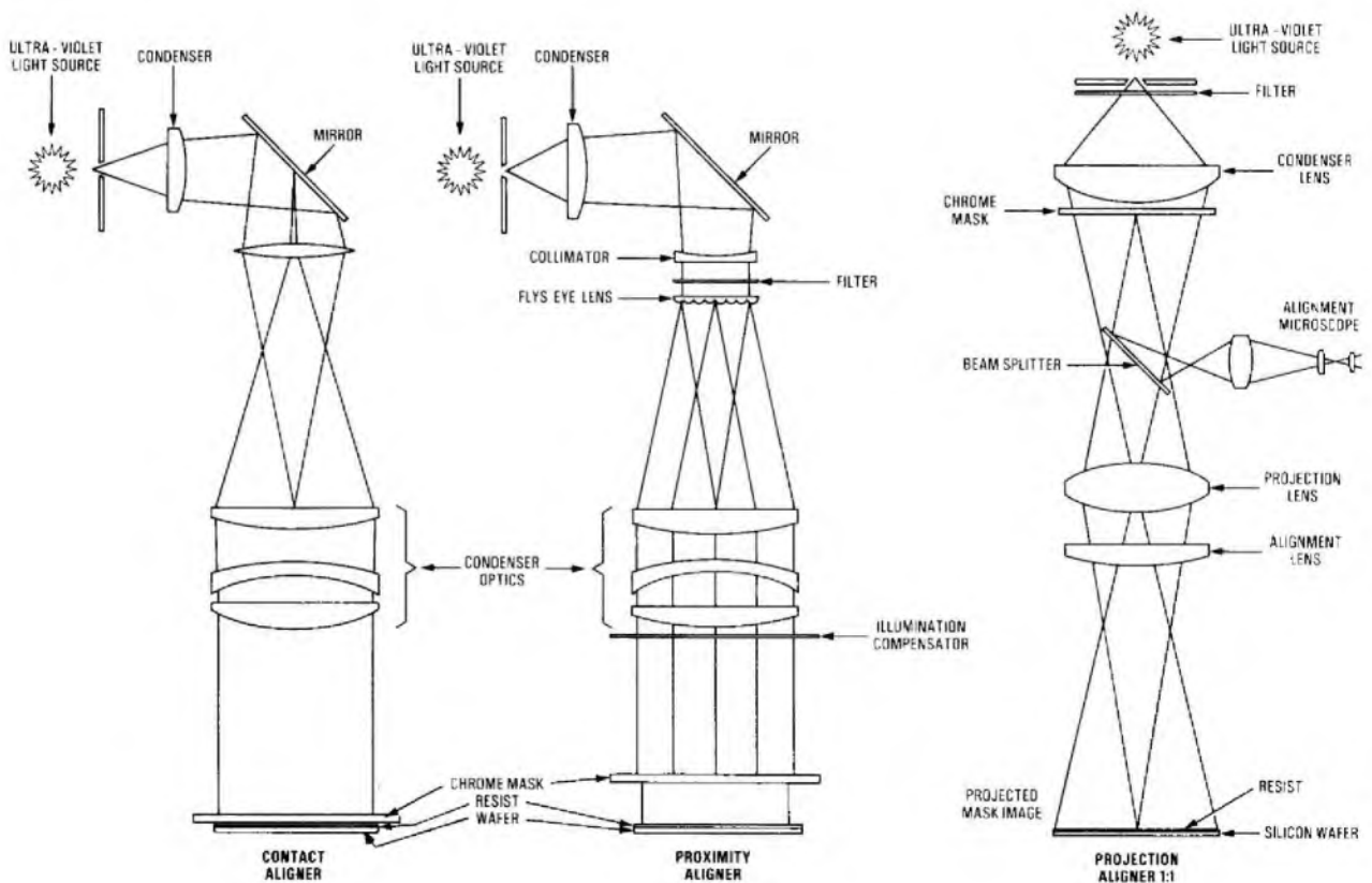
FIG. 7—Three methods of resist exposure
