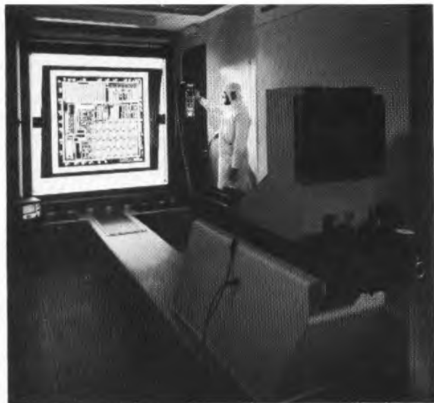
FIG. 3—First reduction camera
