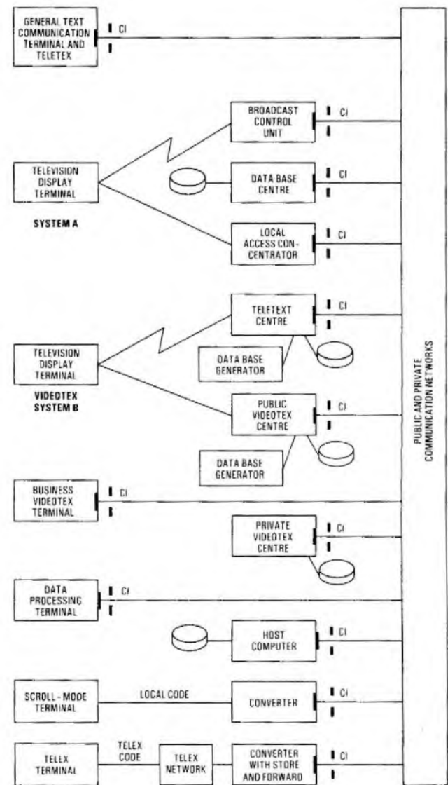
FIG. 7—Overall view of general text communication services
