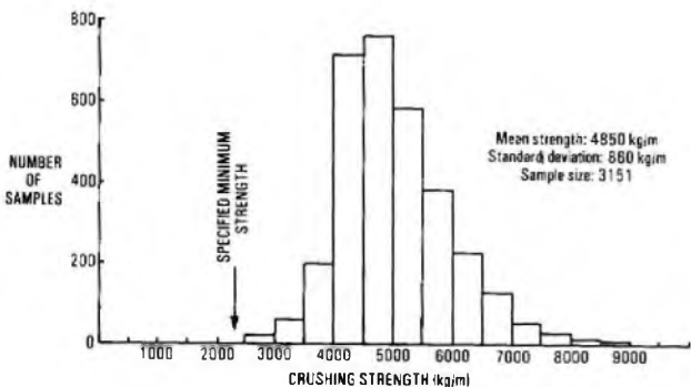
(b) Variation of crushing strength of BPO earthenware Ducts No. 15
