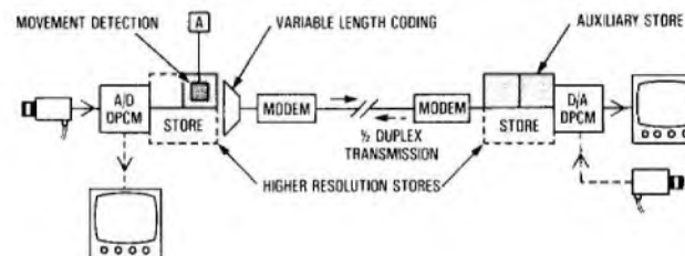
FIG. 1—Basic slow-scan television system
