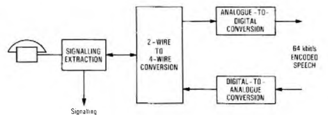
FIG. 1—Simplified speech path
