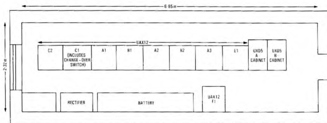
FIG. 4—Equipment layout for the feasibility study trial at the Glenkindie exchange
