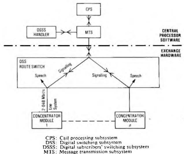
Fig. 2—Subsystem organization
