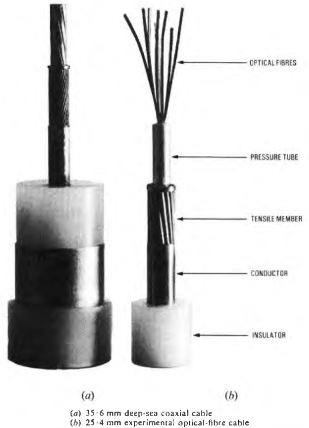
Comparison of coaxial and optical-fibre submarine cables
