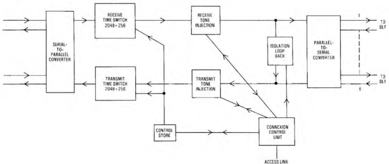
FIG. 7—Digital concentrator switch
