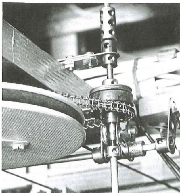
FIG. 3—Detail of clutch assembly
