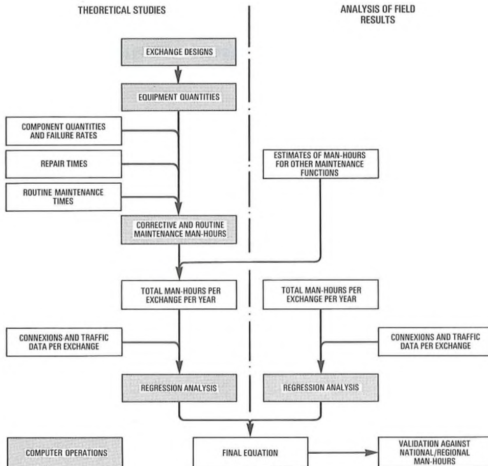
FIG. 1—Study methodology
