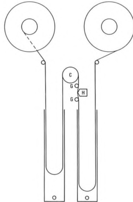
FIG. 10—Typical magnetic tape transport using vacuum-column reservoirs
