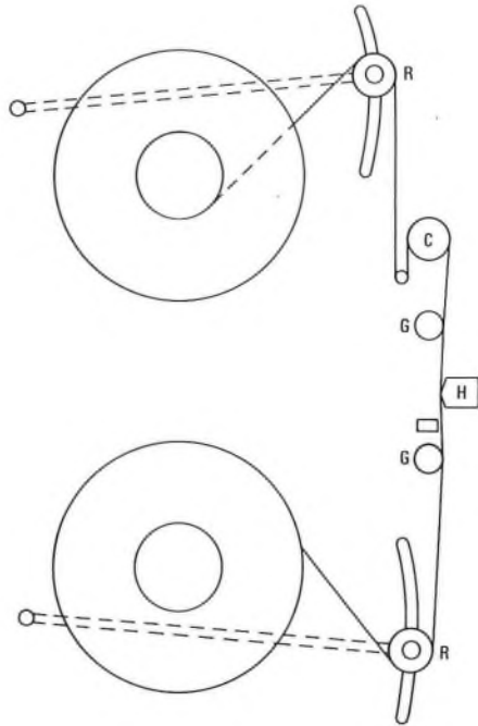
FIG. 9—Typical magnetic tape transport using swinging-arm reservoirs
