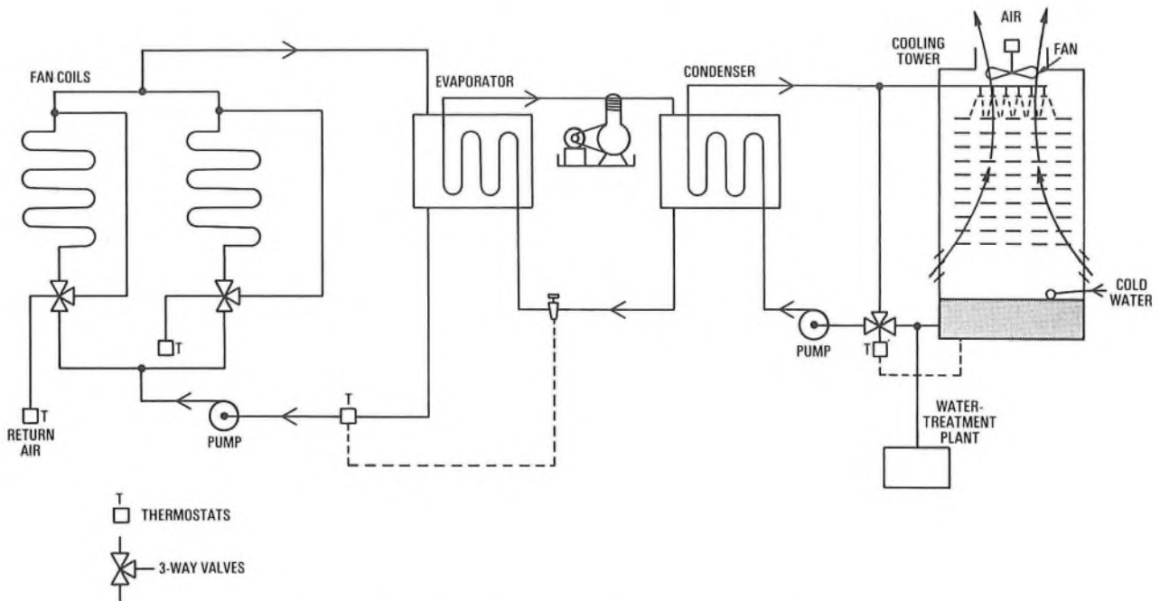
FIG. 10—Chilled-water system using evaporative cooling tower
