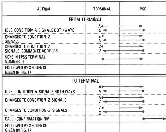
Fig. 19—Call set-up to and from a directly-connected terminal
