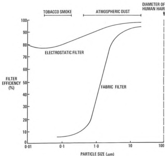
FIG. 8—Filter efficiency
