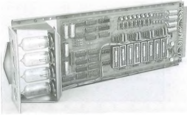
FIG. 3—Four-channel unit
