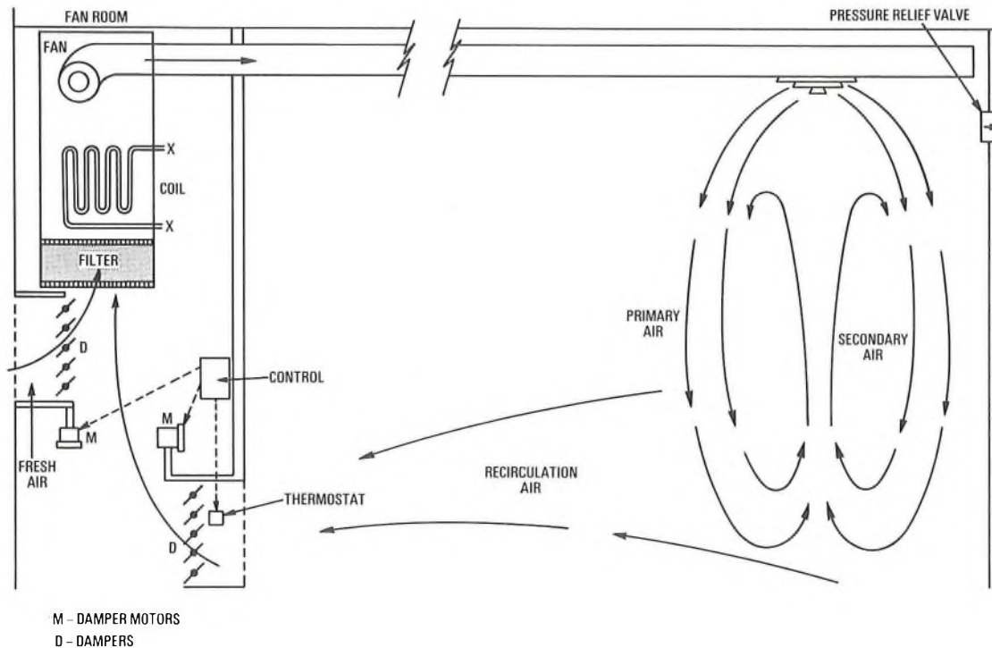
FIG. 7—Simplified block diagram of mechanical ventilation of an equipment room
