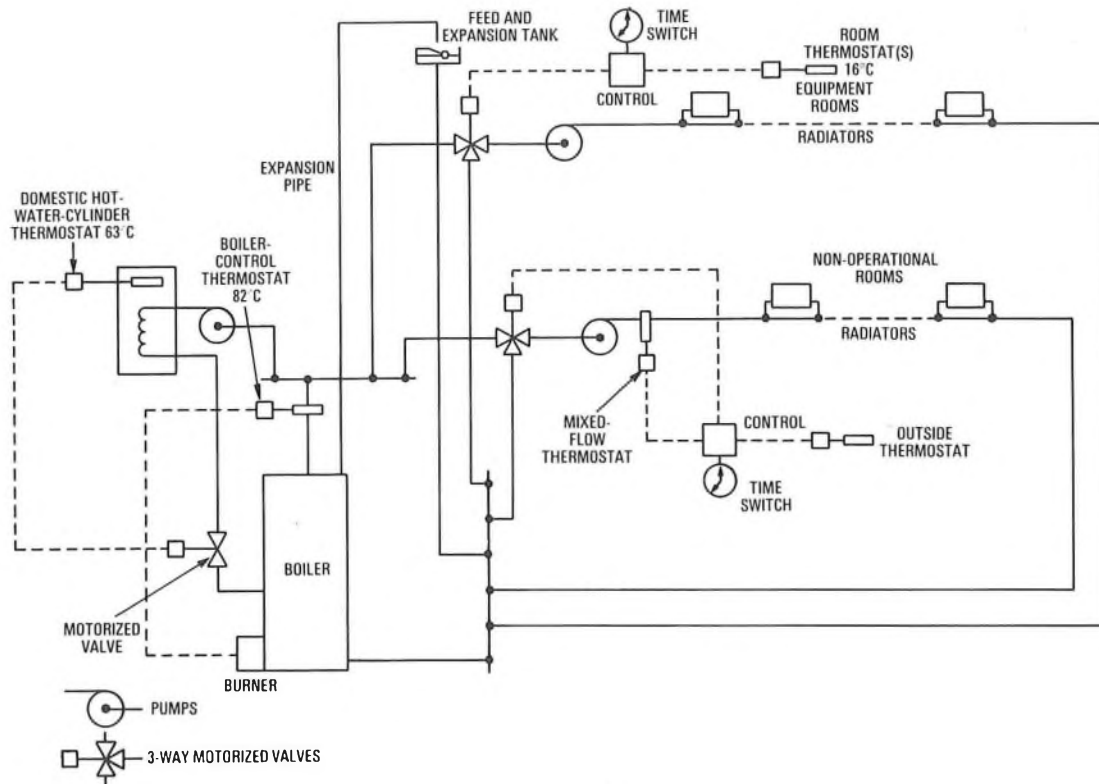
FIG. 6—Low-pressure hot-water system
