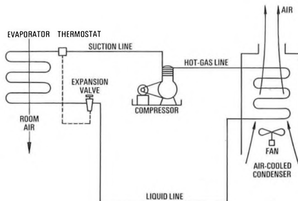
FIG. 9—Direct-expansion system using air-cooled condenser
