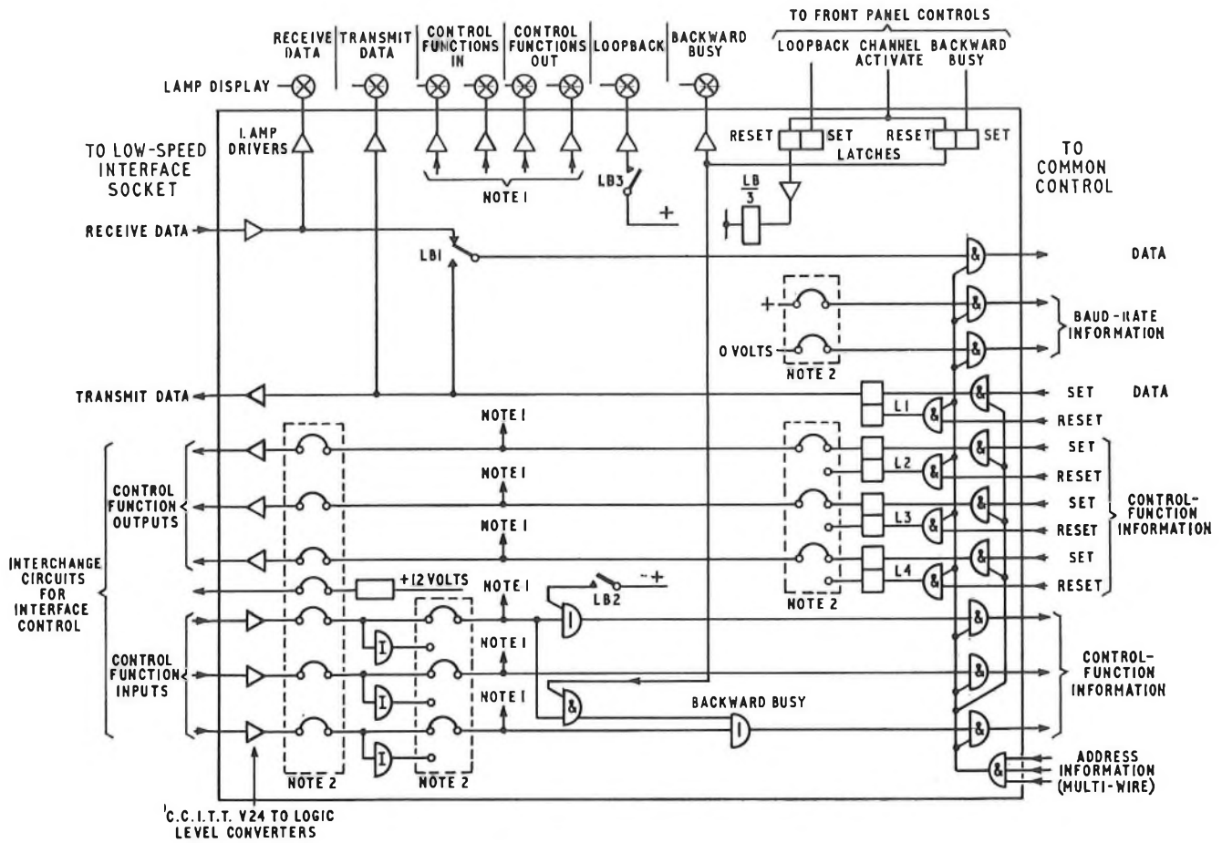
FIG. 5—Simplified block diagram of channel unit
