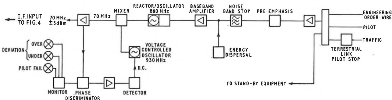
FIG. 3—Block diagram of baseband and modulator arrangements
