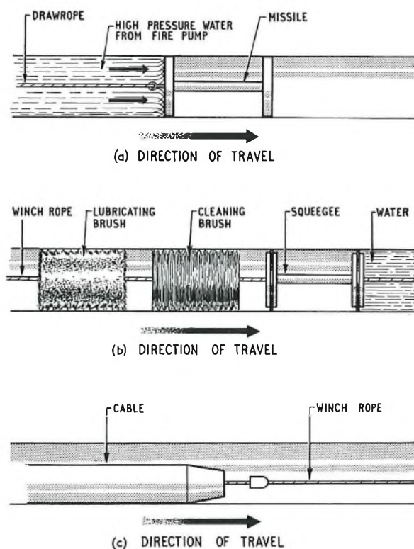
FIG. 6—Cabling operations
