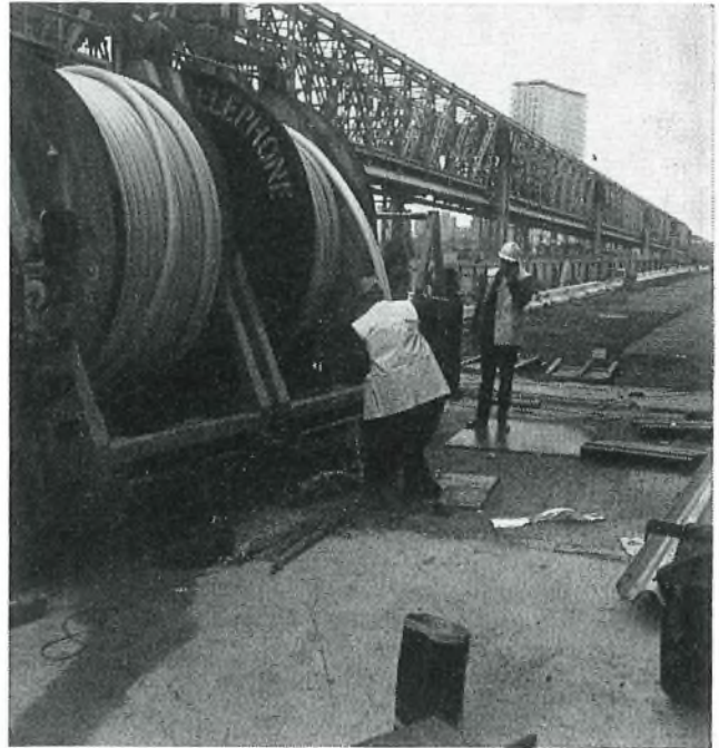
FIG. 2—Cable being fed into ducts, in the main diaphragm below, at the north side of London Bridge
