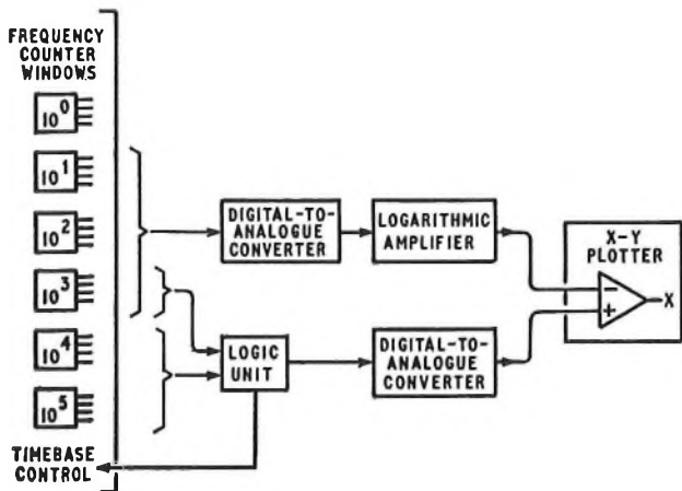
FIG. 3—Block diagram of a logarithmic frequency-plotter using analogue compression
