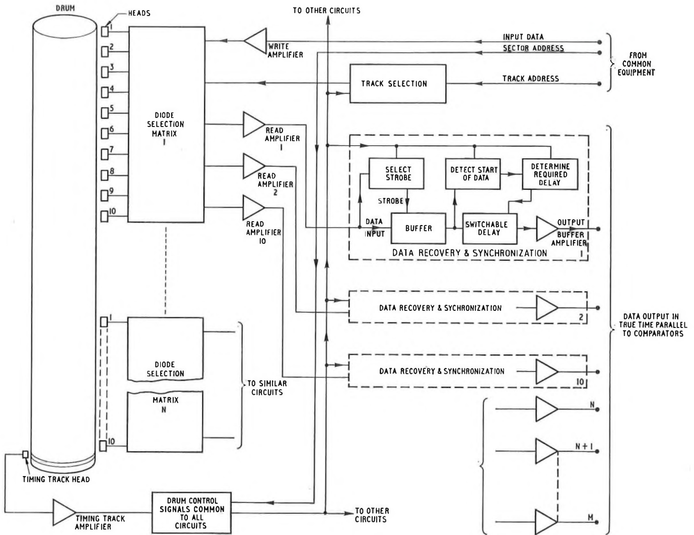
Fig. 4—Organization of drum-memory equipment
