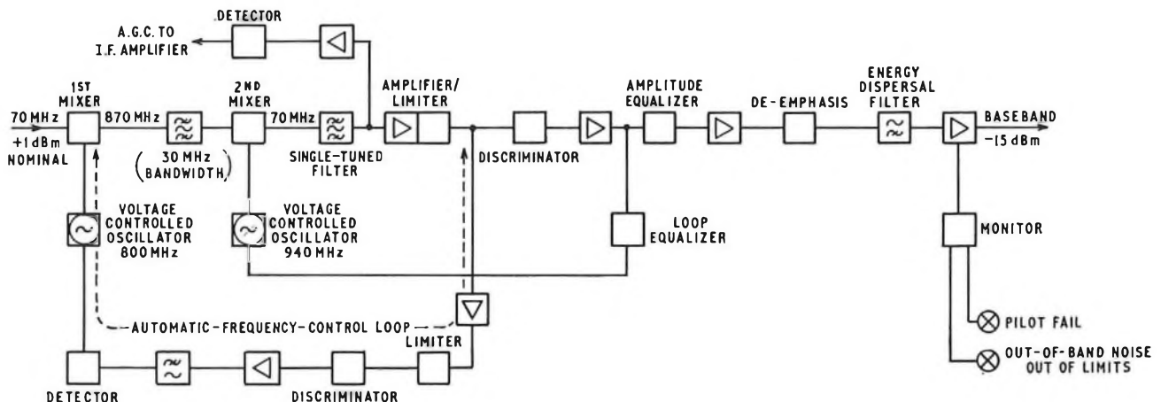
FIG. 8—Block diagram of f.m.f.b. demodulator
