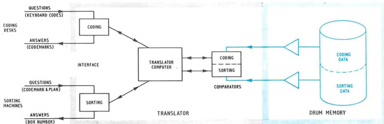
FIG. 1—The code-sort translator showing the position of the drum memory
