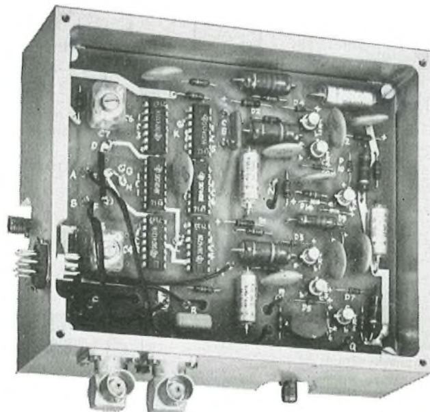
FIG. 6—Transmit unit—modulator drive circuitry
