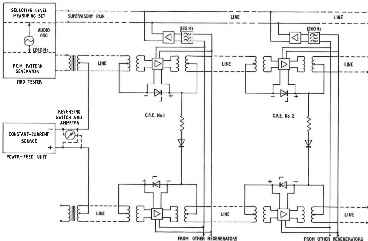
Fig. 5—Trio and reverse power testing
