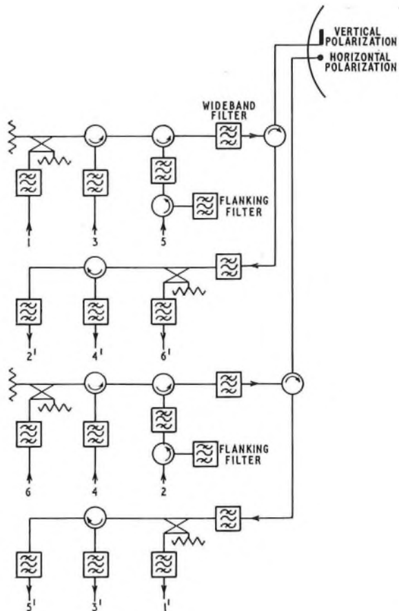
FIG. 3.—Typical multiplexing arrangement
