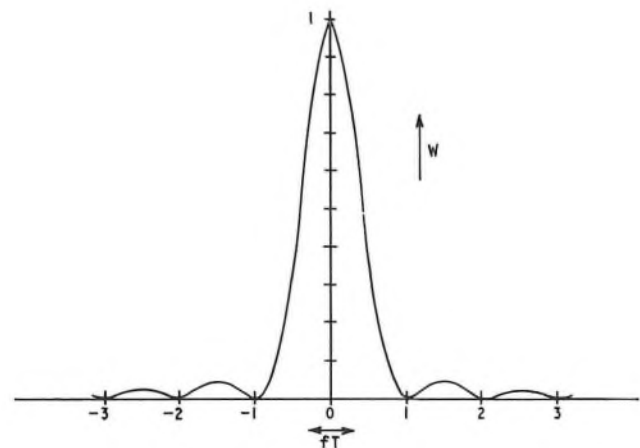
FIG. 1—Spectrum of a binary phase-modulated signal
