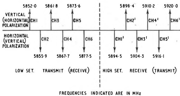
FIG. 2—Frequency-channelling plan
