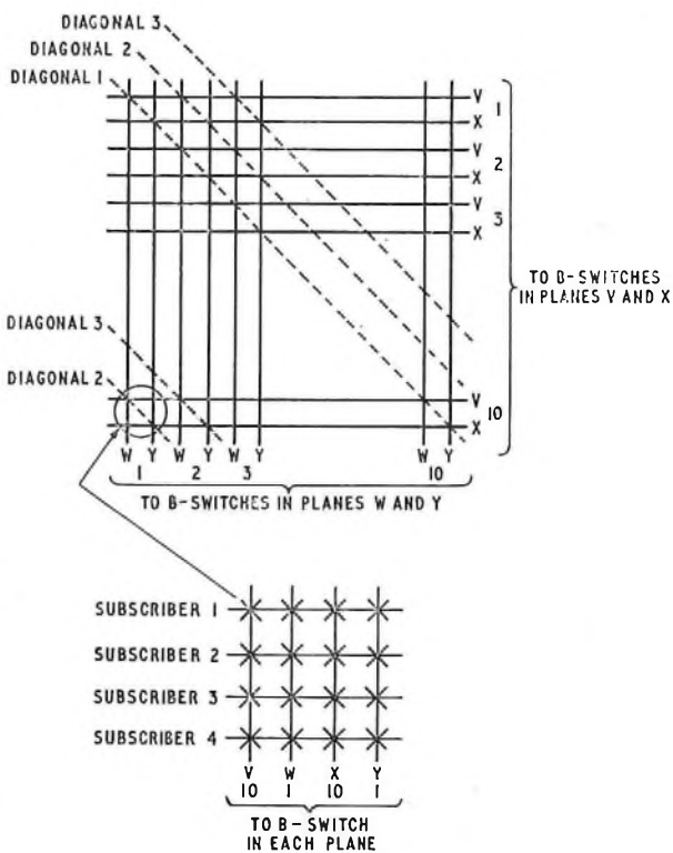
FIG. 3—Variable-concentration A-switch
