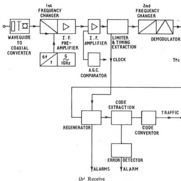
FIG. 4—Trunk digital channel
