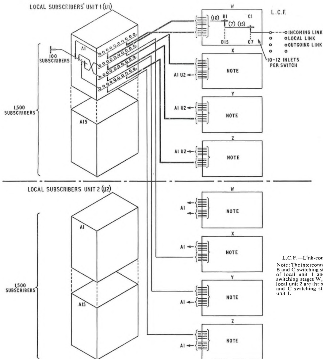
FIG. 2—Local-subscribers' unit trunking
