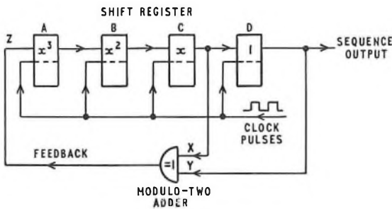
FIG. 3—Binary-pattern generator
