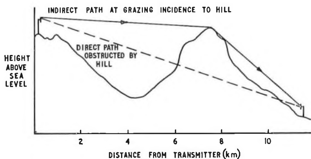
The vertical scale has been exaggerated and hence the radio path lengths appear distorted. In practice they are very nearly equal to the equivalent horizontal distances.
