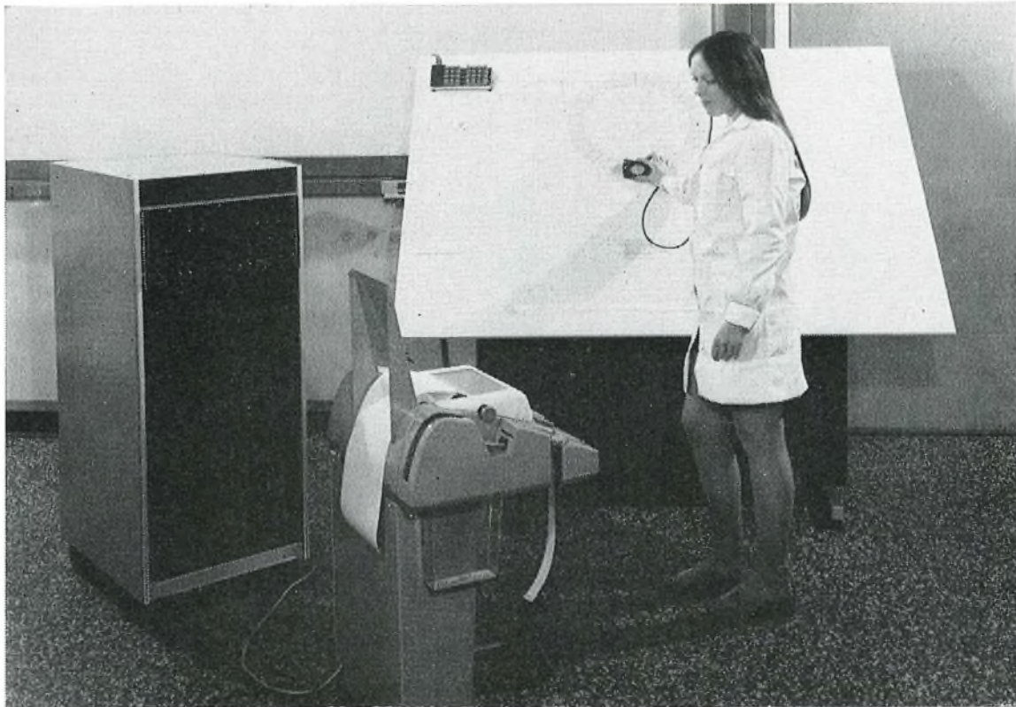
FIG. 3—Digitizing equipment
