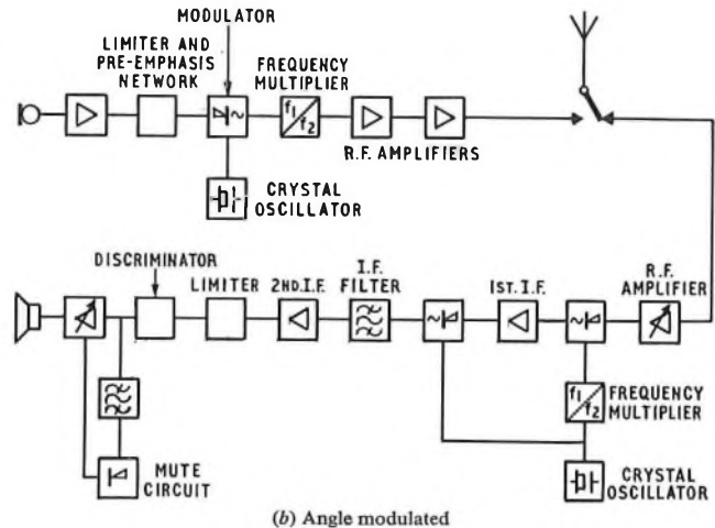
FIG. 3—Block diagrams of typical mobile-radio equipment.
