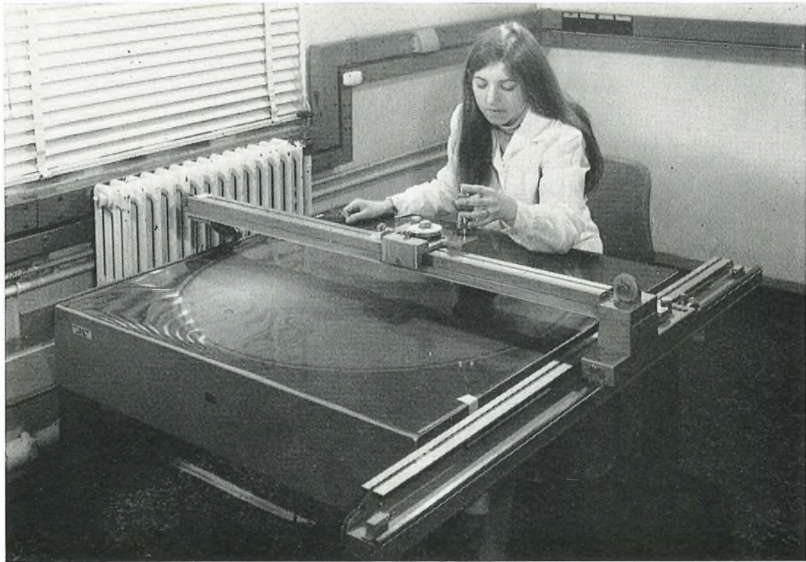
FIG. 5—Manual co-ordinatograph
