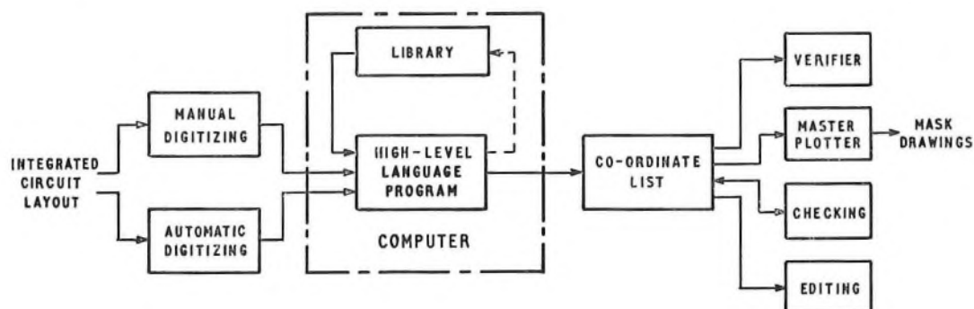
FIG. 1—System arrangement
