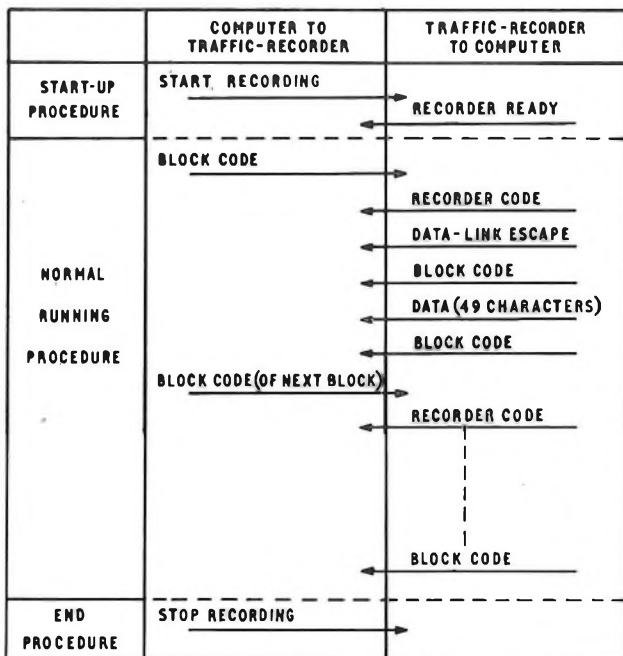
FIG. 4—Signalling sequence between the computer and the traffic recorder
