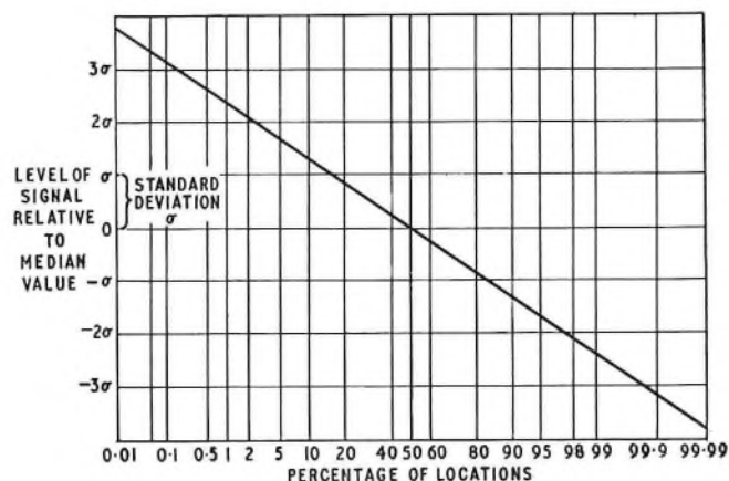
FIG. 6—Level of received signal relative to median value
