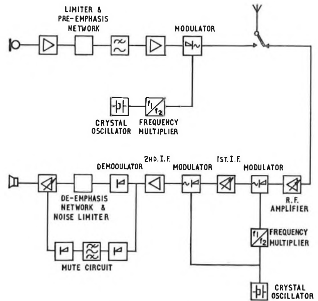
(a) Amplitude modulated
