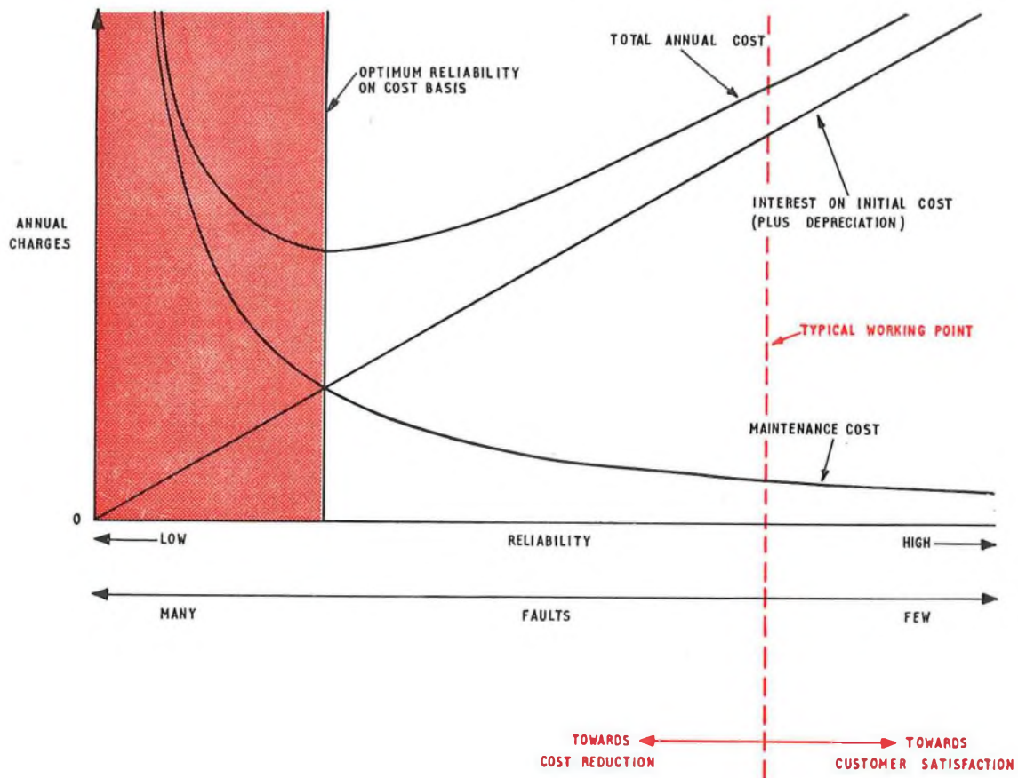
FIG. 2—Application of Kelvin's Economy Law to cable design philosophy
