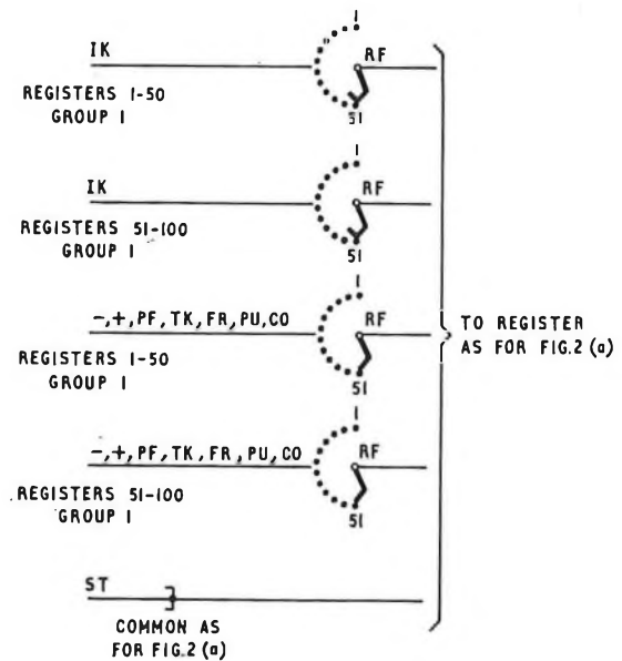
FIG. 2—Circuit diagram of the register-finder
