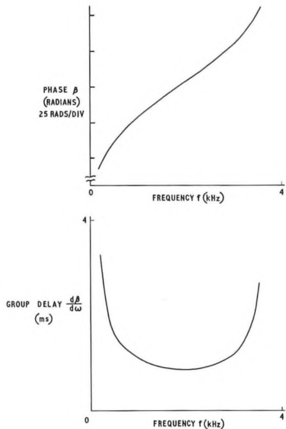
FIG. 4—Phase and group delay/frequency characteristics for a typical carrier channel
