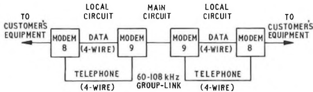
FIG. 2—Basic 48 kbit/s transmission circuit using Datal Modems No. 8 and 9
