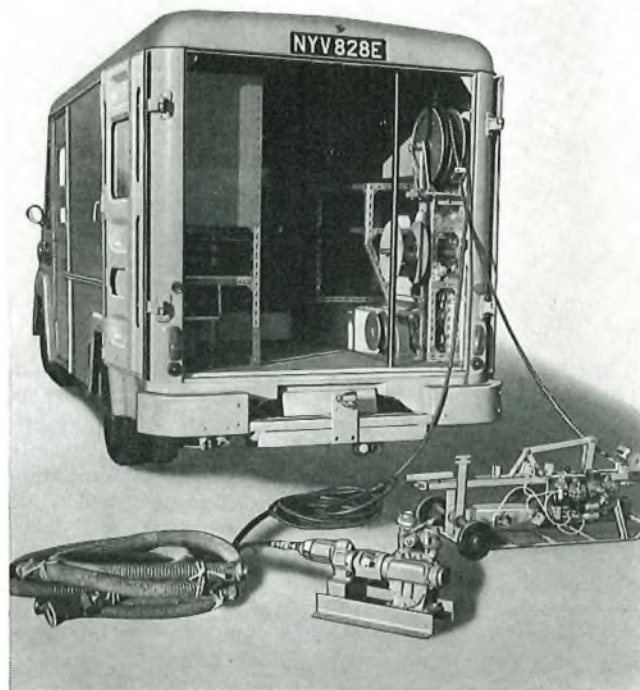
FIG. 1—Two-ton AIRVAN
