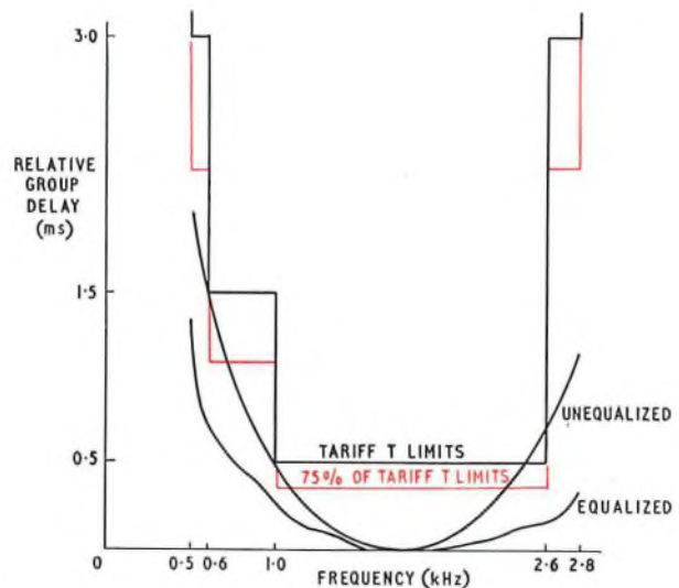
FIG. 8—Tariff T group delay/frequency distortion limits and typical equalized and unequalized circuit characteristics
