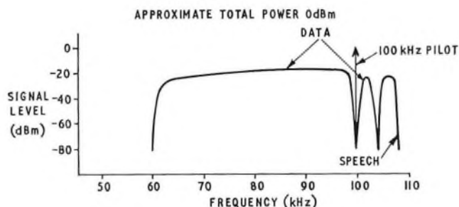
Fig. 1—Frequency spectrum of random data signal at "group-out" terminals of Datal Modem No. 9
