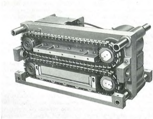
FIG. 2—Rod-pushing machine
