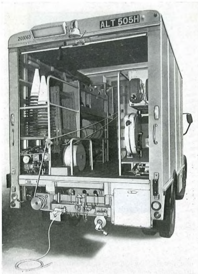
FIG. 4—Prototype hydraulic vehicle showing left-hand racking and winch with rope arranged
