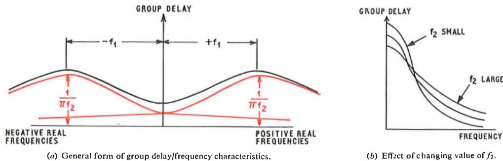
FIG. 7—Group delay/frequency characteristics of equalizer networks
