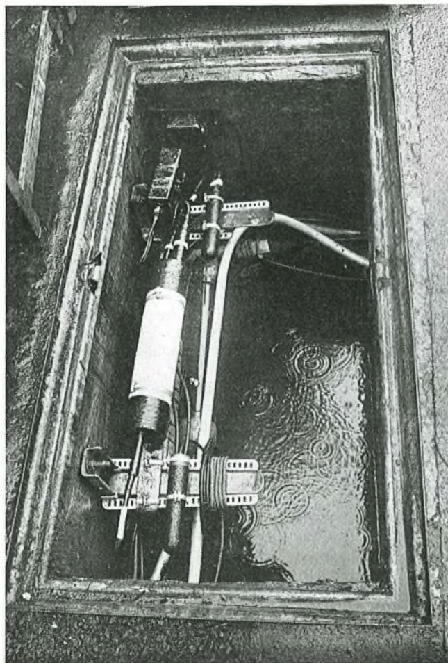
FIG. 6—V.H.F. line amplifier mounted in a joint-box at Washington New Town
