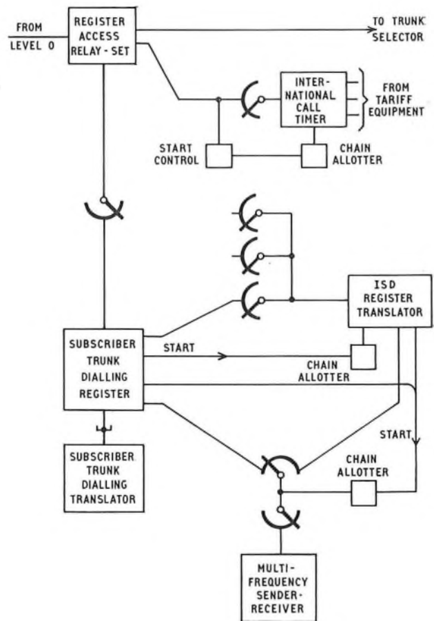
FIG. 1—Trunking diagram for i.s.d. calls at non-director g.s.c.s.
