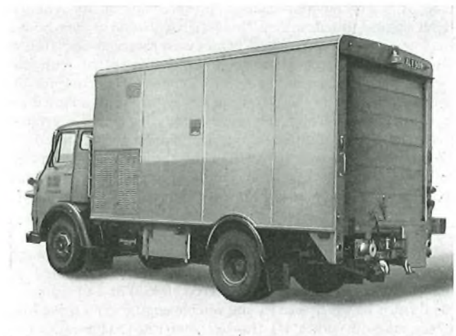
FIG. 5—Prototype hydraulic vehicle, general 3/4 rear view of whole vehicle
