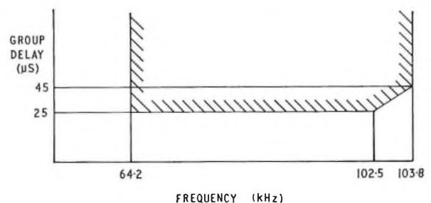
(a) Group-Delay/Frequency Distortion
