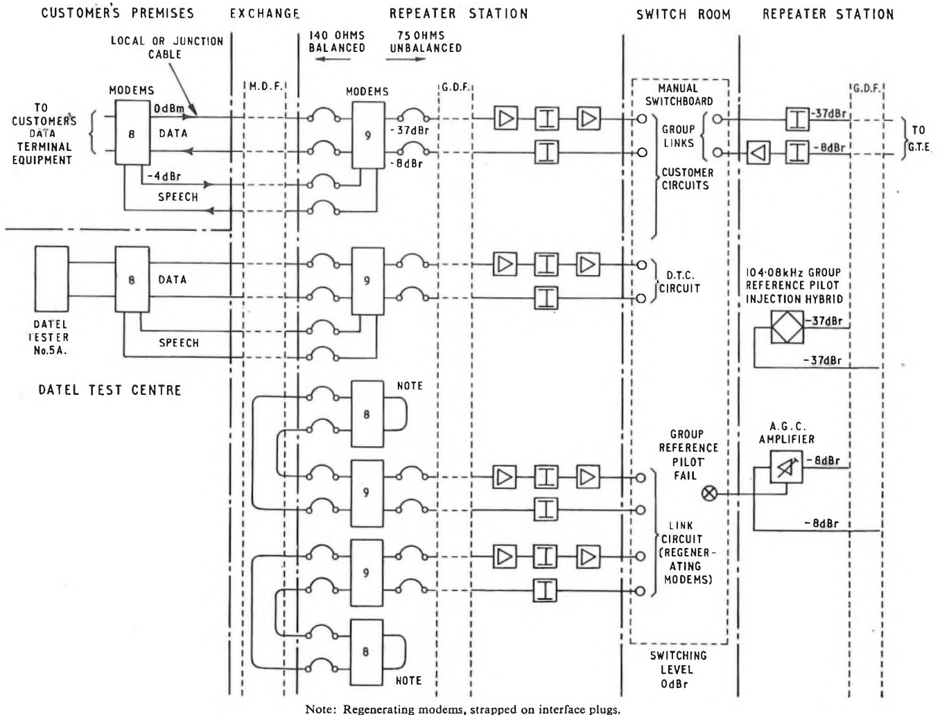
FIG. 6—Details of interconnexion of main items of plant
