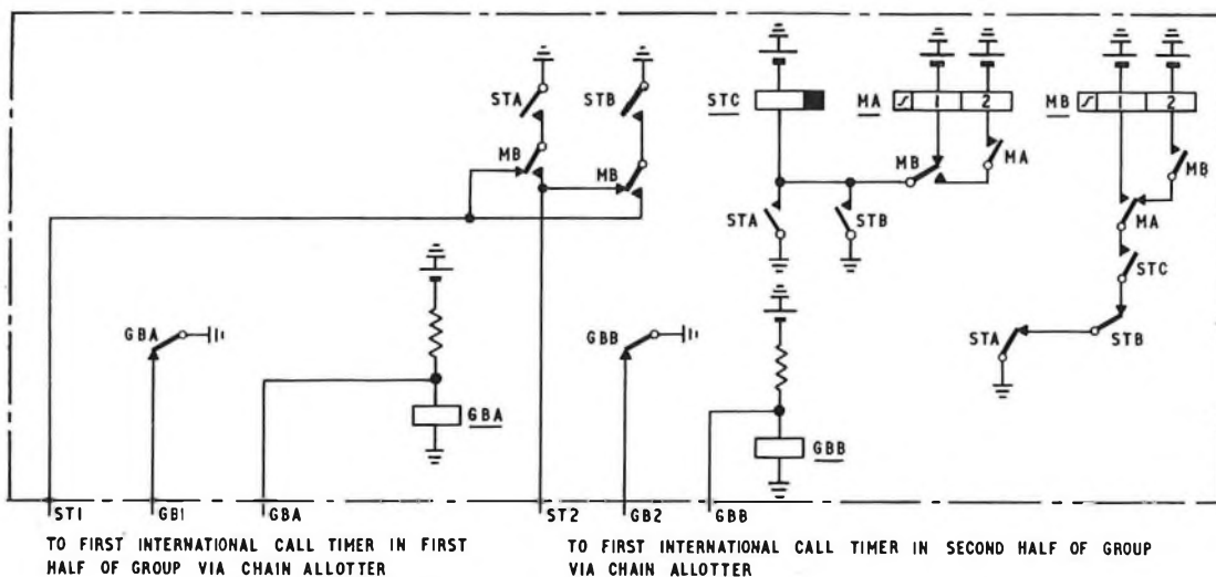
FIG. 8—Circuit diagram of the international-call-timer control circuit
