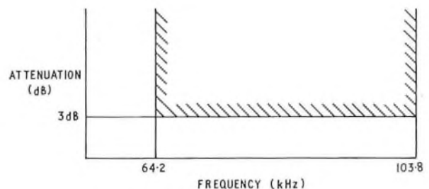
(b) Attenuation/Frequency Distortion
