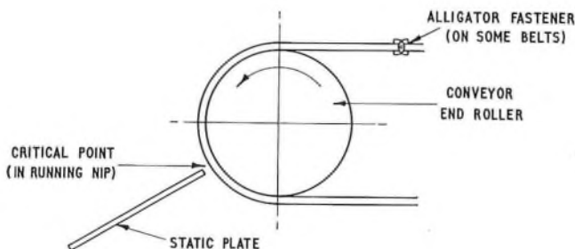
FIG. 1—Original configuration of conveyor end-roller and static plate
