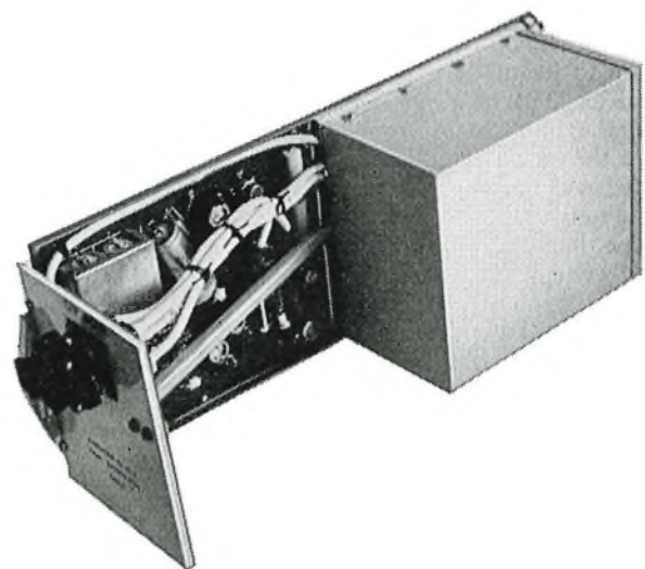
FIG. 4—Video line-amplifier
