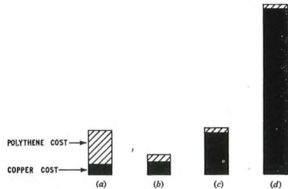
(a) x = 9 C = 20 nF/km (b) x = 2.5 C = 36 nF/km (c) x = 1.33 C = 83 nF/km (d) x = 1.1 C = 310 nF/km
