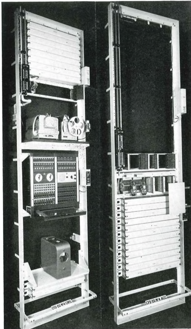
FIG. 1—Call-Failure-Detection Equipment No. 4
