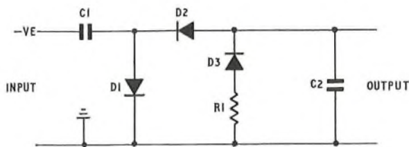
FIG. 2—Diode pump circuit
