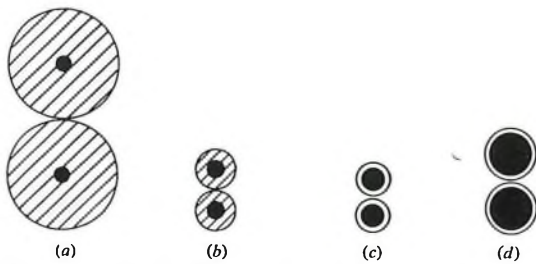
(a) x = 9 C = 20 nF/km (b) x = 2.5 C = 36 nF/km (c) x = 1.33 C = 83 nF/km (d) x = 1.1 C = 310 nF/km (Capacitances are for polythene insulation)
