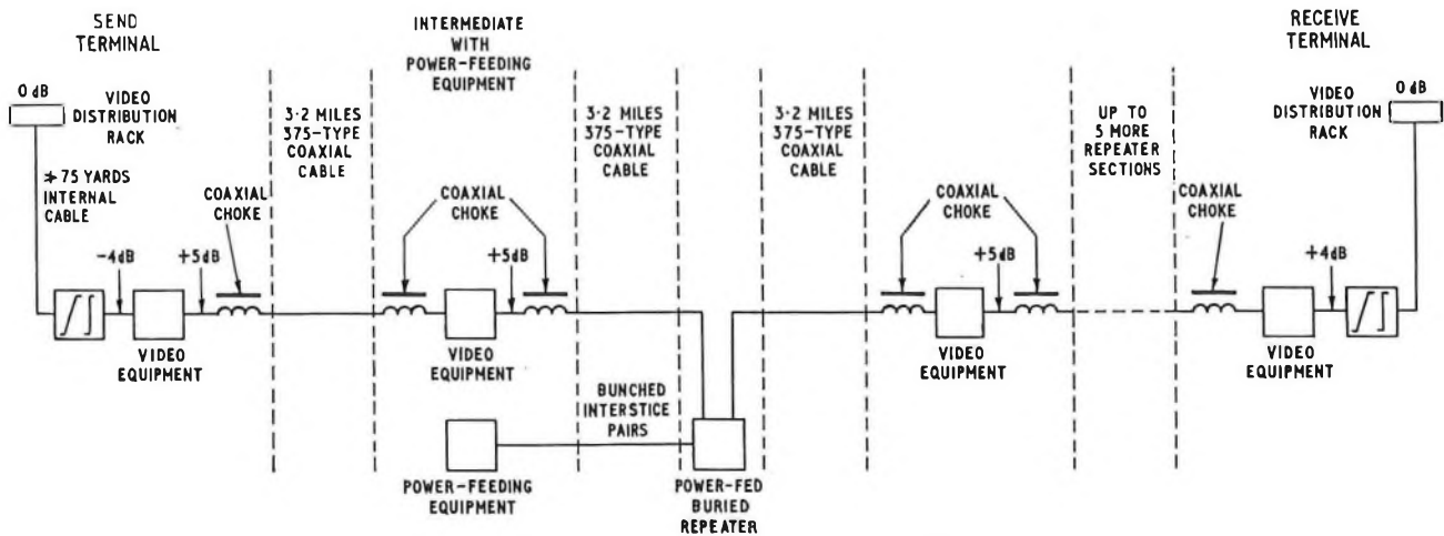
FIG. 1—Block schematic diagram of video system
