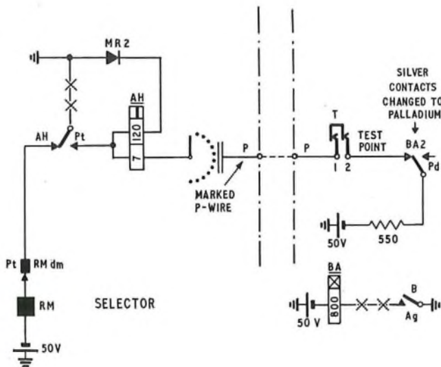
FIG. 13—Selector fails to switch to marked P-wire
