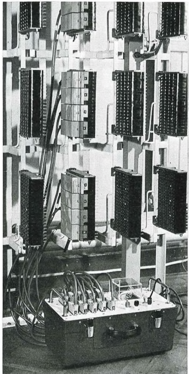
FIG. 1—Exchange equipment connected to type 8064 Fuse Mounting
