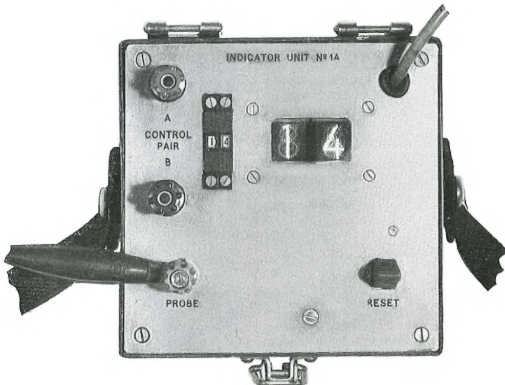
FIG. 3—Jointer's equipment
