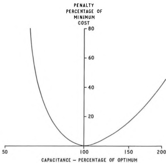
FIG. 4—Material-cost penalty for departure from minimum material-cost capacitance [copper conductors—polythene insulation]
