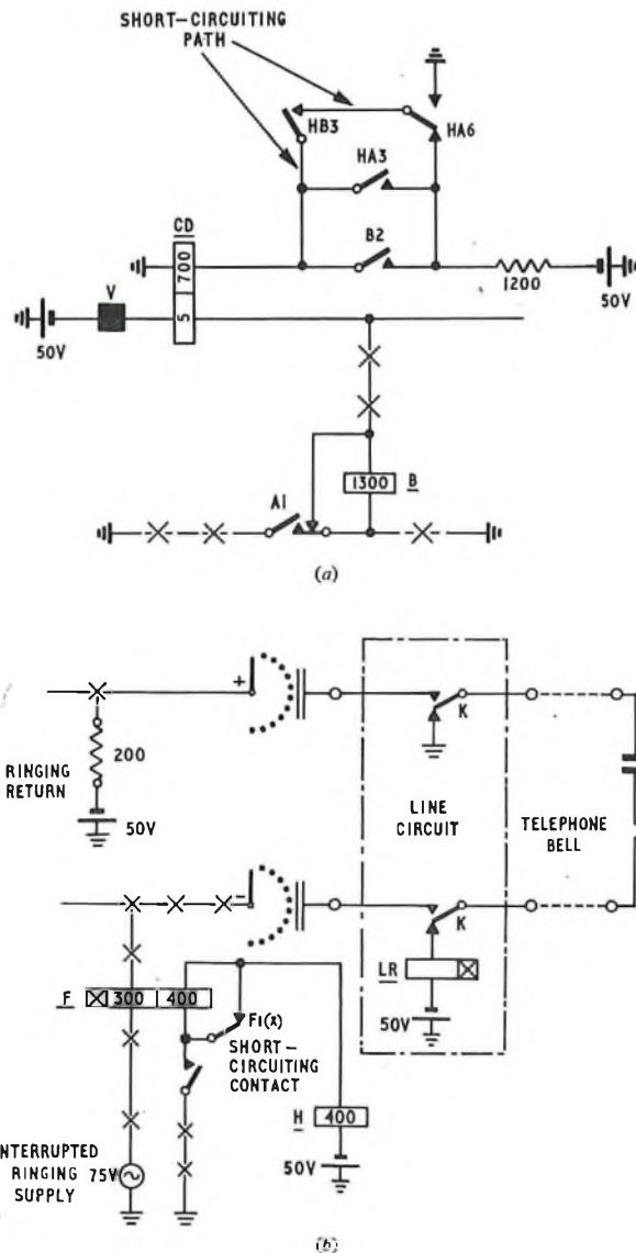
FIG. 15—Failures of short-circuiting function
