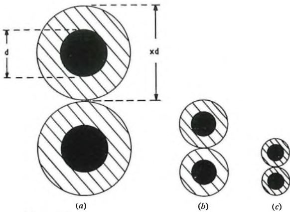
(a) x = 2 (b) x = 2 (c) x = 1.5 } cable pairs with equal capacitances (c) x = 1.5 cable pair with higher capacitance than (a) and (b)
