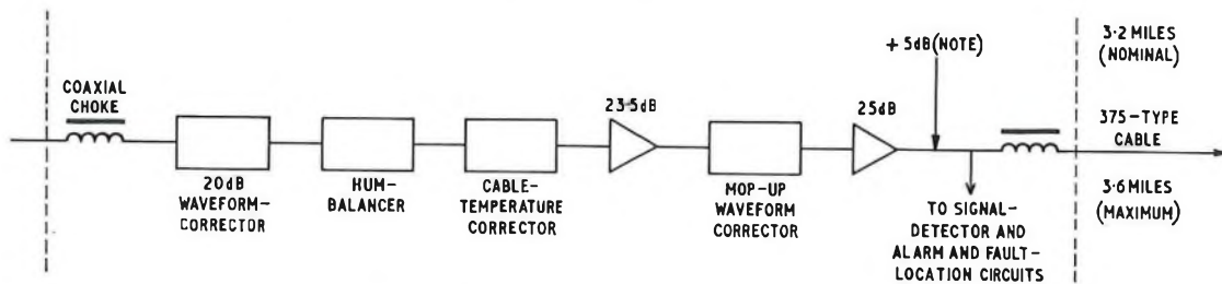
FIG. 2—Block schematic diagram of intermediate repeater
