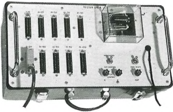
FIG. 2—Exchange equipment
