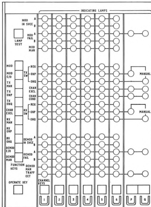
FIG. 4—Display-lamp and key layout
