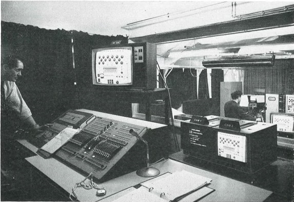
FIG. 5—Television studio and control room for video tape-recording production
