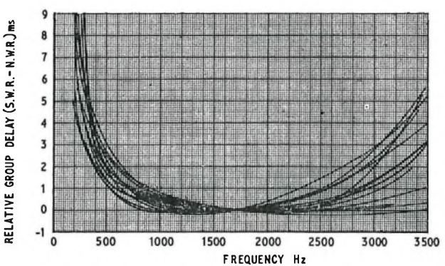
Fig. 6—Samples of group delay/frequency characteristics
