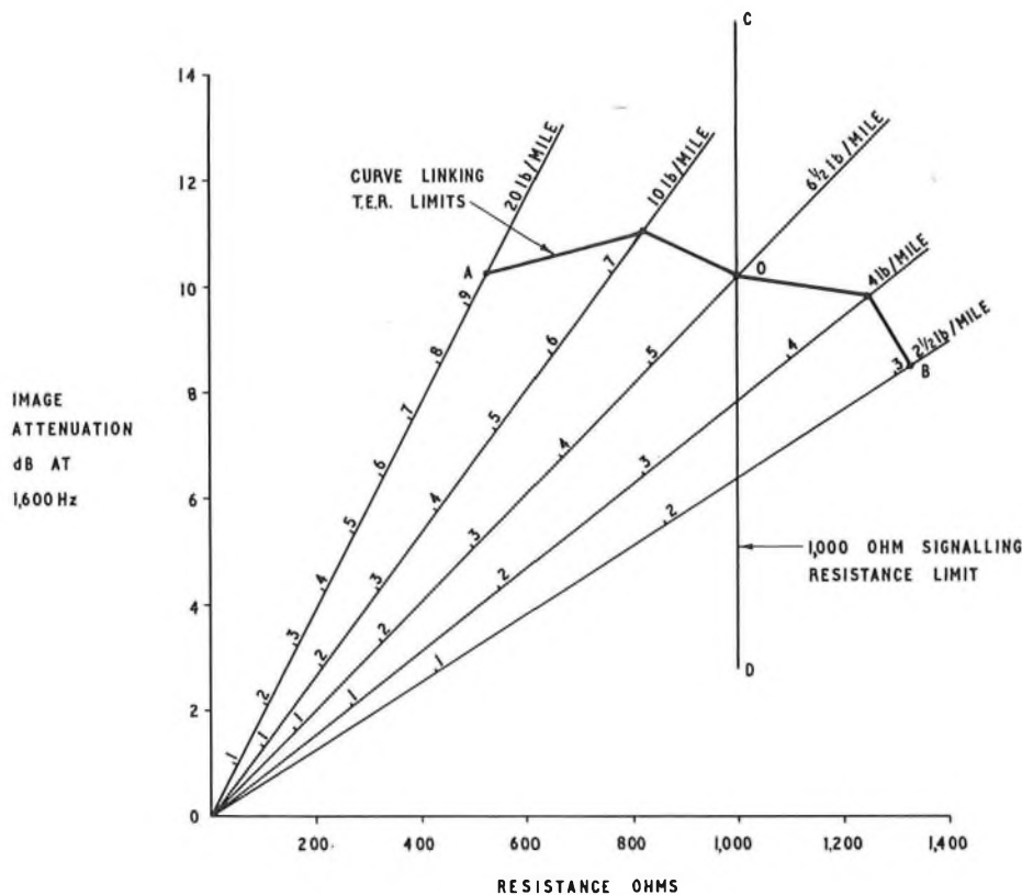
FIG. 1—T.E.R. limits presented in attenuation/resistance form
