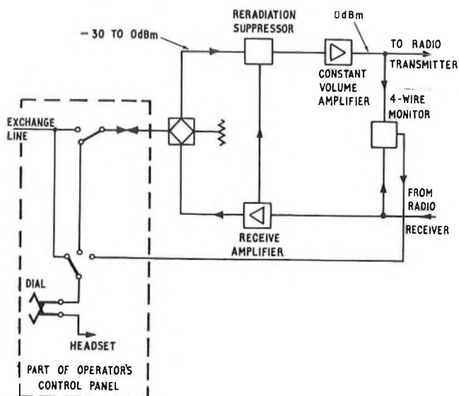
FIG. 3—Coast station radiotelephone terminal (schematic)
