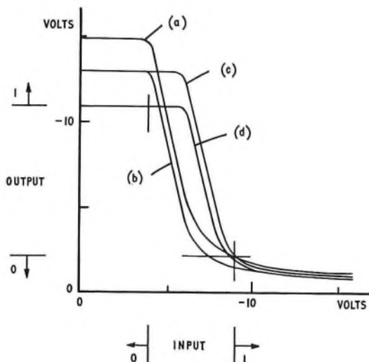
(a) V_{DD} = -20 volts V_t = -4 volts (c) V_{DD} = -20 volts V_t = -6 volts (b) V_{DD} = -18 volts V_t = -4 volts (d) V_{DD} = -18 volts V_t = -6 volts
