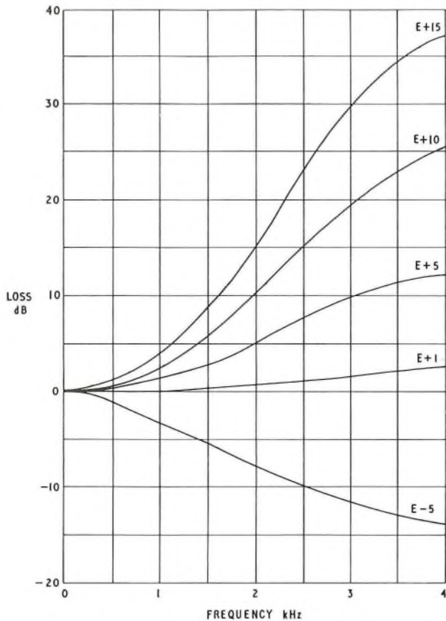
FIG. 3—Attenuation/frequency characteristics
