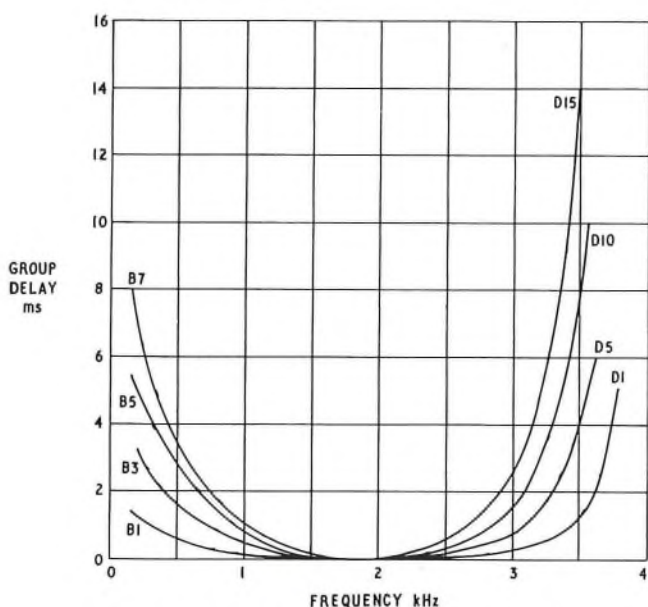
FIG. 7—Group-delay/frequency characteristics
