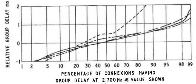
Fig. 7—Regional and inter-regional traffic-weighted cumulative distributions of group delay relative to that at 1,700 Hz
