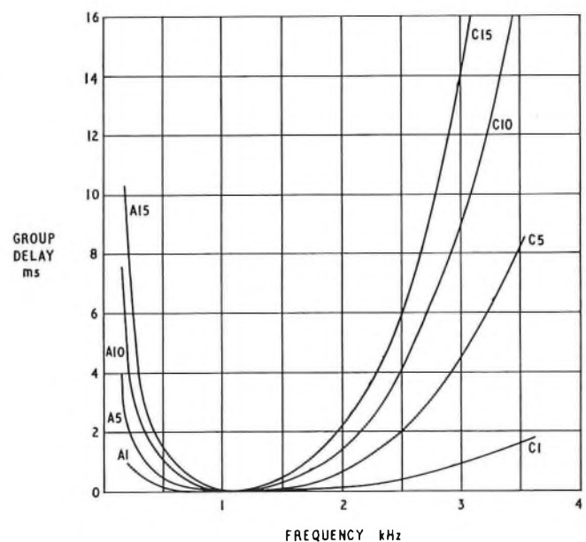
FIG. 6—Group-delay/frequency characteristics
