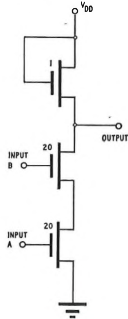
FIG. 5—Static 2-input NAND gate
