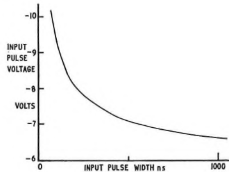
Relationship between pulse width and amplitude applied to one input of 3-input static NOR gate for output level -5 volts. V_{DD} = -20 volts
