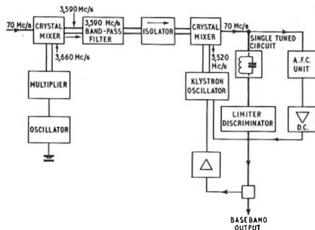
FIG. 10—SIMPLIFIED BLOCK-SCHEMATIC DIAGRAM OF THE FREQUENCY-MODULATION NEGATIVE-FEEDBACK RECEIVER
