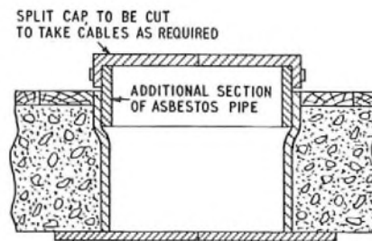
(c) Section Showing Arrangement for Feeding to Vertical of Intermediate Distribution Frame when Frame is Extended.
