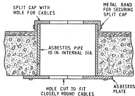
(a) Section of Hole for Feeding to Equipped Vertical of Intermediate Distribution Frame.
