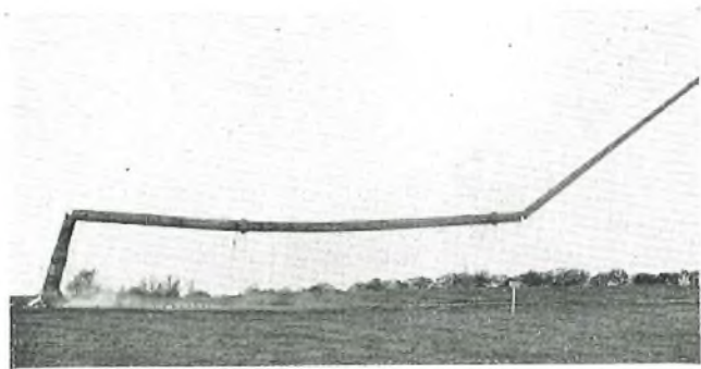
FIG. 5—THIRD MAST JUST BEFORE HITTING GROUND
