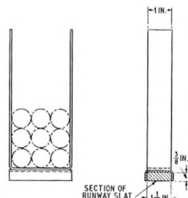
FIG. 2—SKETCH OF CABLE CLIP
