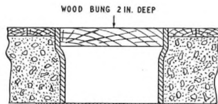
(b) Section of Sealed Hole in Area Reserved for Extension of Intermediate Distribution Frame.
