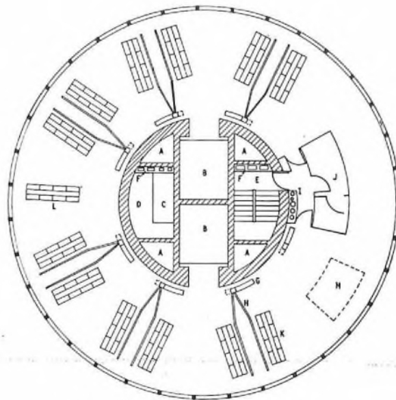
FIG. 4—TYPICAL LAYOUT OF APPARATUS FLOOR AND CENTRAL SHAFT
