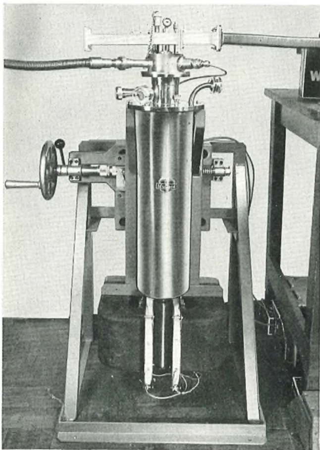
FIG. 9—THE GOONHILLY MASER AMPLIFIER
