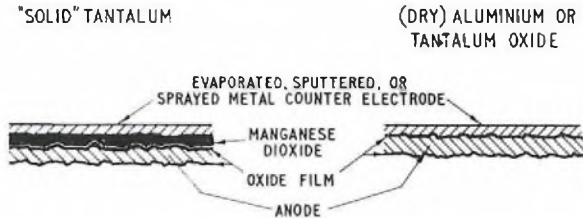
FIG. 4—"SOLID" TANTALUM AND "DRY" ALUMINIUM OR TANTALUM-OXIDE CAPACITOR CONSTRUCTION
