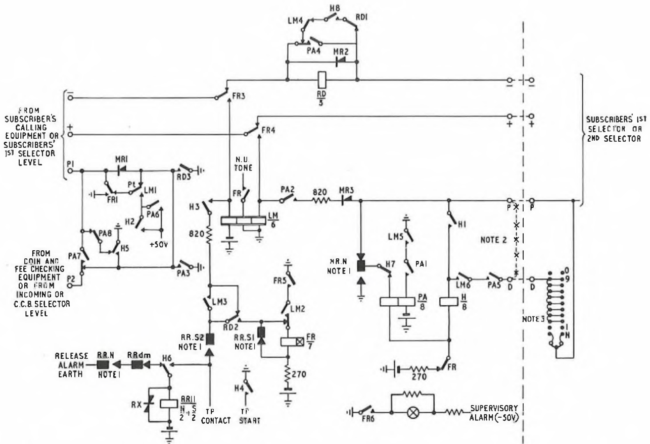
FIG. 2—CIRCUIT OF LOCAL-CALL TIMER
