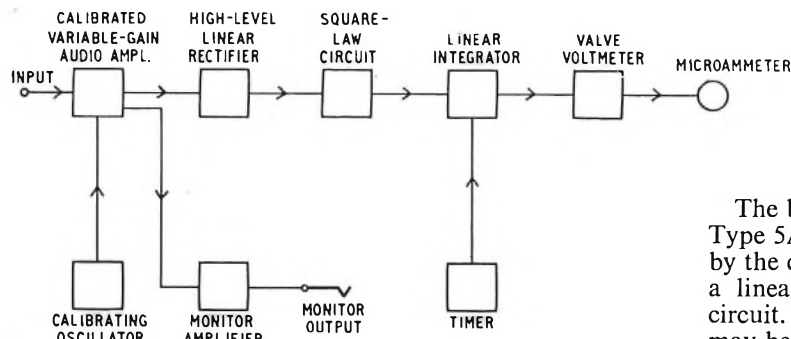
FIG. 1—BLOCK SCHEMATIC DIAGRAM OF SPEECH VOLTMETER TYPE 5A
