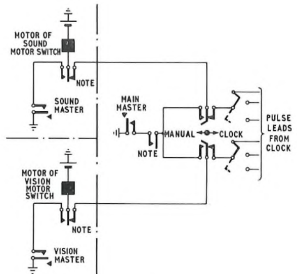
Note: For manual operation these keys are depressed simultaneously with the main master key FIG. 7—MASTER SWITCHING UNIT
