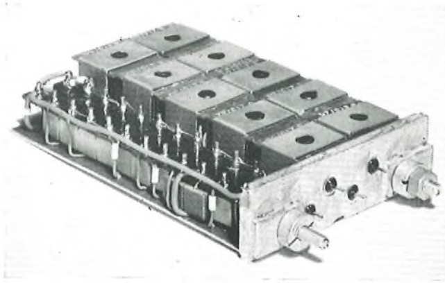
FIG. 6—CHANNEL FILTER
