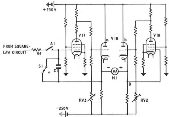
FIG. 4—SIMPLIFIED INTEGRATOR AND VALVE-VOLTMETER CIRCUITS
