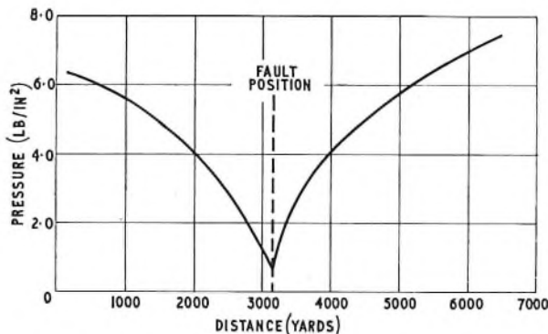
FIG. 1.—TYPICAL PRESSURE/DISTANCE CHARACTERISTIC OF FAULTY GAS-FILLED CABLE
