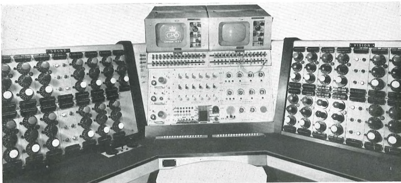
FIG. 8—SWITCHING CONSOLE
