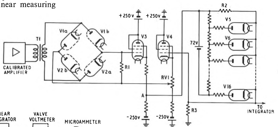
FIG. 2—SIMPLIFIED LINEAR-RECTIFIER AND SQUARE-LAW CIRCUITS
