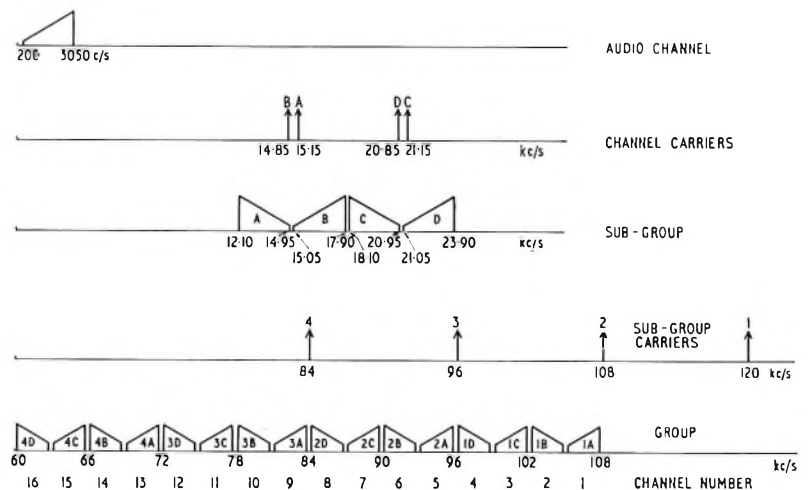
FIG. 1—FREQUENCY ALLOCATION
