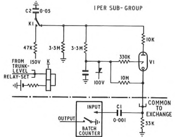
FIG. 3—COUNTING CIRCUIT
