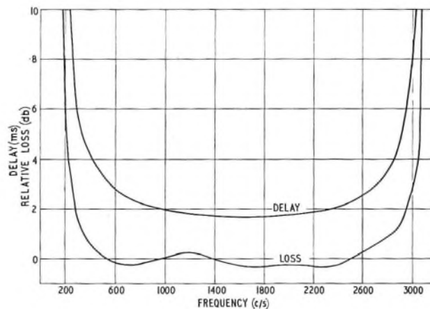
FIG. 3—TYPICAL CHANNEL AUDIO-AUDIO FREQUENCY CHARACTERISTICS
