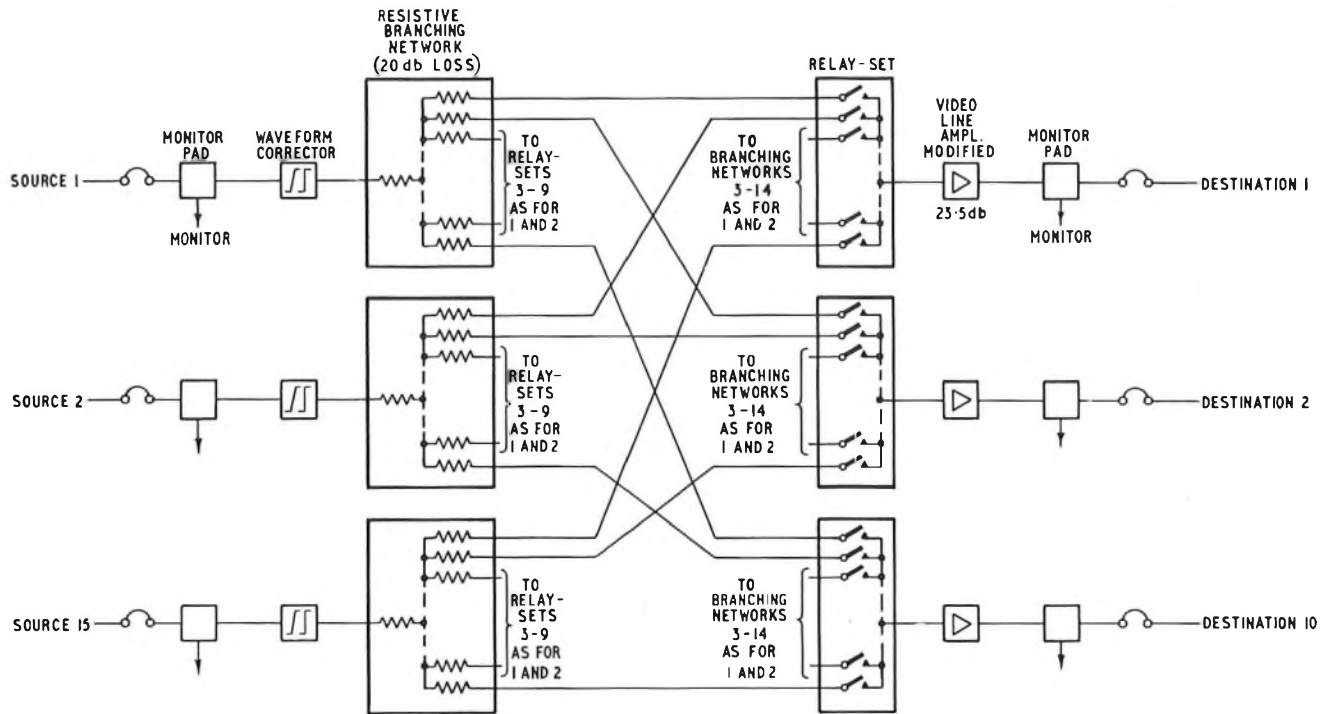
FIG. 3—SIMPLIFIED SCHEMATIC OF TRANSMISSION PATH FOR VISION-CIRCUIT SWITCHING
