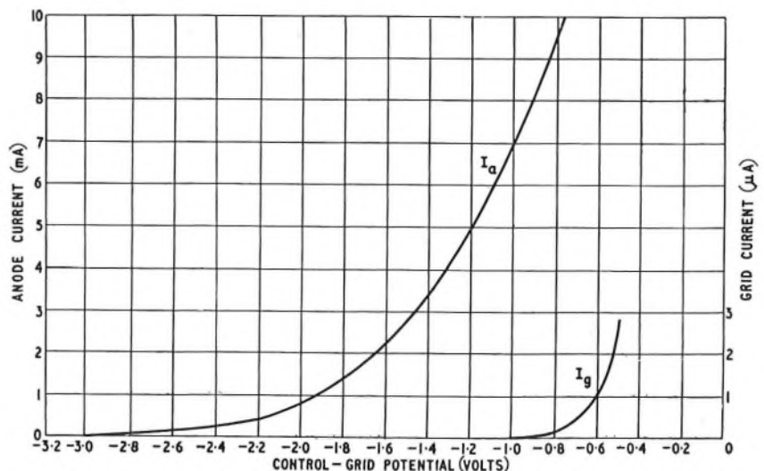
FIG. 3—TYPICAL MUTUAL AND GRID-CURRENT CHARACTERISTICS OF 10P2-TYPE VALVE
