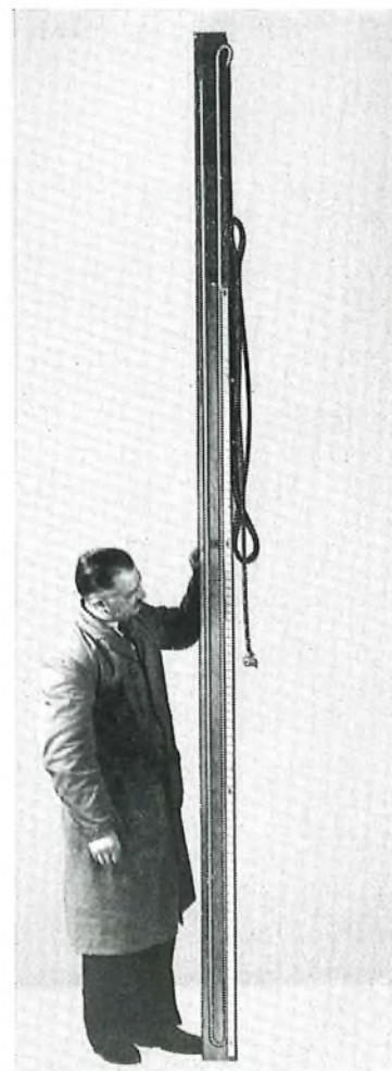
FIG. 2—LOW-DENSITY-LIQUID MANOMETER
