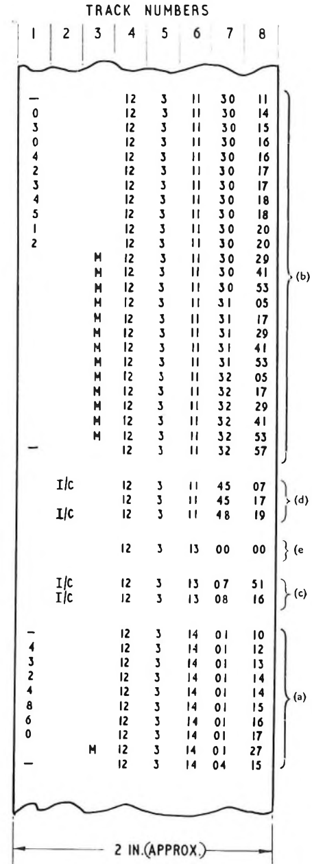
FIG. 1—TYPICAL SECTION OF RECORDINGS ON THE PAPER TAPE
