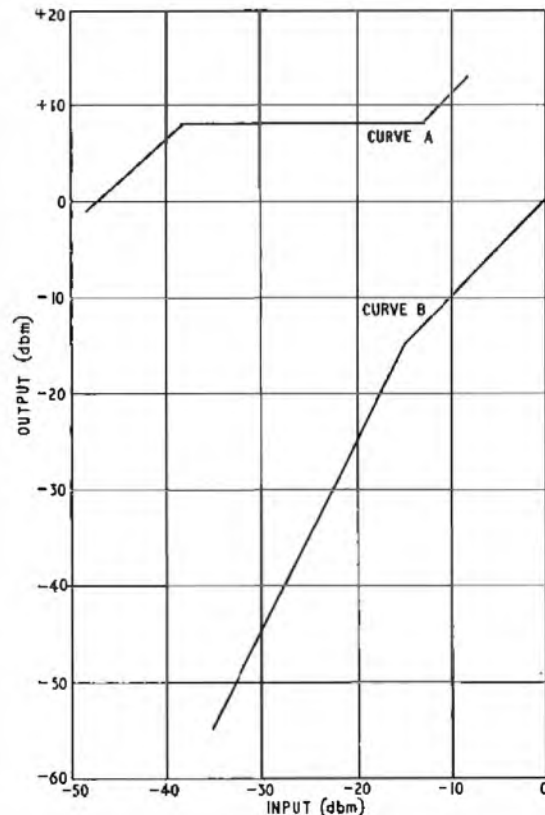
Curve A—Constant-Volume-Amplifier Characteristic Curve B—Noise-Reducer Characteristic FIG. 6—OPERATING CHARACTERISTICS OF THE CONSTANT-VOLUME AMPLIFIER AND NOISE REDUCER
