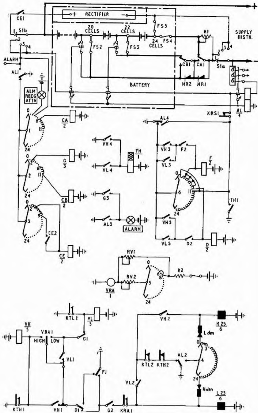
FIG. 1—CONTROL CIRCUIT
