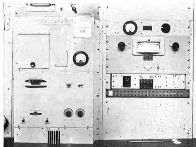
FIG. 2—RYALL-SULLIVAN OSCILLATOR AND TESTER RP 790
