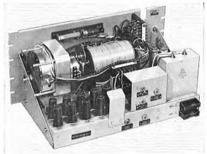
FIG. 5—A COMPARATOR UNIT
