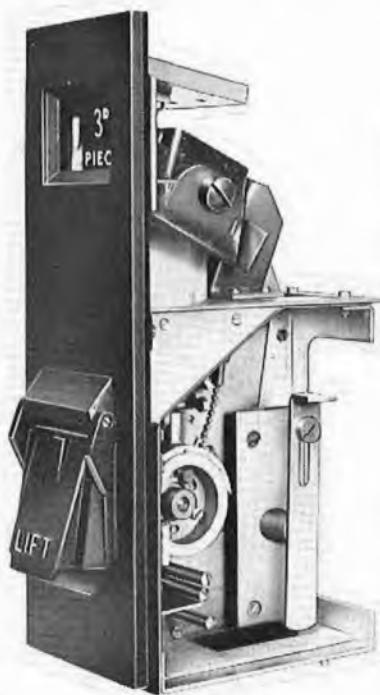
FIG. 1.—3d. STAMP-SELLING MACHINE, TYPE B4
