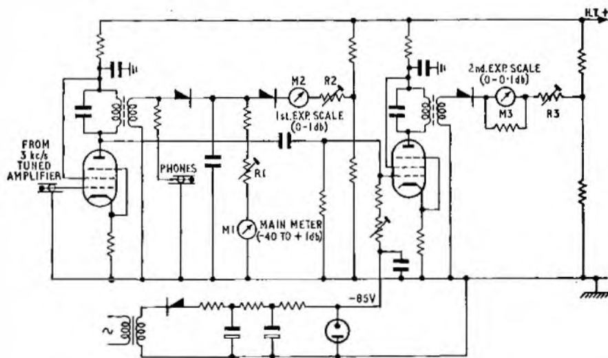
FIG. 3—EXPANDED-SCALE UNIT
