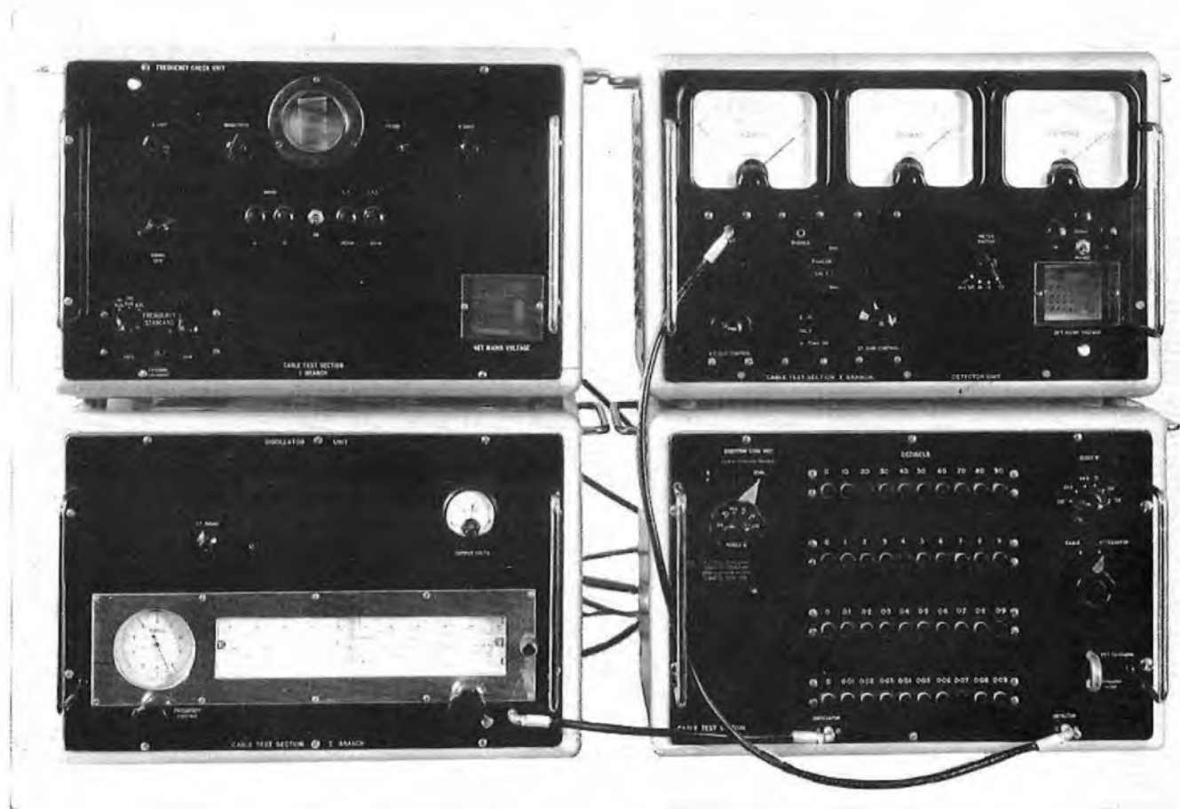
FIG. 2--SELF-TUNING INSERTION-LOSS MEASURING EQUIPMENT
