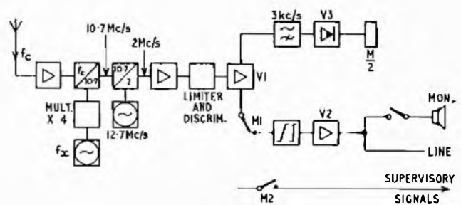
FIG. 4—RADIO RECEIVER
