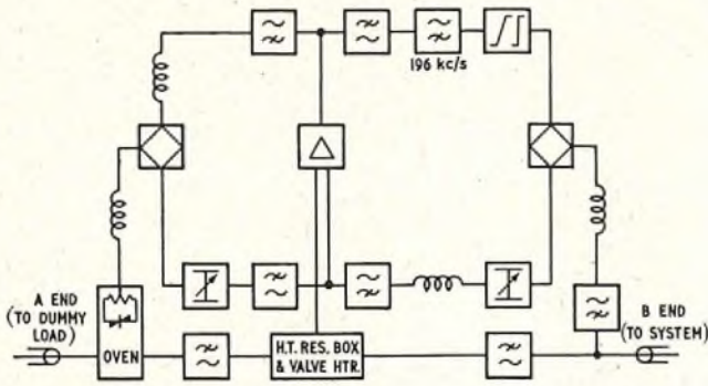
FIG. 6—BLOCK SCHEMATIC DIAGRAM OF TESTING REPEATER AT TERRENCEVILLE
