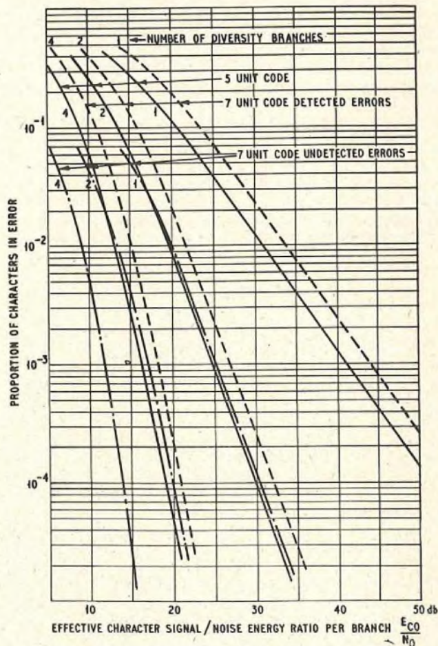
FIG. 5—ERROR LIABILITIES OF 5-UNIT AND 7-UNIT ERROR-DETECTING CODES IN NON-DUAL- AND QUADRUPLE-DIVERSITY RECEPTION OF RAYLEIGH-FADING SIGNALS
