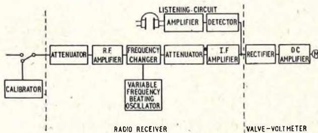
FIG. 16—BLOCK SCHEMATIC DIAGRAM OF TYPICAL INTERFERENCE MEASURING SET
