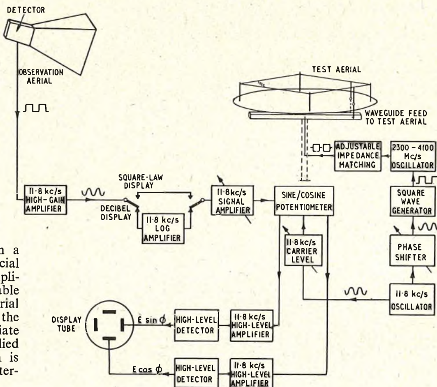
FIG. 3—BLOCK SCHEMATIC DIAGRAM OF THE EQUIPMENT
