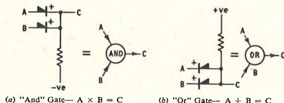
FIG. 7—TYPICAL DIODE GATES
