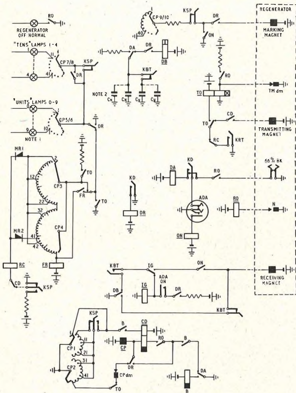
Note 1.—Units lamps multiplied at intervals of ten contacts Note 2.—Capacitors are strapped to give required pulse lengths FIG. 2.—DIALLING-IN AND STORAGE TESTS
