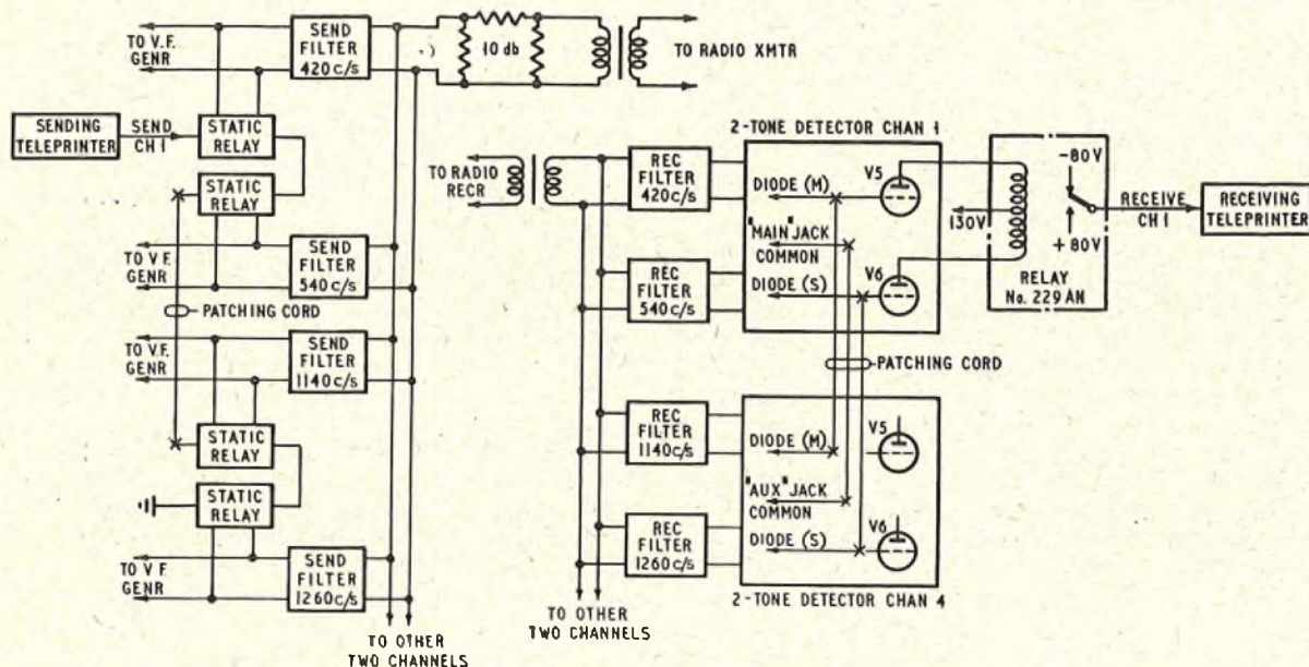
FIG. 2—SCHEMATIC DIAGRAM OF 2/4-TONE DUAL FREQUENCY-DIVERSITY TELEGRAPH SYSTEM
