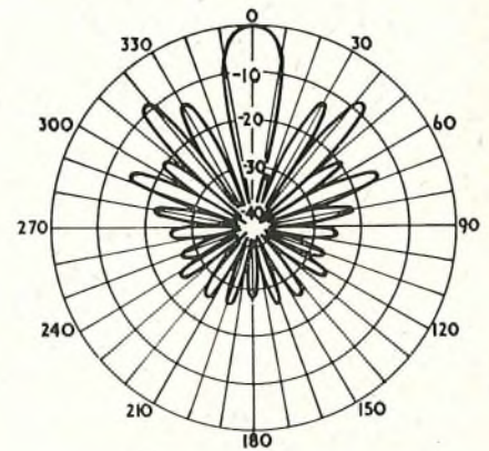
FIG. 7.—CALCULATED DIRECTIVITY CHARACTERISTIC OF RHOMBIC AERIAL
