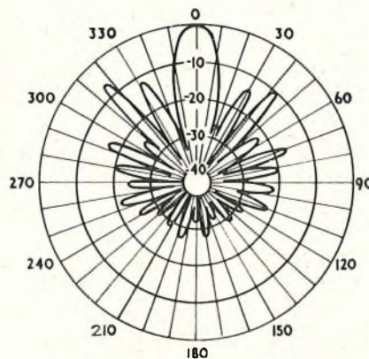
FIG. 6.—MEASURED DIRECTIVITY CHARACTERISTIC OF FULL-SCALE RHOMBIC AERIAL
