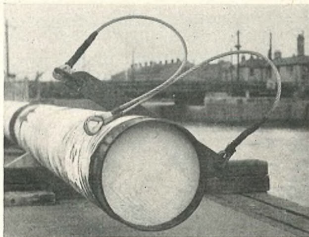
FIG. 9—END OF MAIN-CROSSING PIPE, SHOWING SLING AND WOODEN DISK
