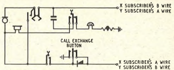
FIG. 9—SHARED-SERVICE TELEPHONE CIRCUIT
