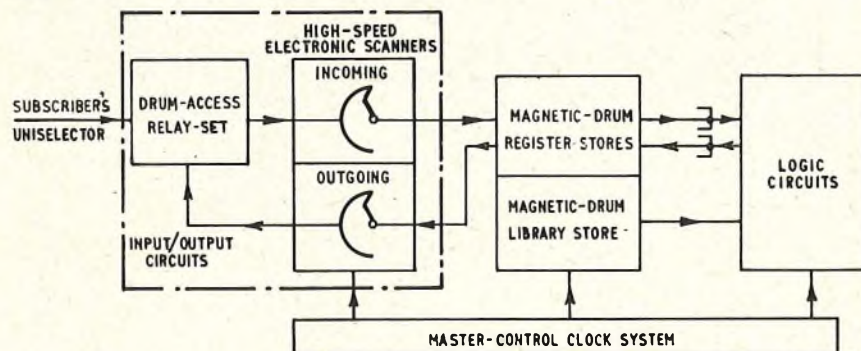
FIG. 1—BLOCK SCHEMATIC DIAGRAM OF REGISTER-TRANSLATOR
