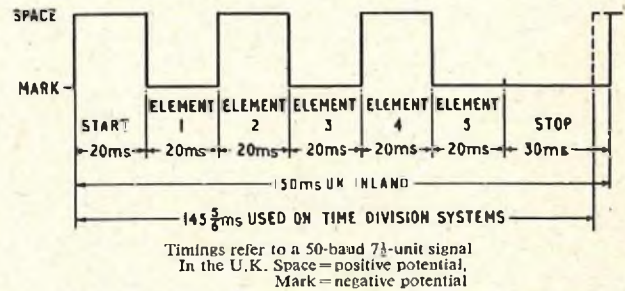
FIG. 1.—EXAMPLE OF 5-UNIT CODE:—LETTER Y (MSMSM)
