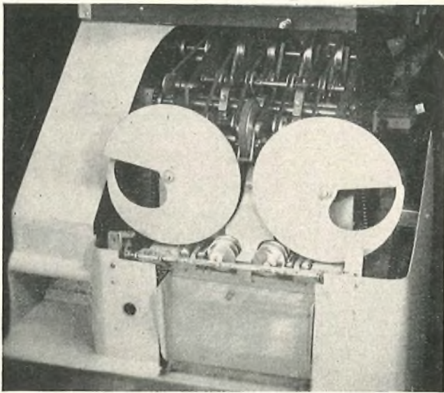
The four helices, two large and two small, can be seen at the front. FIG. 3—LETTER-PRESENTATION SECTION WITH COVER REMOVED
