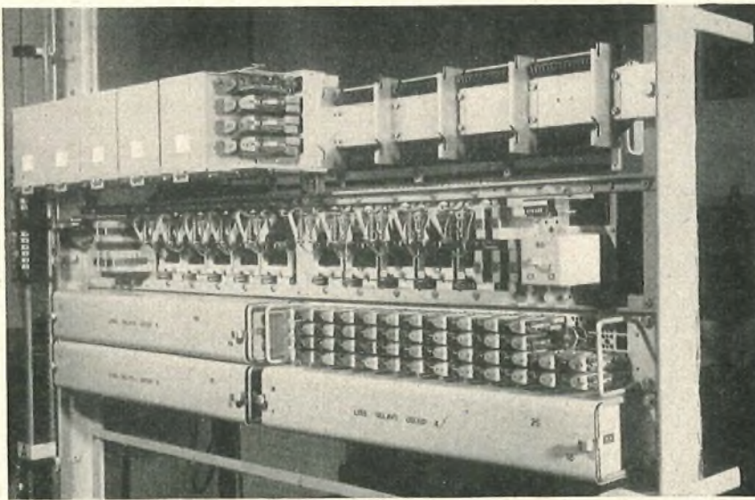
FIG. 12—FRONT VIEW OF SHELF UNIT.
