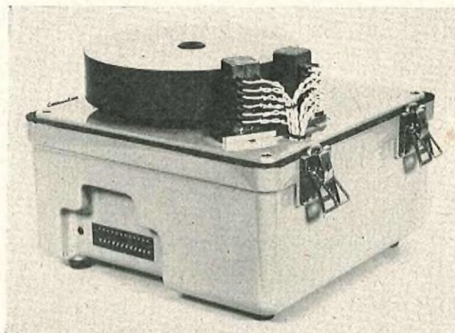
FIG. 2—MAGNETIC DRUM
