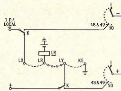
FIG. 10—T.O.S. ARRANGEMENTS FOR SHARED-SERVICE LINES
