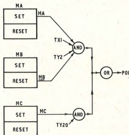
(a) MA \times \overline{MB} \times TX1 \times TY2 + MC \times TY20 = POI
