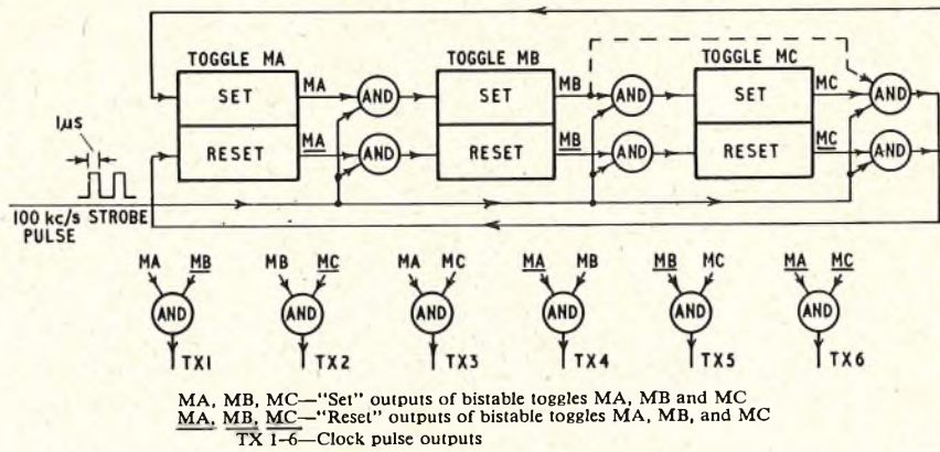
FIG. 5—FUNCTIONAL DIAGRAM OF TX CLOCK RING COUNTER
