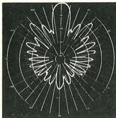
Photographed from face of cathode-ray tube FIG. 5.—MEASURED DIRECTIVITY CHARACTERISTIC OF MODEL RHOMBIC AERIAL
