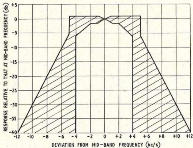
The overall response curve of the measuring set should be within the shaded area. FIG. 17—TYPICAL LIMITS OF OVERALL FREQUENCY CHARACTERISTIC
