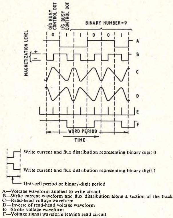
FIG. 3—PHASE MODULATION RECORDING WAVEFORMS
