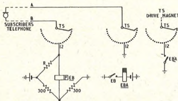
FIG. 7—LOOP-RESISTANCE TEST
