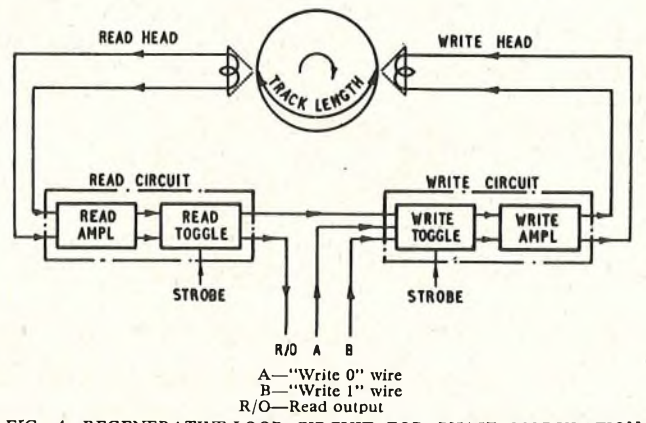
FIG. 4—REGENERATIVE-LOOP CIRCUIT FOR PHASE MODULATION RECORDING
