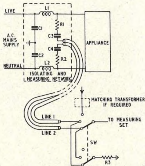
Up to 30 Mc/s: R1 = R2 = 75 ohms; R3 = 150 ohms Above 30 Mc/s: R1 = R2 = 0 ohms; R3 = 75 ohms FIG. 18—ARRANGEMENT FOR MAINS-VOLTAGE AND FIELD-STRENGTH MEASUREMENTS
