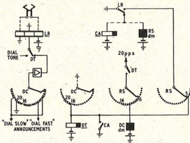
FIG. 8—DIAL-SPEED TEST
