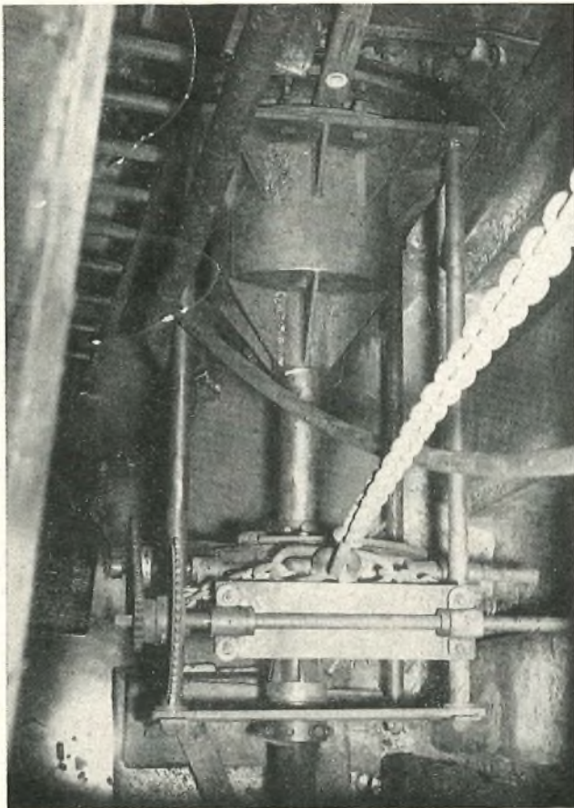
FIG. 6—MACHINE USED TO TREPAN THE HARBOUR-WALL PILING
