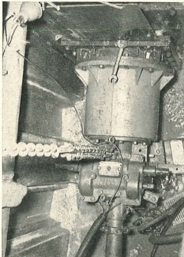
FIG. 3—TREPPANNING MACHINE
