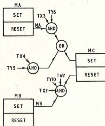
(b) MA \times TX3 \times TY6 + TX4 \times TY5 = MC \overline{MB} \times TX2 \times TY10 \times TW2 = MC
