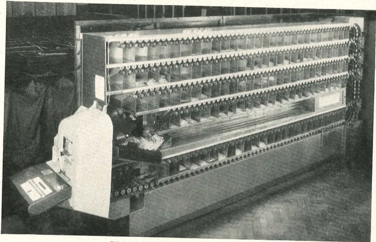
FIG. 1—THE EXPERIMENTAL LETTER-SORTING MACHINE
