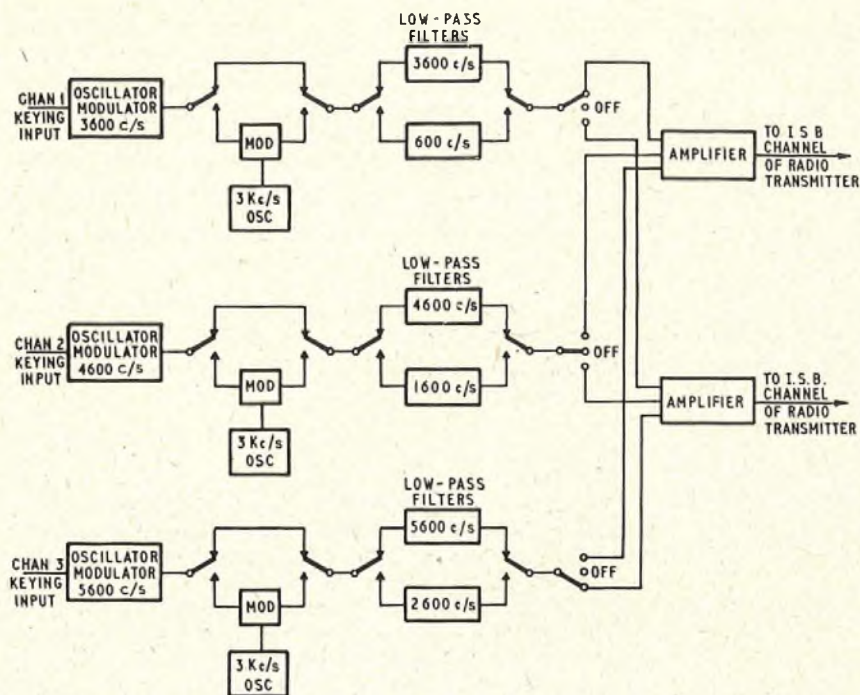
FIG. 3—THREE-CHANNEL TELEGRAPH MODULATOR (W.H.A.55) FOR I.S.B. RADIO TRANSMITTERS
