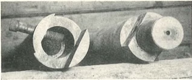
FIG. 5—JOINT USED IN CUTTER DRIVE SHAFT TO MAINTAIN THE CYLINDRICAL PROFILE OF THE SHAFT
