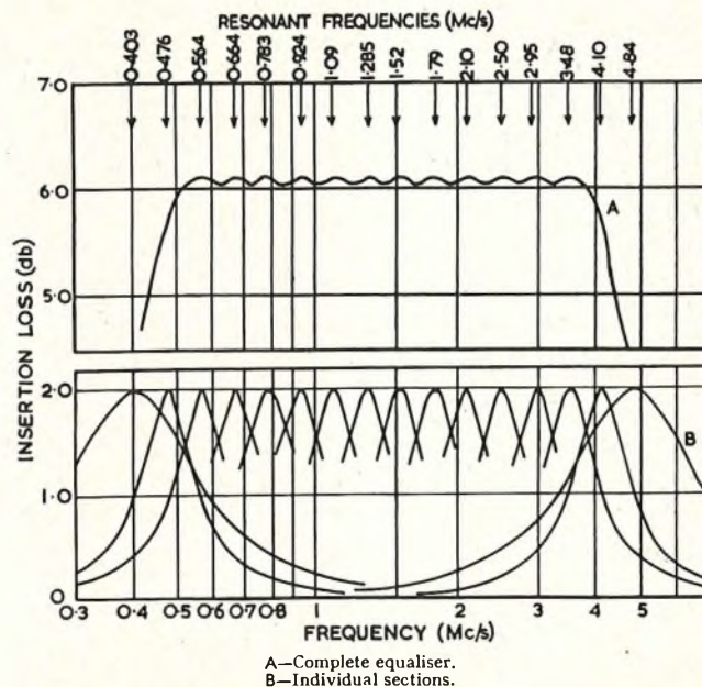
FIG. 13.—INSERTION LOSS OF 0.5-4 Mc/s LINE RESIDUAL EQUALISER, WITH ALL SECTIONS SET AT 2-DB. PAD LOSS.
