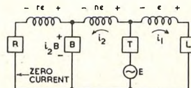
FIG. 2.—THE BASIC CIRCUIT SENDING TO LINE.
