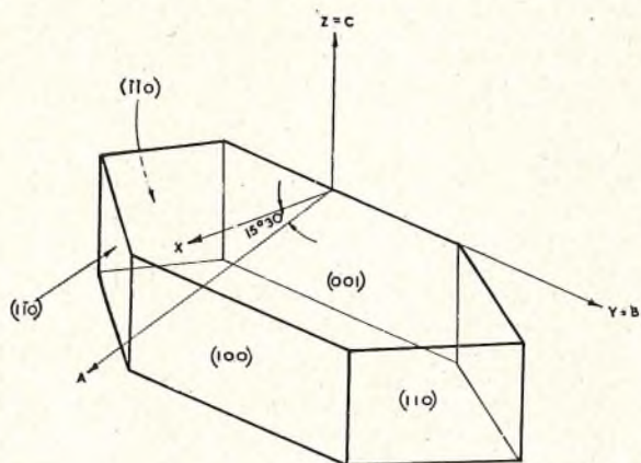
X, Y, Z, ARE RECTANGULAR CO-ORDINATES. A, B, C, ARE CRYSTAL AXES.
