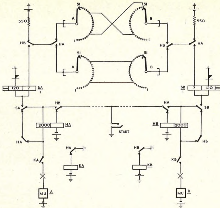
FIG. 4.—TEST CIRCUIT FOR MOTOR-DRIVEN UNISELECTORS.
