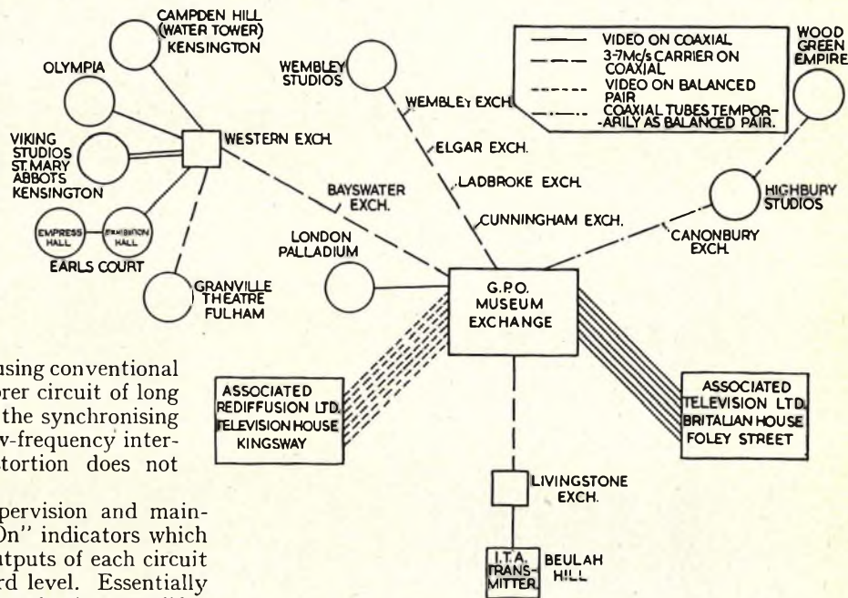
FIG. 6.—THE LONDON NETWORK.
