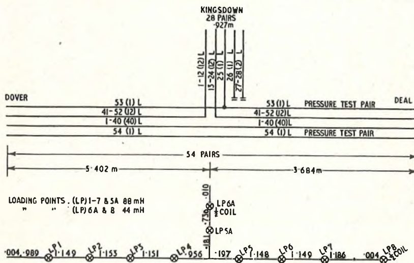
FIG. 1.—DIAGRAM OF THE DOVER-DEAL EXPERIMENTAL CABLE.
