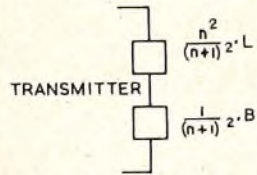
FIG. 3.—IMPEDANCE TO WHICH TRANSMITTER IS CONNECTED.
