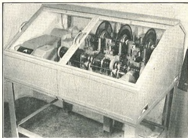
FIG. 10.—ANNOUNCING MACHINE.
