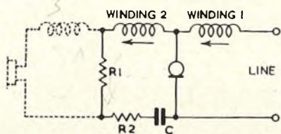
FIG. 13.—SENDING CIRCUIT OF TELEPHONE NO. 332.
