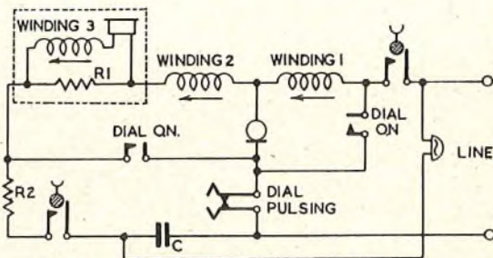
FIG. 11.—REARRANGED CIRCUIT OF TELEPHONE NO. 332.
