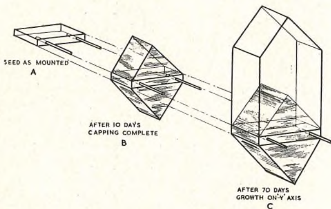
FIG. 7.—GROWTH OF EDT CRYSTAL.
