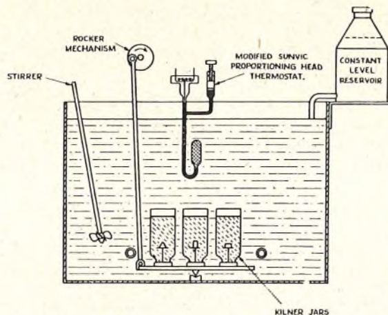
FIG. 4.—HOT-WATER BATH.
