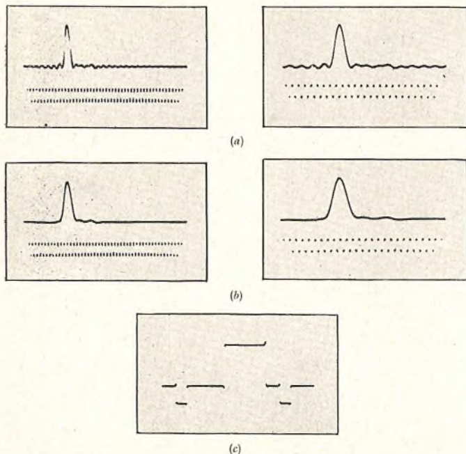
(a) Sine-squared Pulse, 0.17-microsecond duration at half-amplitude. (b) Sine-squared Pulse, 0.33-microsecond duration at half-amplitude. (c) 40-microsecond Bar, 0.33-microsecond rise-time. (a) and (b) Timing Wave: 6 Mc/s.
